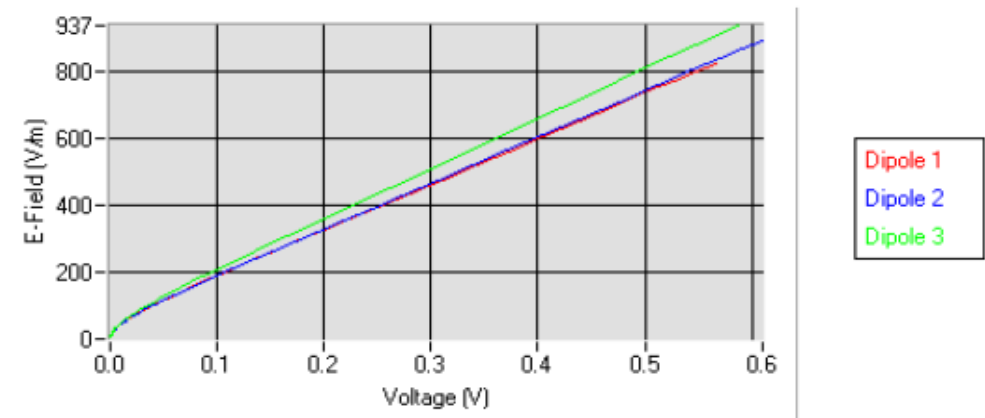
Calibration curves
