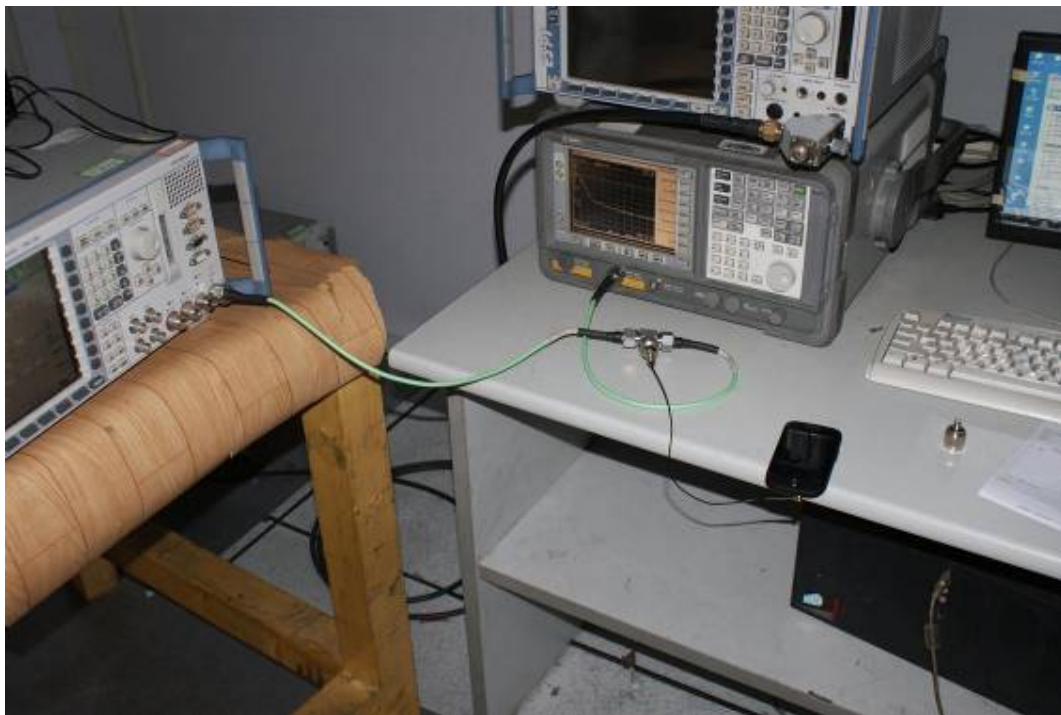
CONDUCTED TEST SETUP
