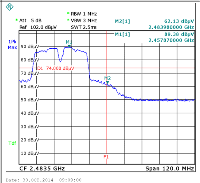
N40-9 Band Edge, Right Side (Peak) - 802.11n40
