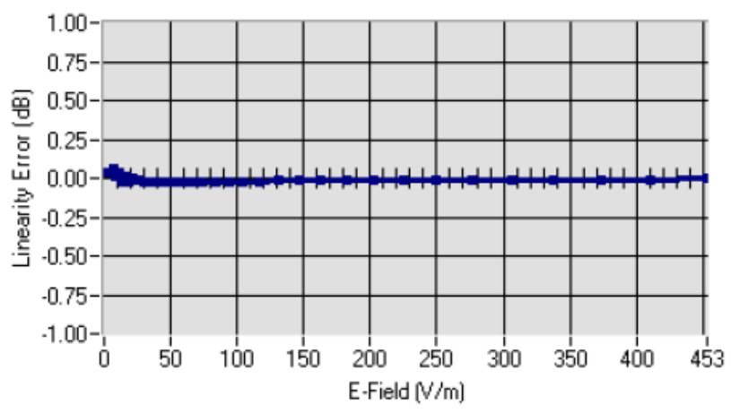
Linearity
