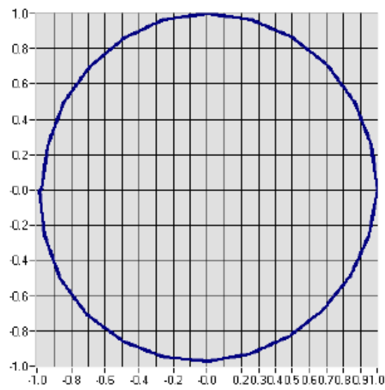
Isotropy curve
