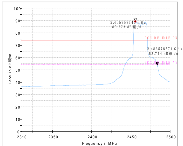
Fig.49 Radiated emission (Power): 802.11g, high channel
