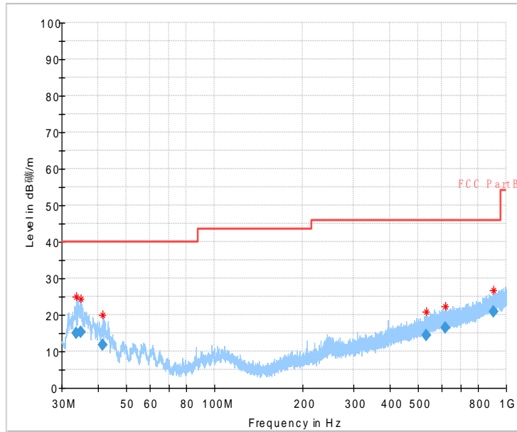
Fig.50 Radiated Spurious Emission (802.11g,Ch6,30MHz~1GHz)
