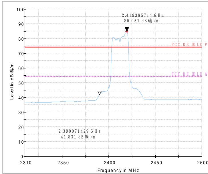
Fig.53 Radiated emission (Power): 802.11n, low channel
