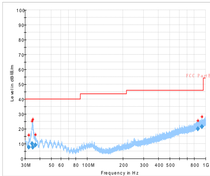
Fig.45 Radiated Spurious Emission (802.11b,Ch6,30MHz~1GHz)
