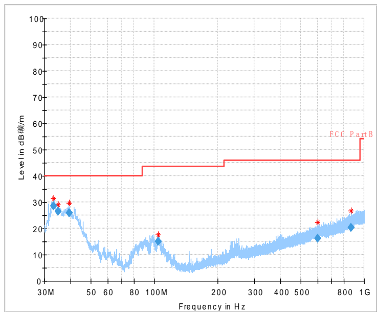
Fig.55 Radiated Spurious Emission (802.11 n-20MHz,Ch6,30MHz~1GHz)
