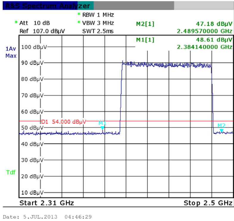
8DPSK hopping-PK
