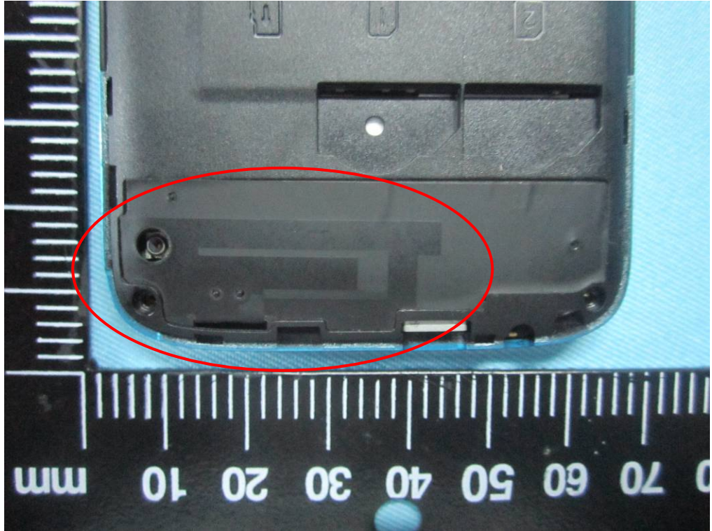
GSM/PCS/UMTS-FDD Antenna
