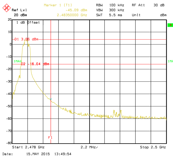
No-hopping mode
