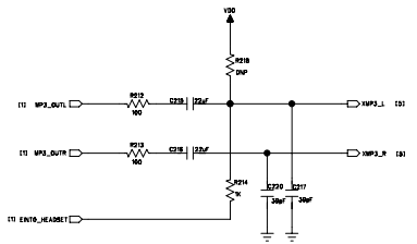
Headset spk
