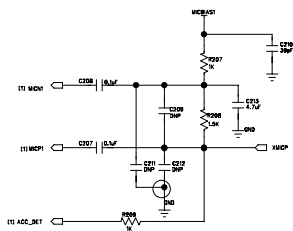
Headset MIC
