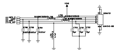
IO connector
