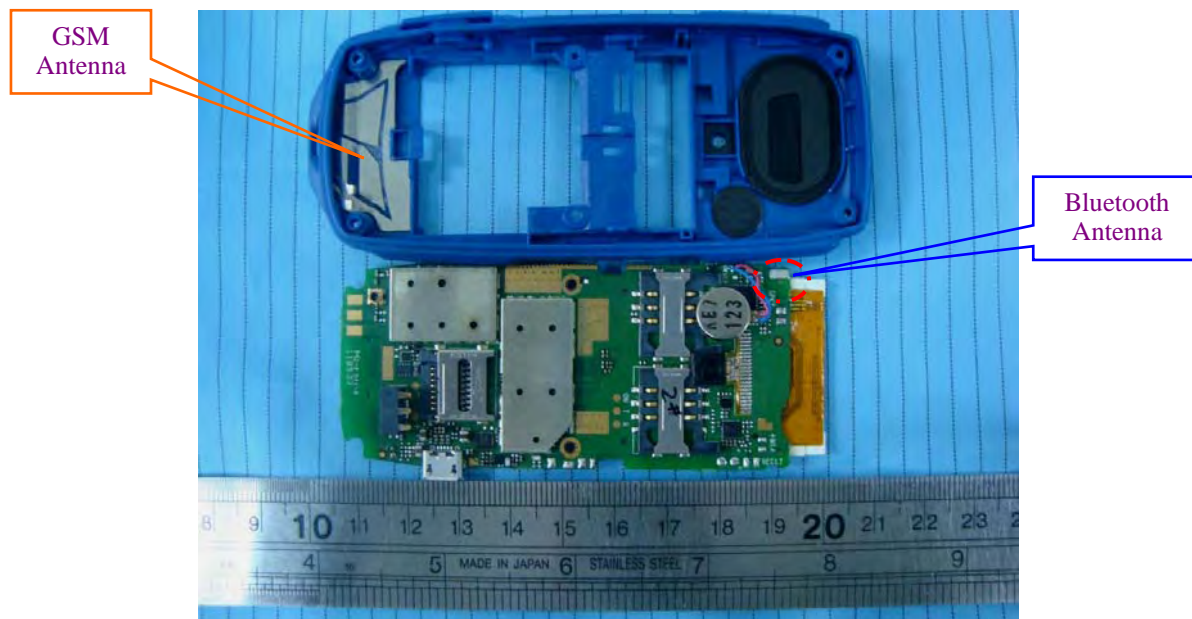
Antenna Location
