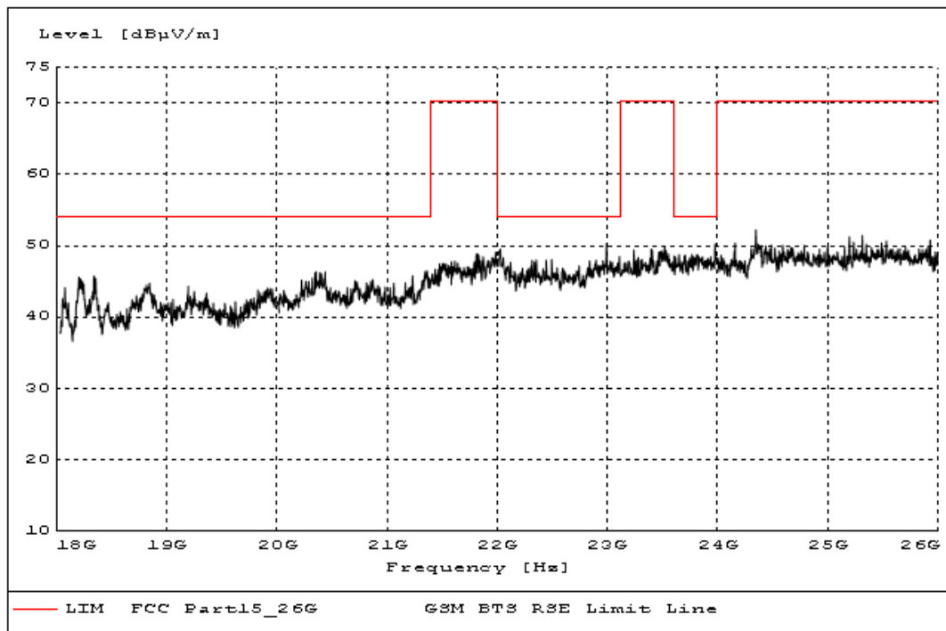
Fig. 24 Radiated emission: 18 GHz ~ 26 GHz
