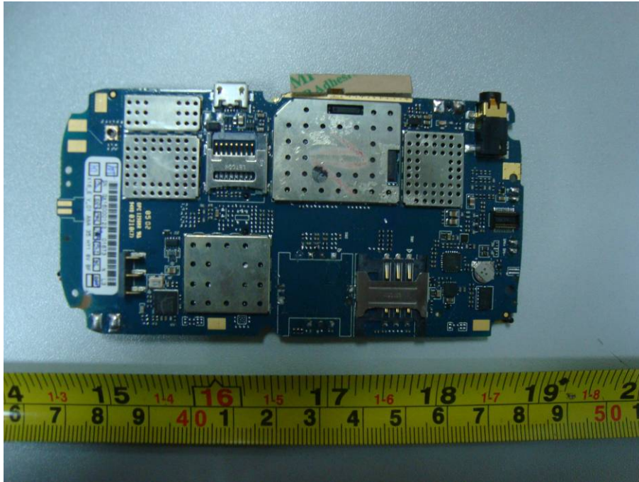
EUT – Main Board without Antenna view
