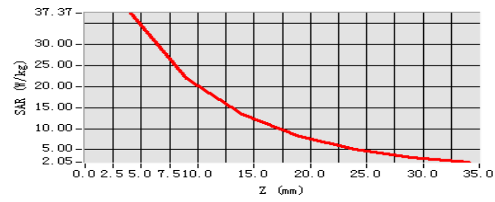
SAR, Z Axis Scan (X = 0, Y = -1)
