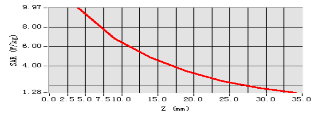
SAR, Z Axis Scan (X = 0, Y = -2)
