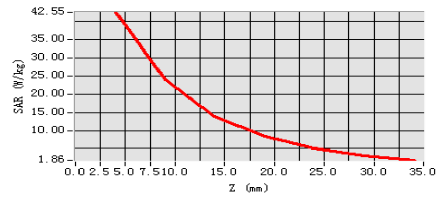
SAR, Z Axis Scan (X = 0, Y = 0)
