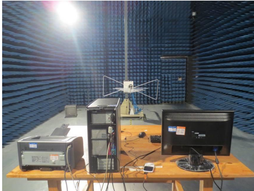
Radiated Emission
