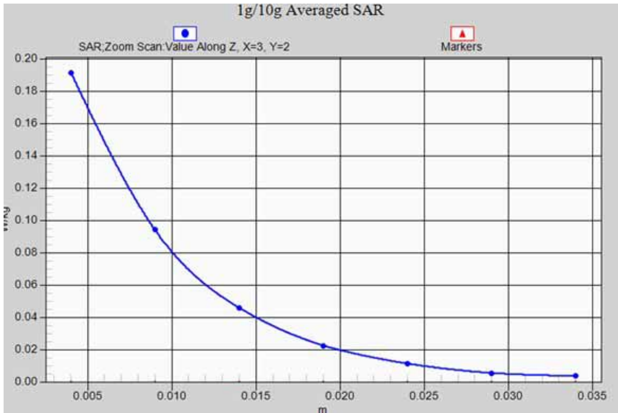
WIFI-802.11b RIGHT/CHEEK-High_ z-axis scan
