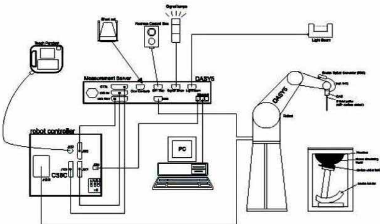
Figure1 system diagram
