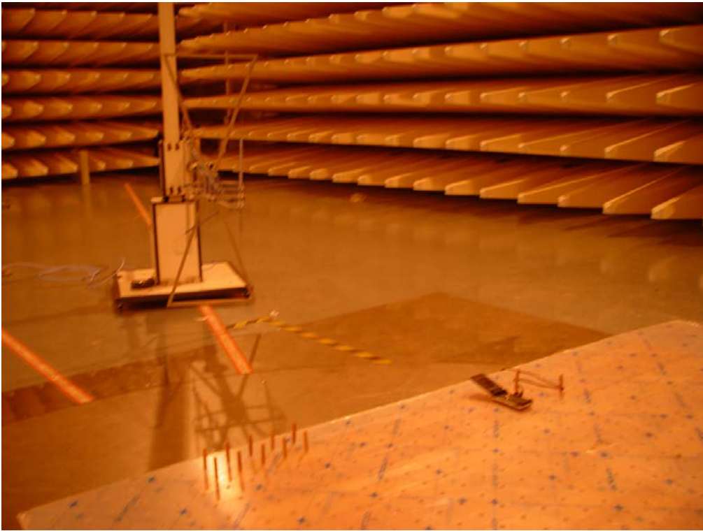
Pic 3 Radiated Emissions Test Setup
