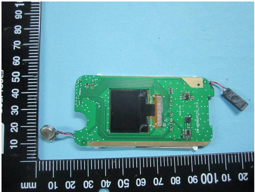
LCD board - Rear View
