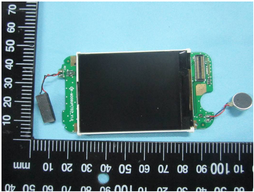
LCD board - Front View
