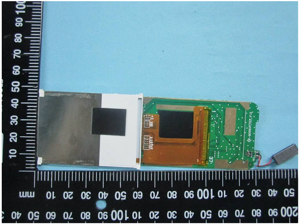
LCD board Cover off - Front View
