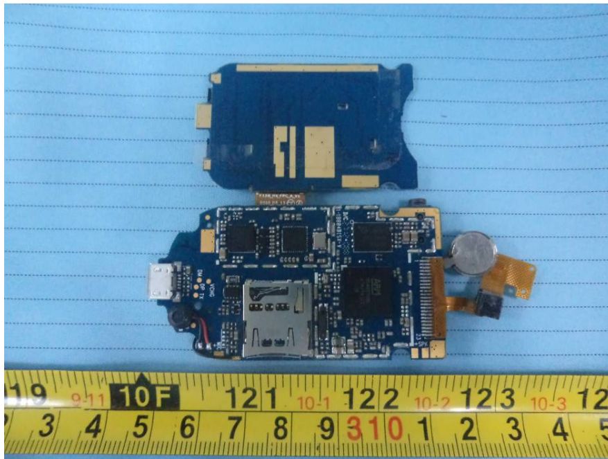
EUT – Main Board and Key Board Top View
