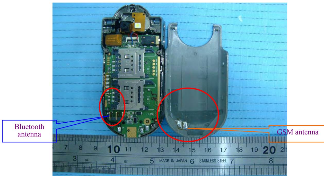
BT and GSM Antenna Location
