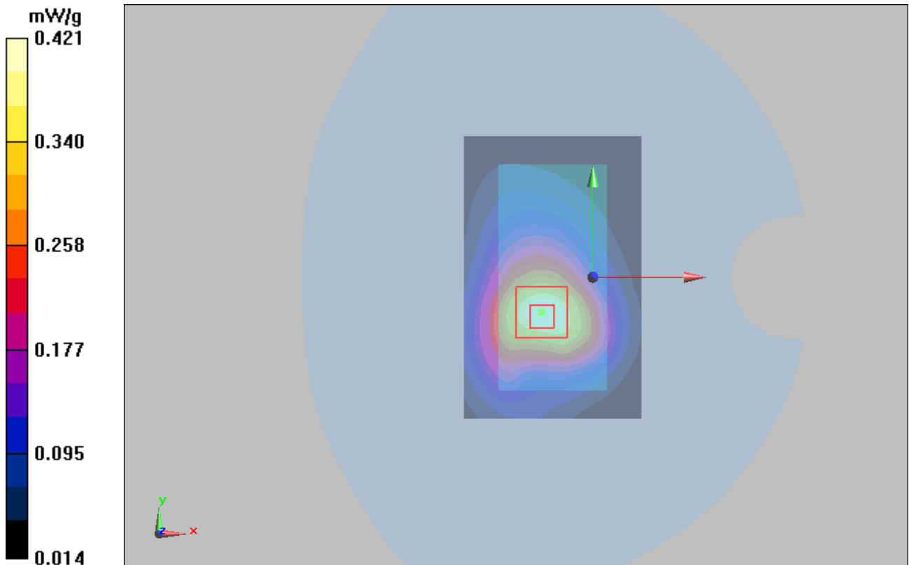
Figure 32 Body, Towards Ground, GSM 1900 Channel 661 Close
