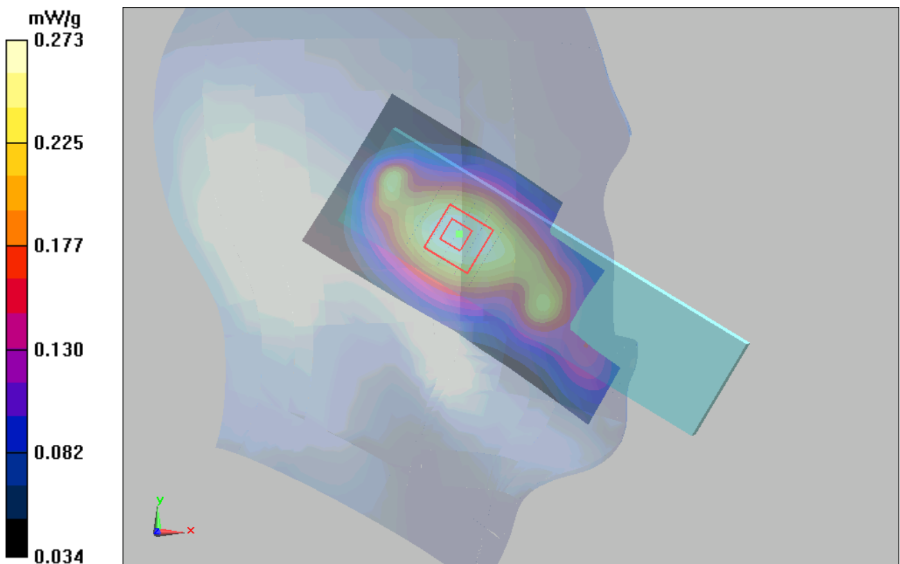
Figure 11 Left Hand Touch Cheek GSM 850 Channel 251 Open
