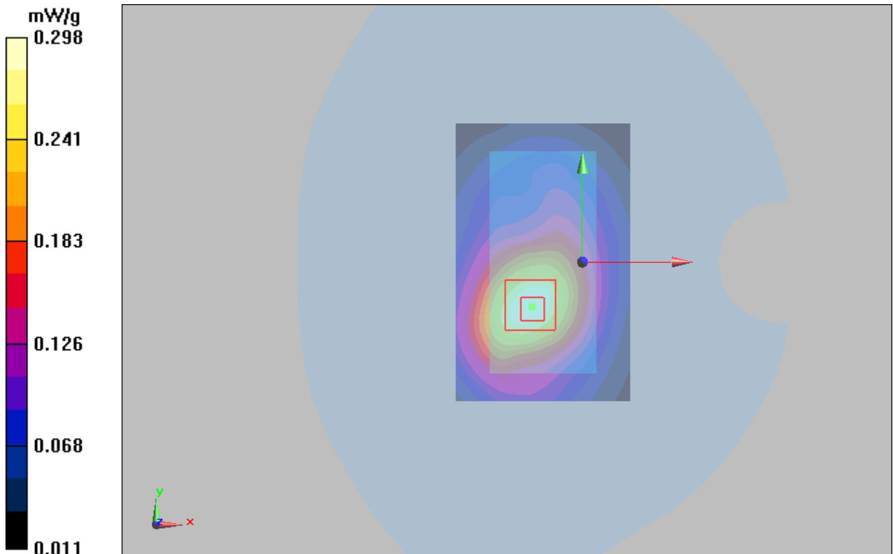
Figure 38 Body, Towards Phantom, GSM 1900 GPRS (4TXslots) Channel 661 Close
