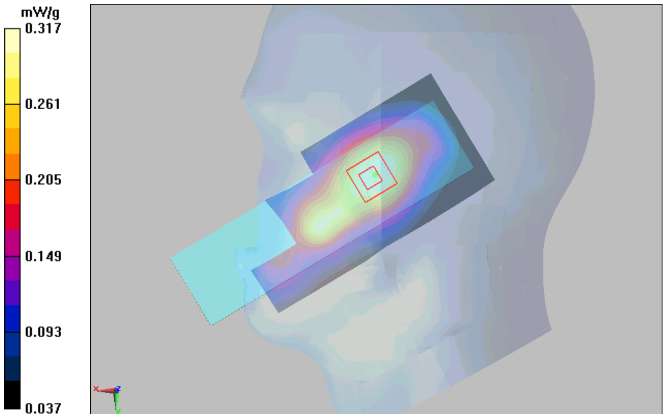
Figure 15 Right Hand Touch Cheek GSM 850 Channel 190 Open
