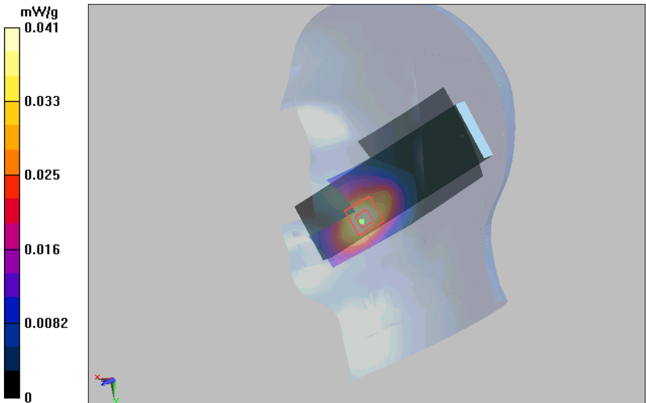
Figure 31 Right Hand Tilt 15° GSM 1900 Channel 661 Open
