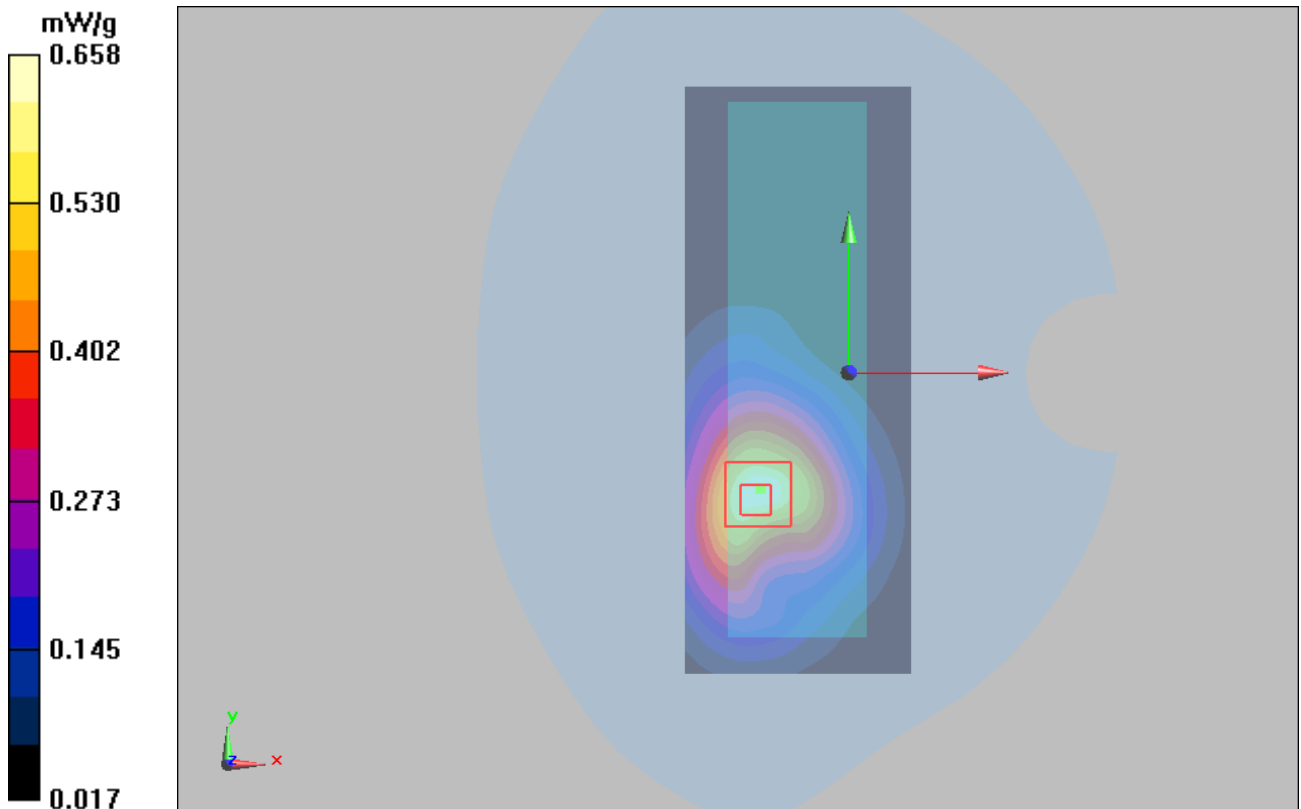
Figure 39 Body, Towards Ground, GSM 1900 GPRS (4TXslots) Channel 661 Open
