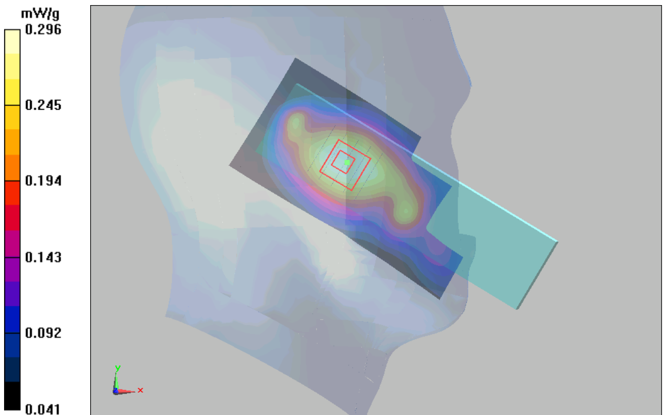
Figure 13 Left Hand Touch Cheek GSM 850 Channel 128 Open
