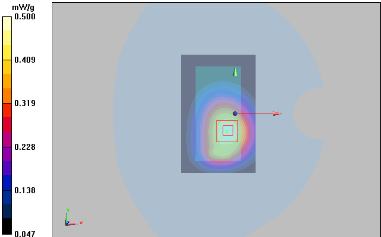
Figure 18 Body, Towards Ground, GSM 850 GPRS (2TXslots) Channel 190 Close
