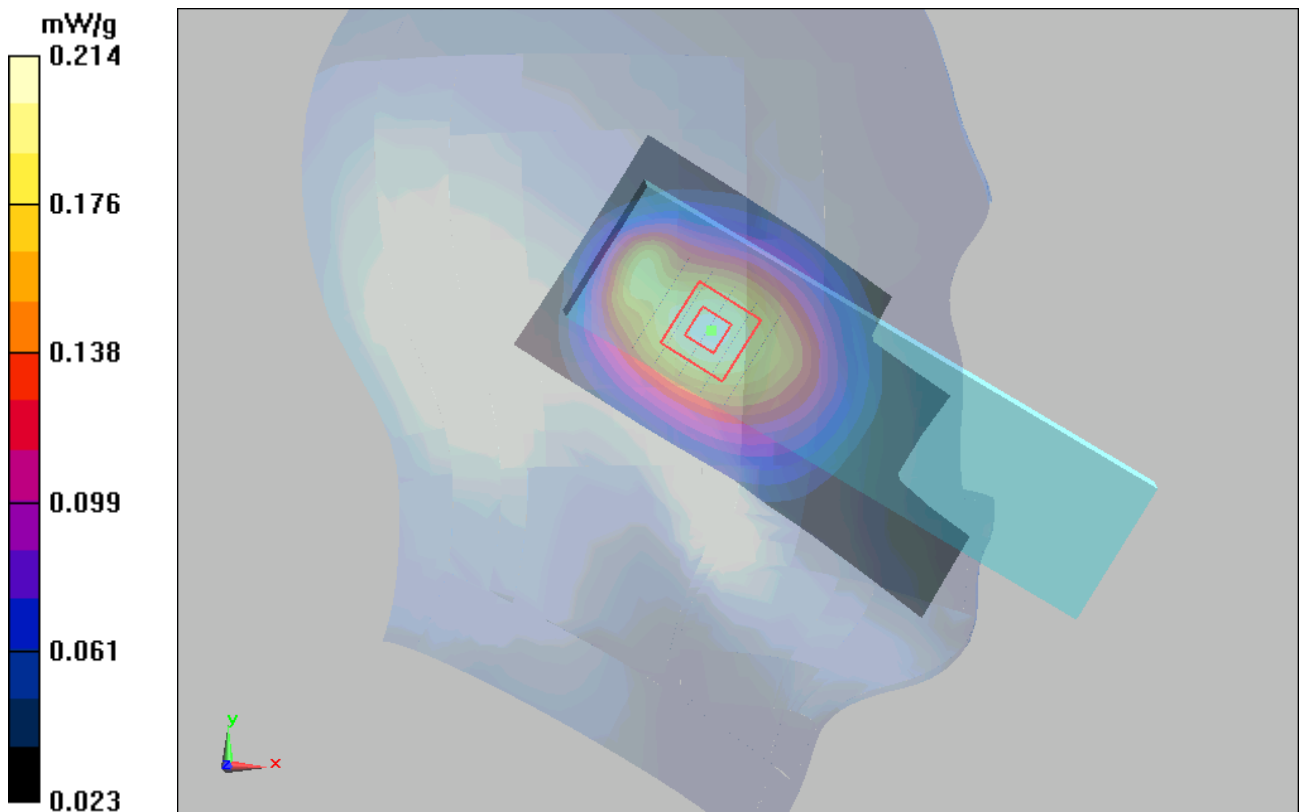
Figure 14 Left Hand Tilt 15° GSM 850 Channel 190 Open
