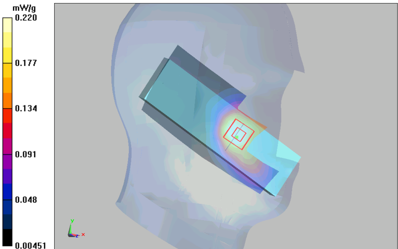
Figure 26 Left Hand Touch Cheek GSM 1900 Channel 661 Open
