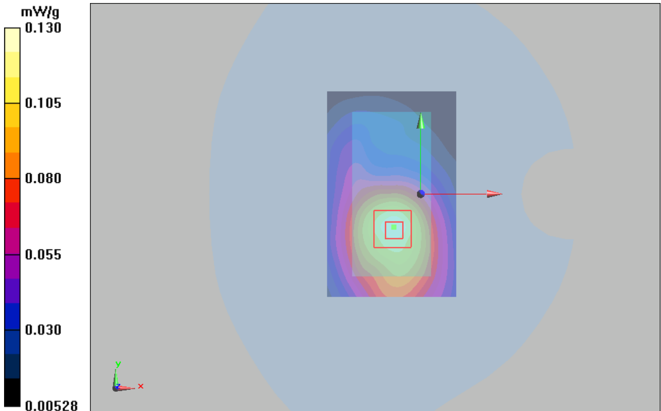
Figure 40 Body with Earphone, Towards Ground, GSM 1900 Channel 512 Close
