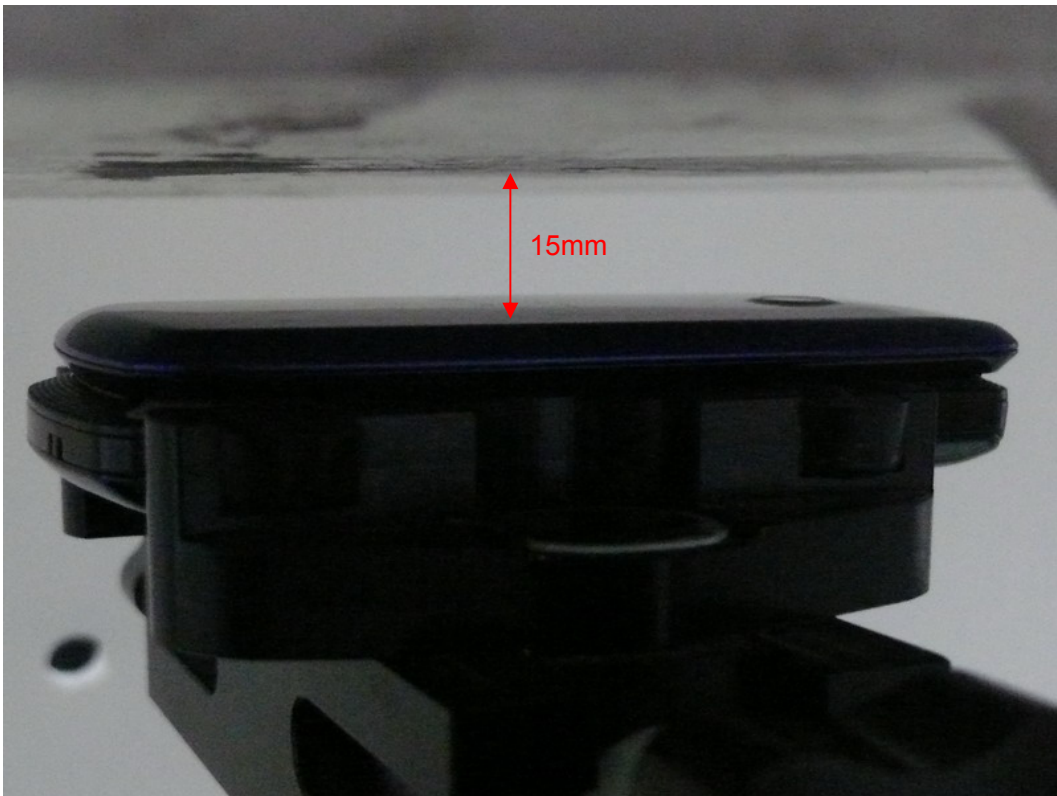
Picture 12: Body, The EUT display towards phantom, the distance from handset to the bottom of the Phantom is 15mm (Close)
