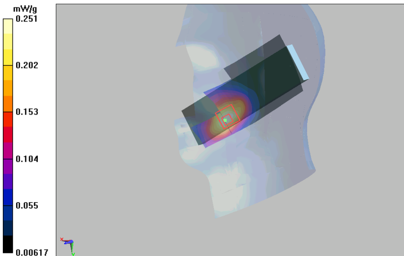
Figure 29 Right Hand Touch Cheek GSM 1900 Channel 661 Open
