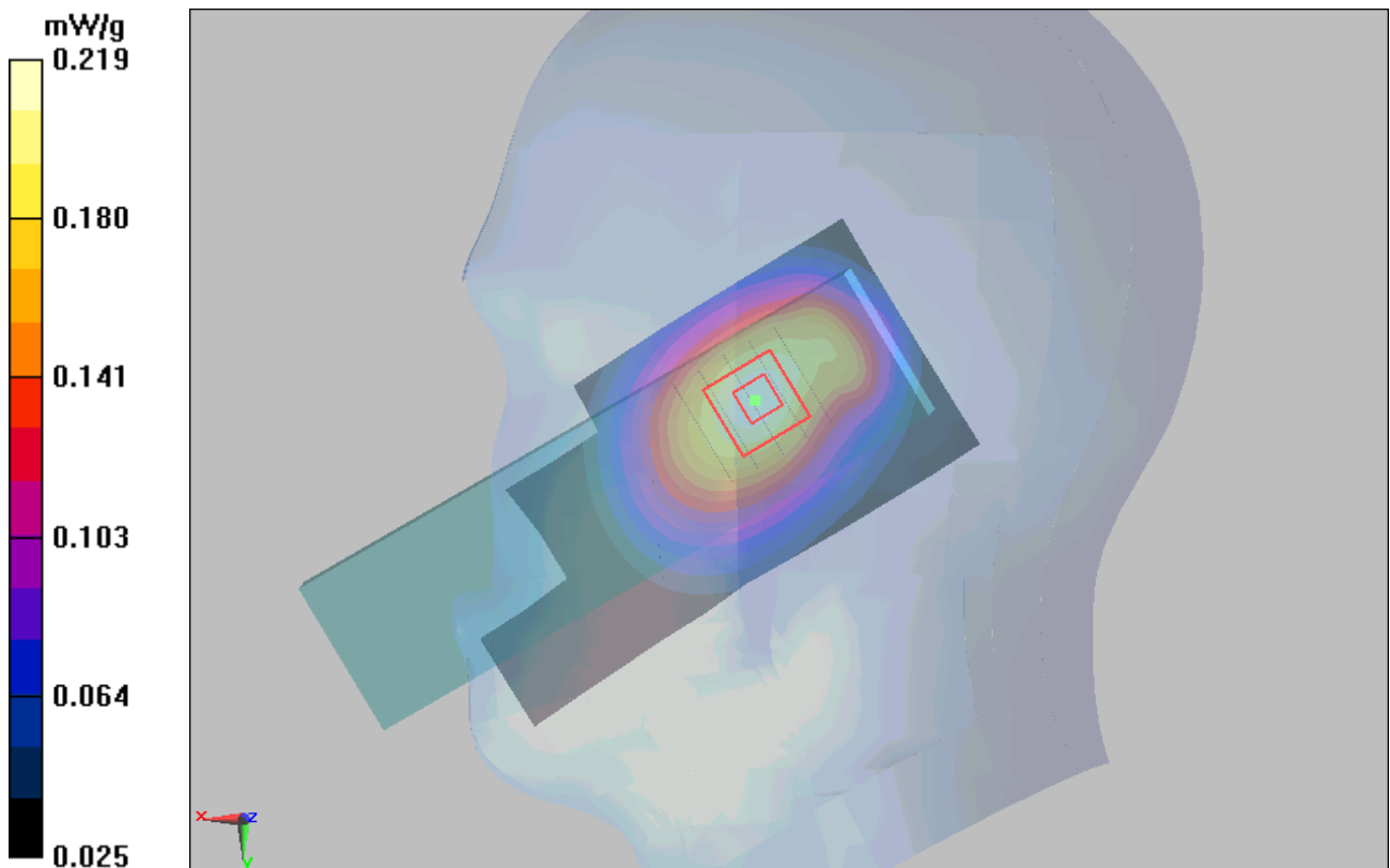
Figure 16 Right Hand Tilt 15° GSM 850 Channel 190 Open
