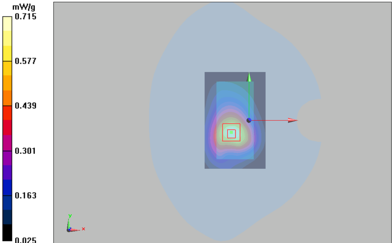
Figure 36 Body, Towards Ground, GSM 1900 GPRS (4TXslots) Channel 661 Close
