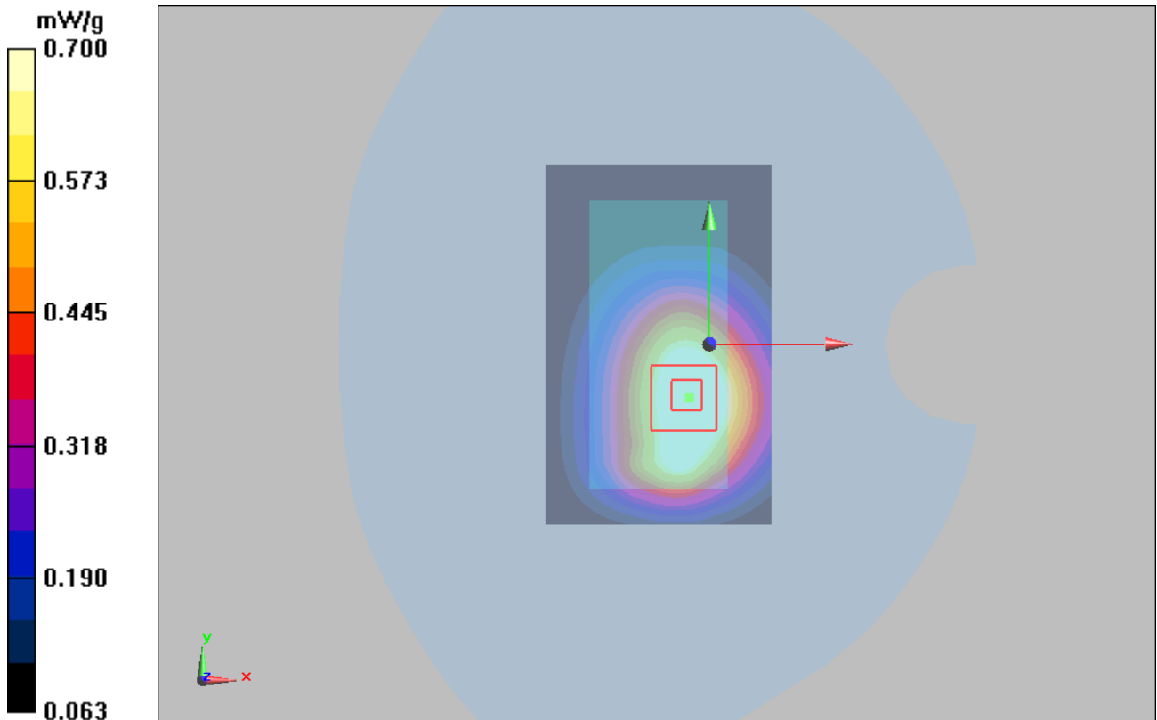
Figure 19 Body, Towards Ground, GSM 850 GPRS (3TXslots) Channel 190 Close
