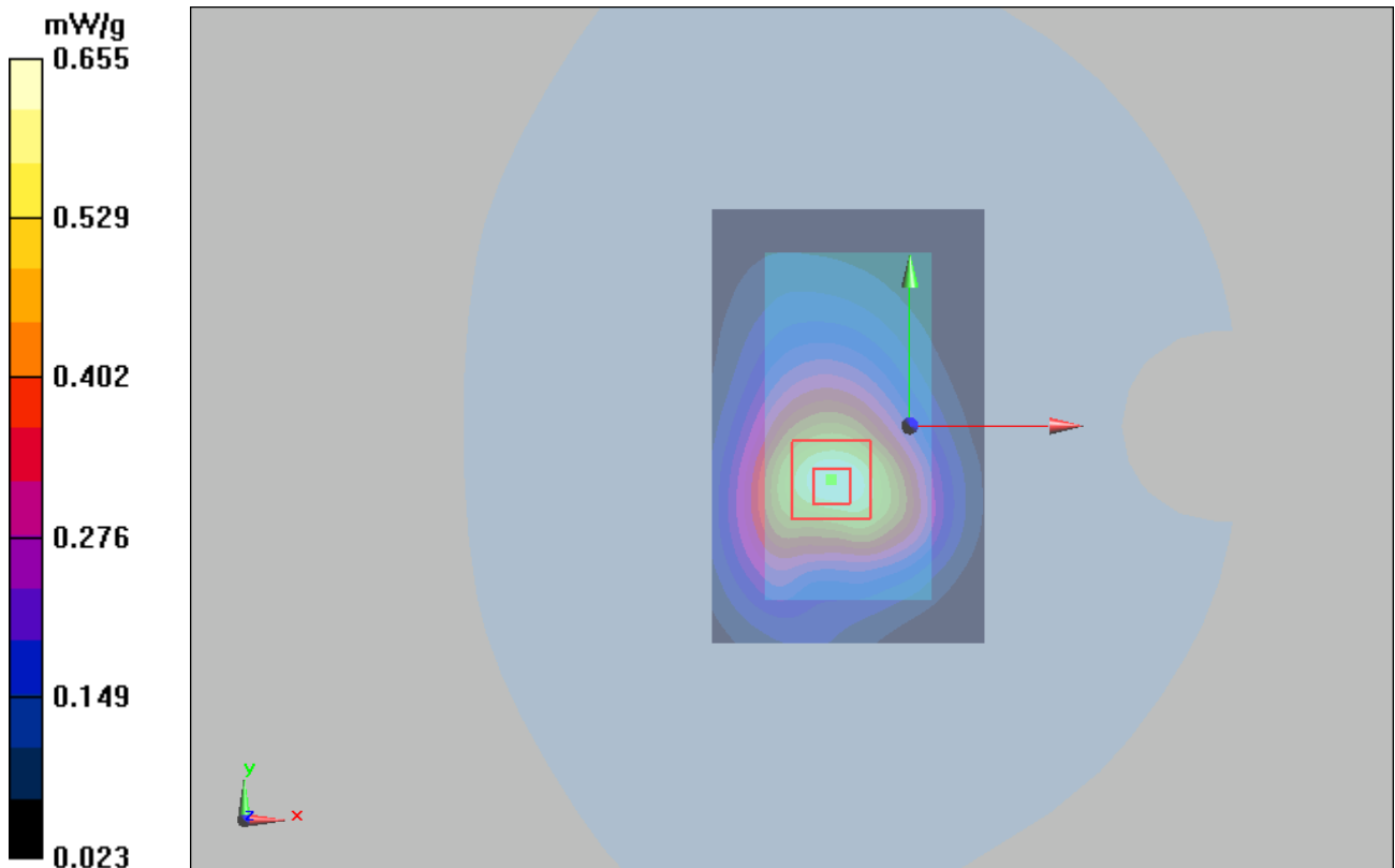
Figure 34 Body, Towards Ground, GSM 1900 GPRS (3TXslots) Channel 661 Close
