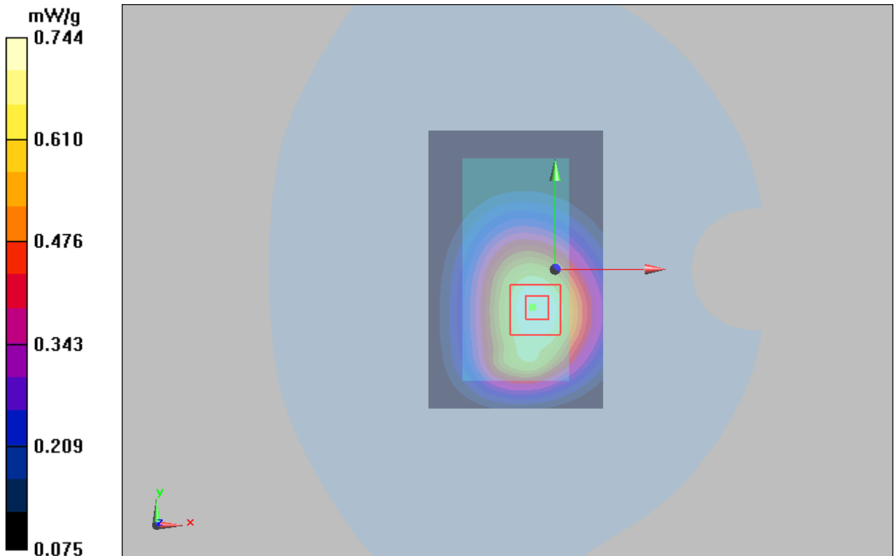
Figure 20 Body, Towards Ground, GSM 850 GPRS (4TXslots) Channel 251 Close
