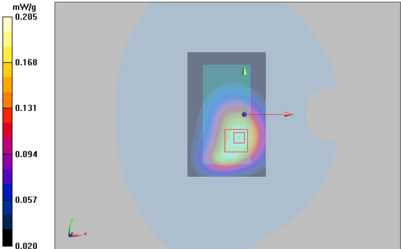
Figure 25 Body with Earphone, Towards Ground, GSM 850 Channel 190 Close
