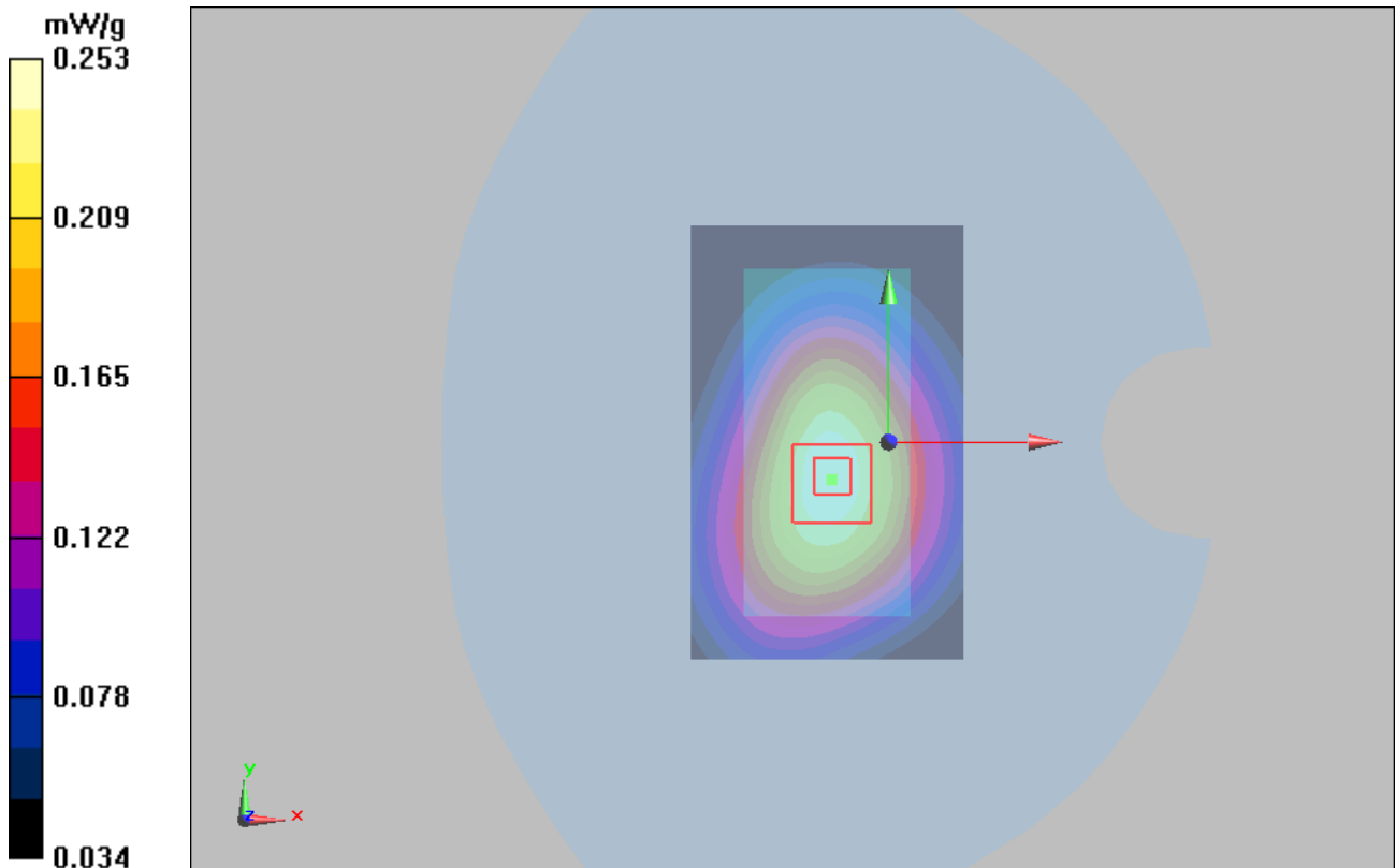
Figure 23 Body, Towards Phantom, GSM 850 GPRS (4TXslots) Channel 190 Close
