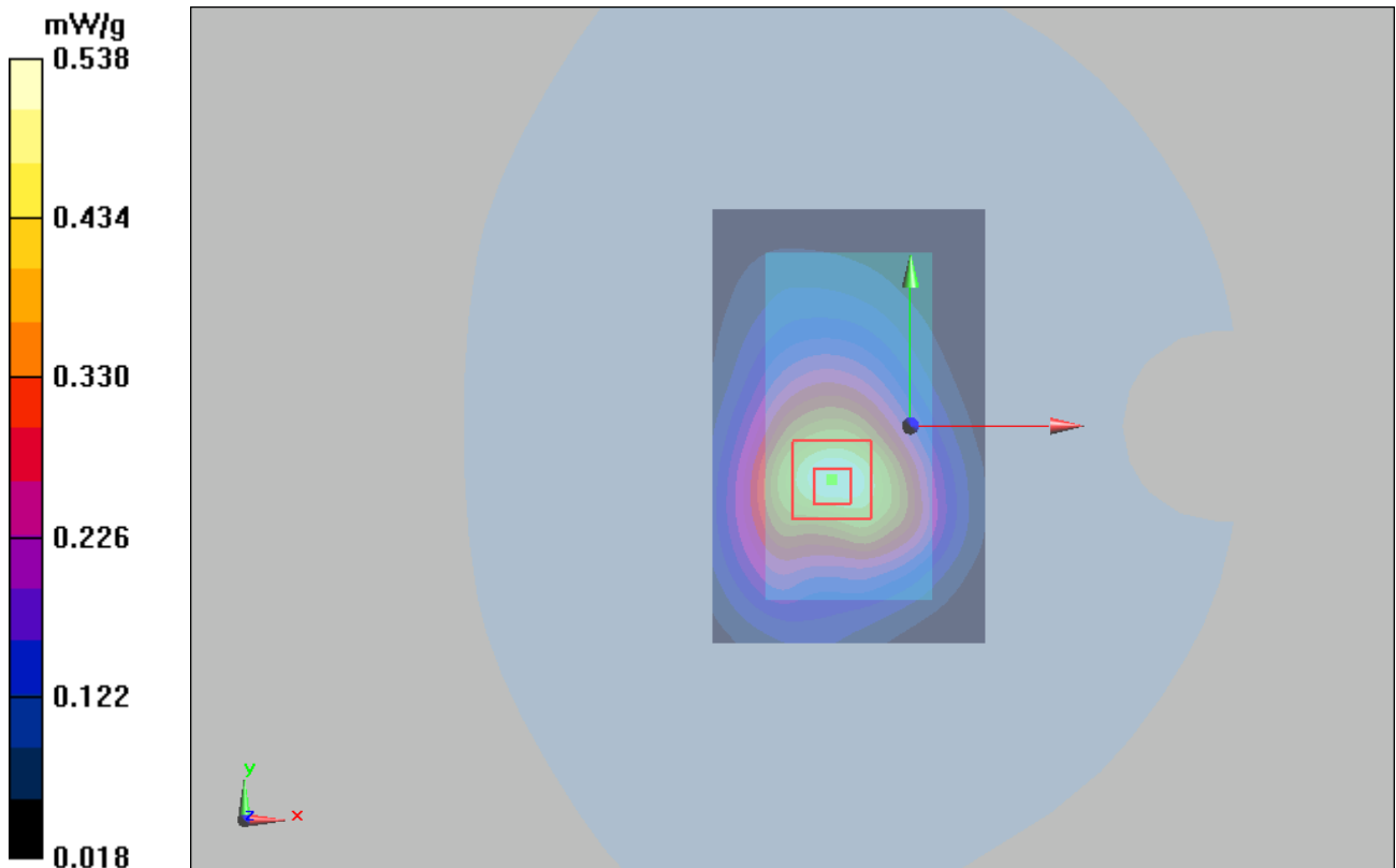
Figure 35 Body, Towards Ground, GSM 1900 GPRS (4TXslots) Channel 810 Close
