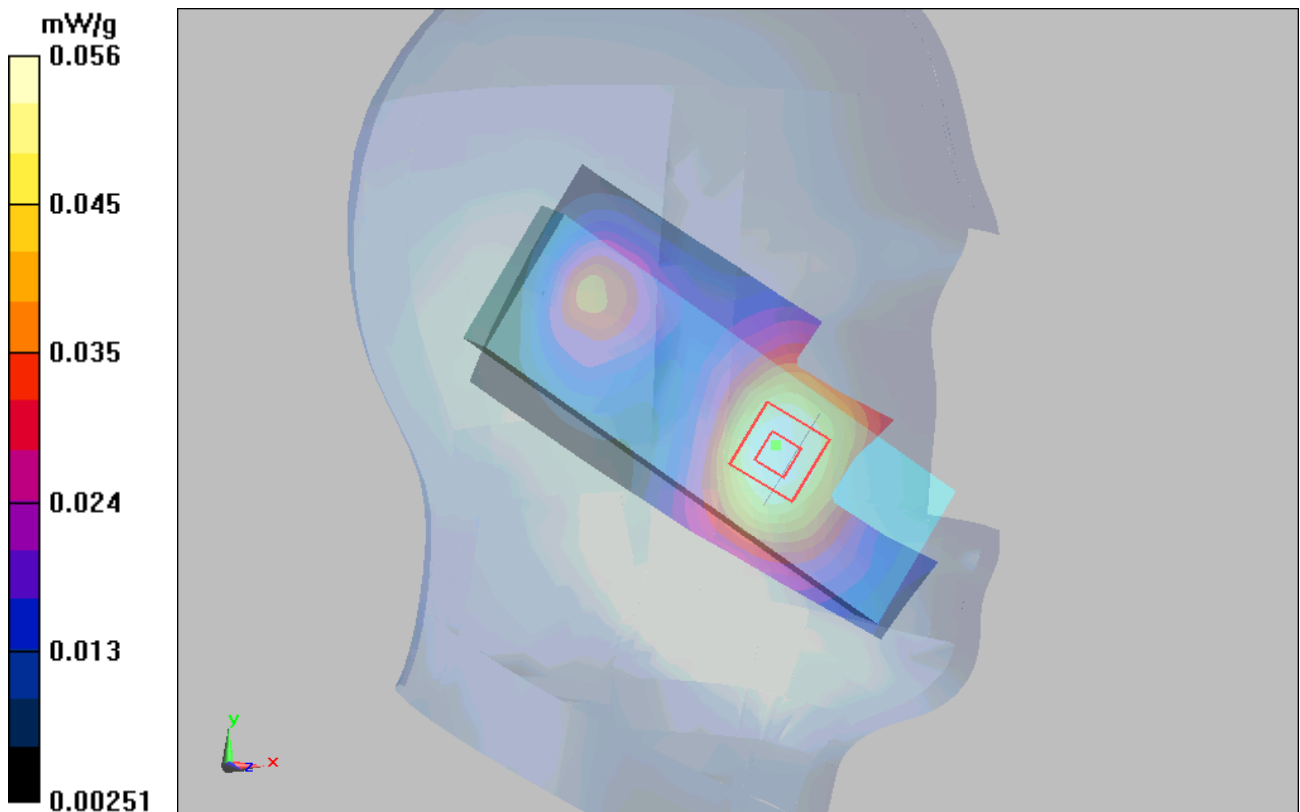
Figure 27 Left Hand Tilt 15° GSM 1900 Channel 661 Open
