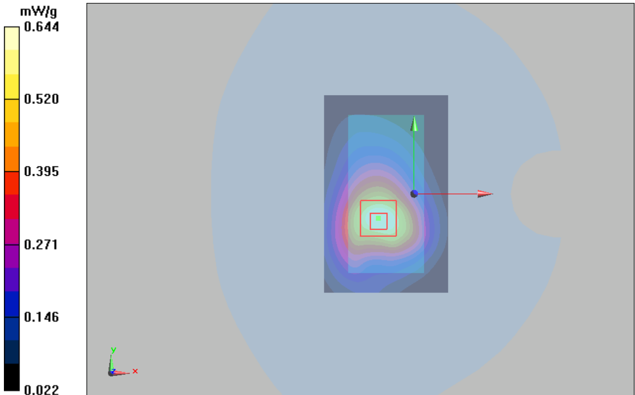
Figure 33 Body, Towards Ground, GSM 1900 GPRS (2TXslots) Channel 661 Close
