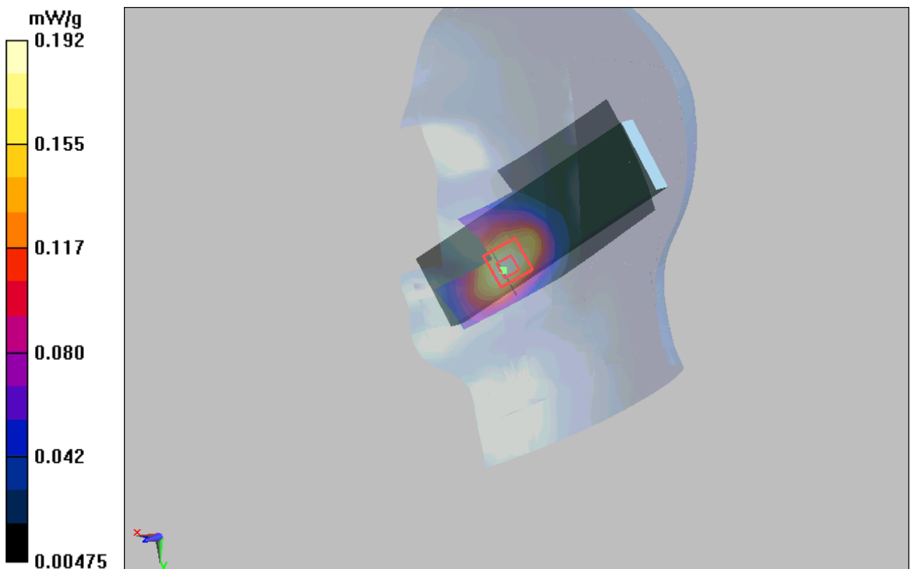
Figure 28 Right Hand Touch Cheek GSM 1900 Channel 810 Open
