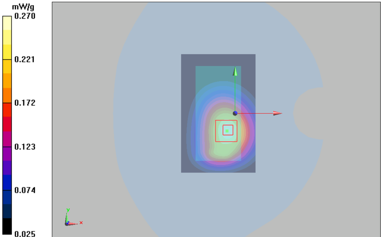
Figure 17 Body, Towards Ground, GSM 850 Channel 190 Close
