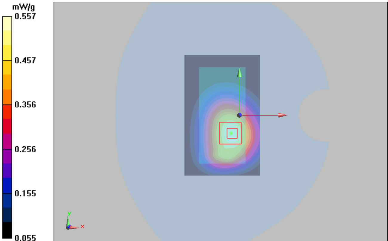
Figure 22 Body, Towards Ground, GSM 850 GPRS (4TXslots) Channel 128 Close
