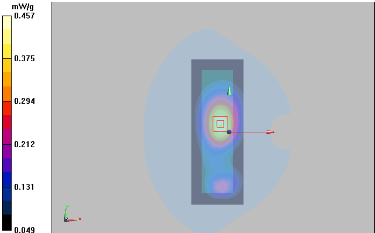
Figure 24 Body, Towards Ground, GSM 850 GPRS (4TXslots) Channel 190 Open
