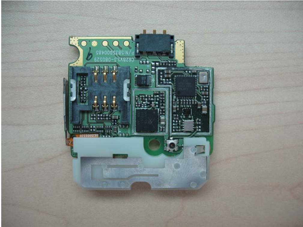
Mobile Phone Internal View -4
