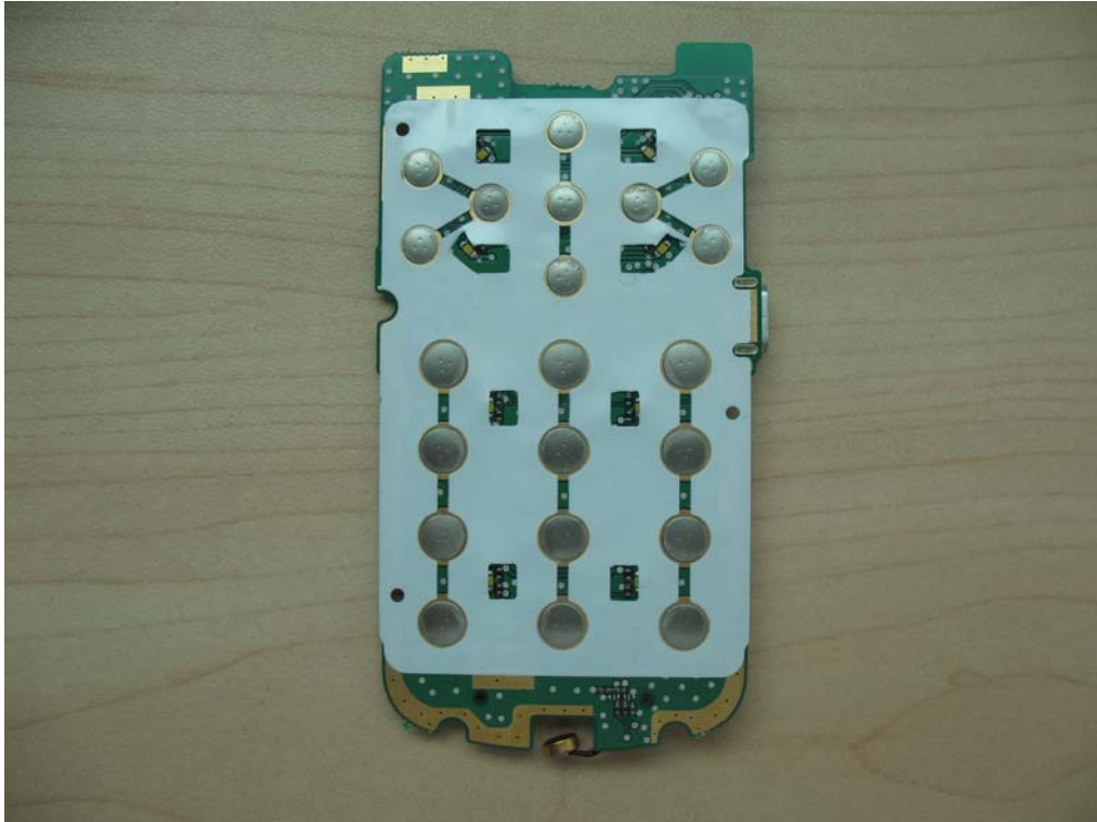
Mobile Phone Internal View -2
