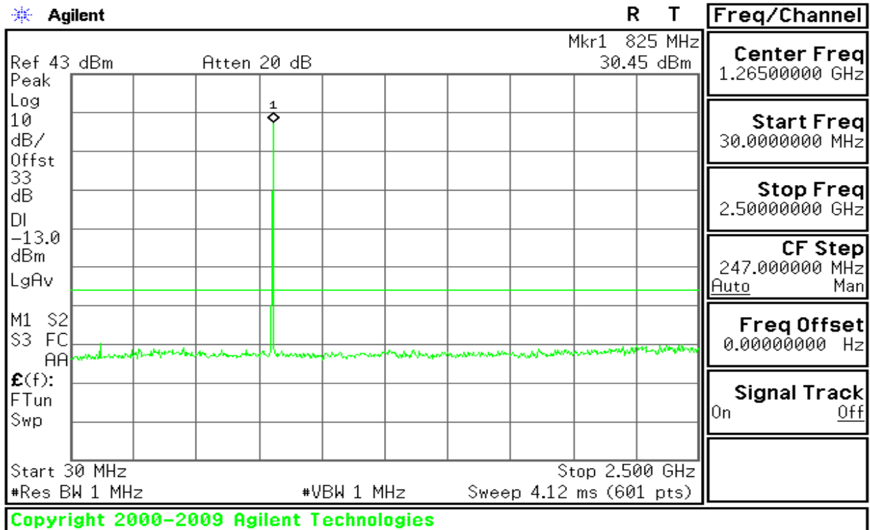
Figure 7-14: Out of Band emission at antenna terminals – EDGE CH Low
