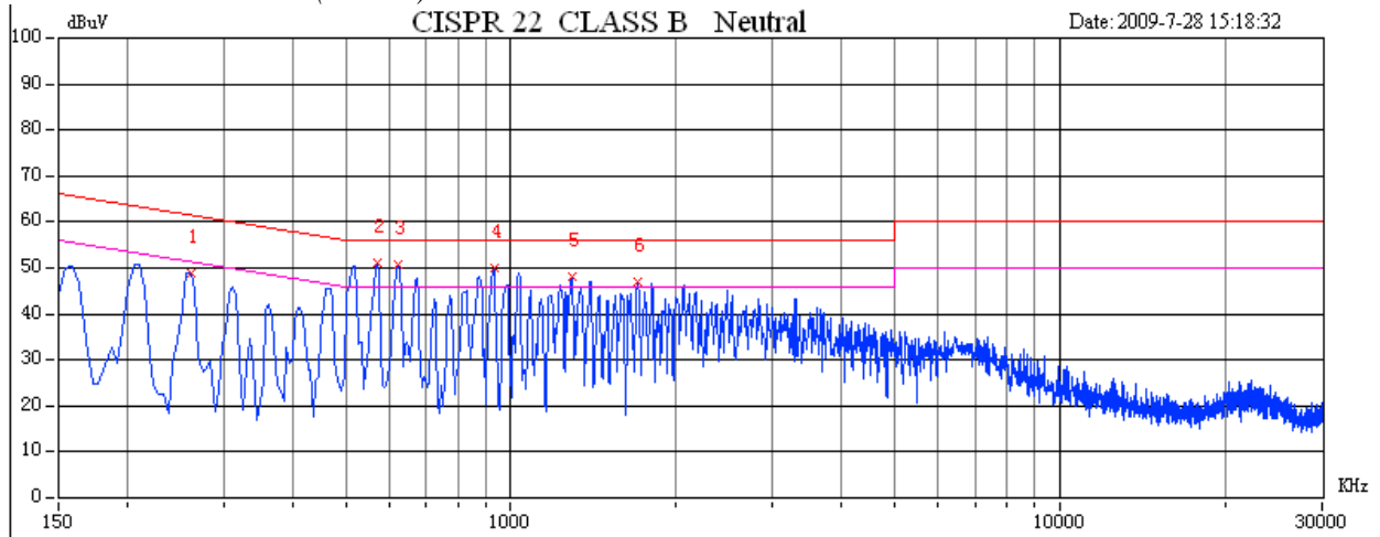
Conducted emissions (Line 2)
