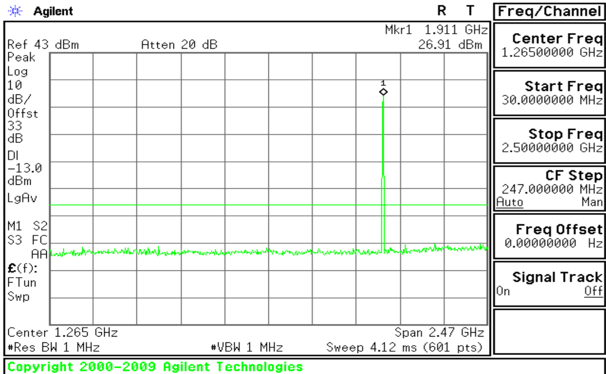
Figure 8-18: Out of Band emission at antenna terminals – EDGE CH High
