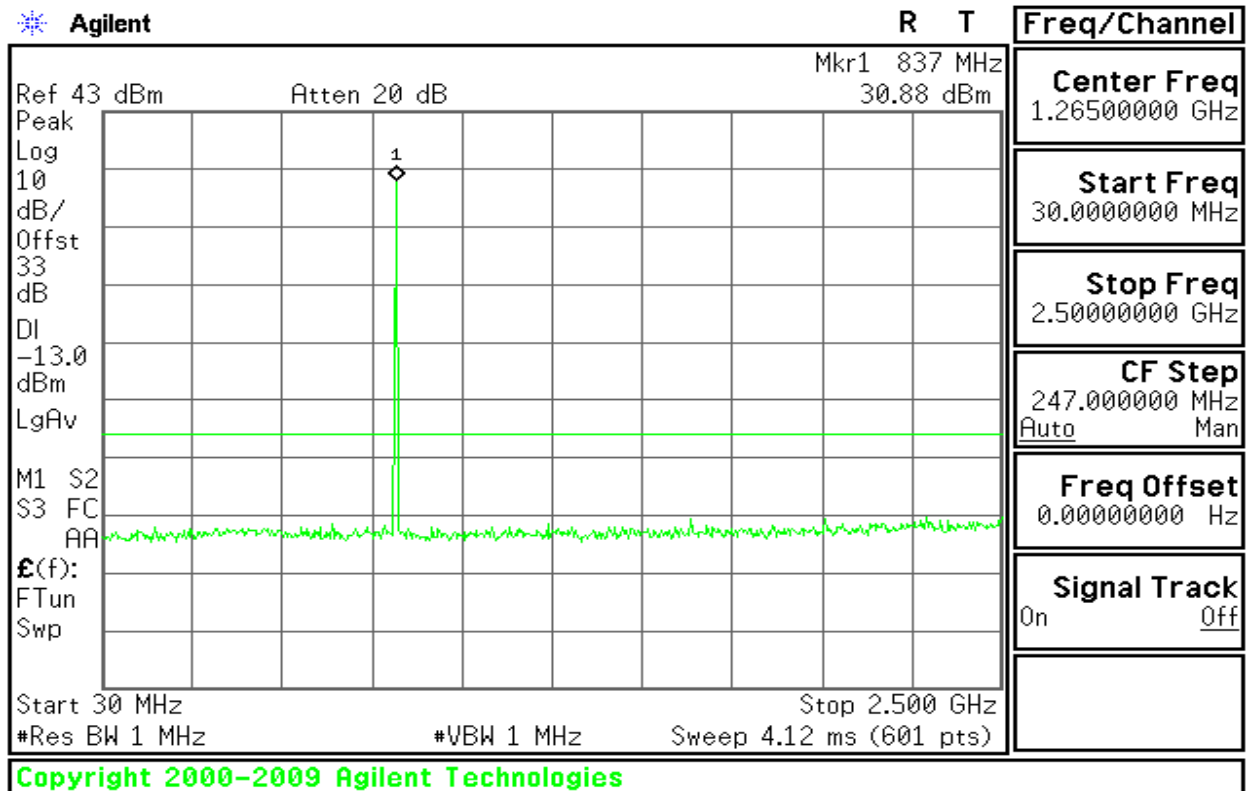
Figure 7-16: Out of Band emission at antenna terminals – EDGE CH Middle
