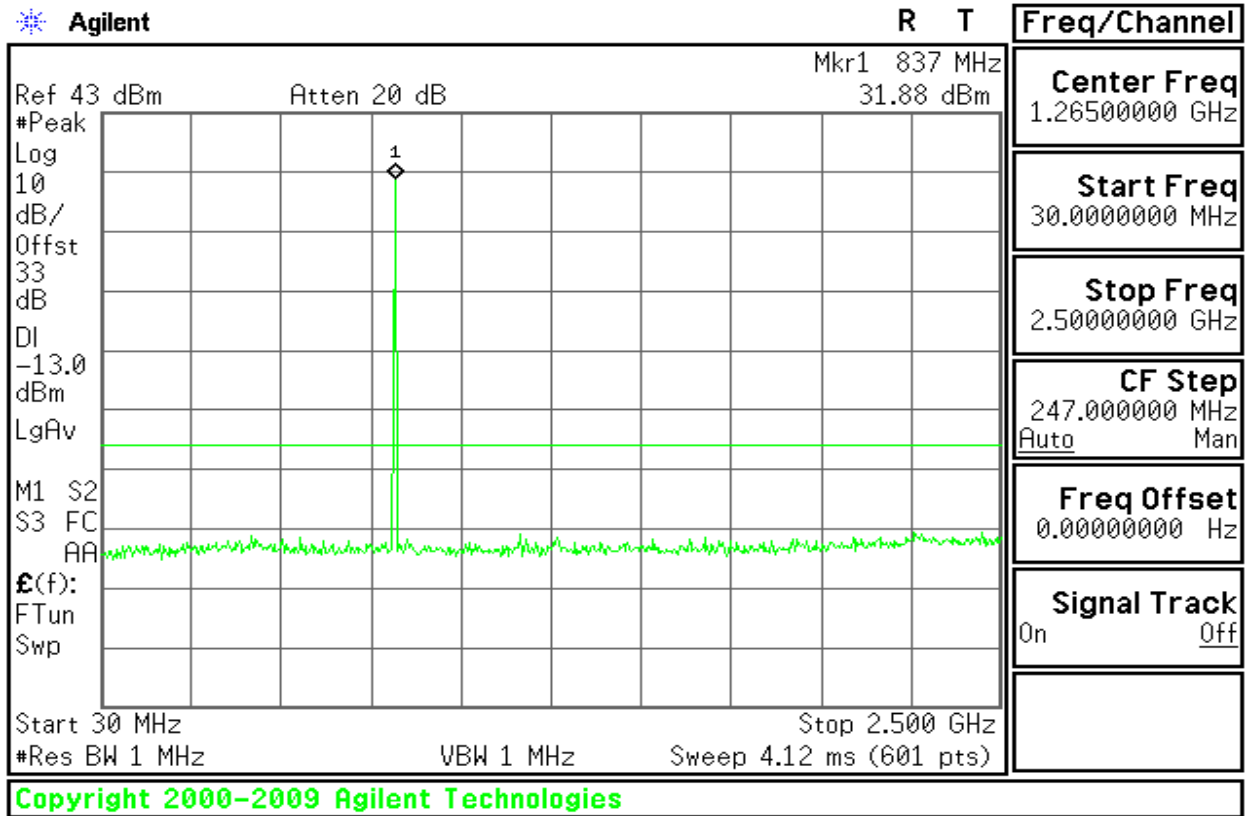
Figure 7-10: Out of Band emission at antenna terminals – GPRS CH Middle
