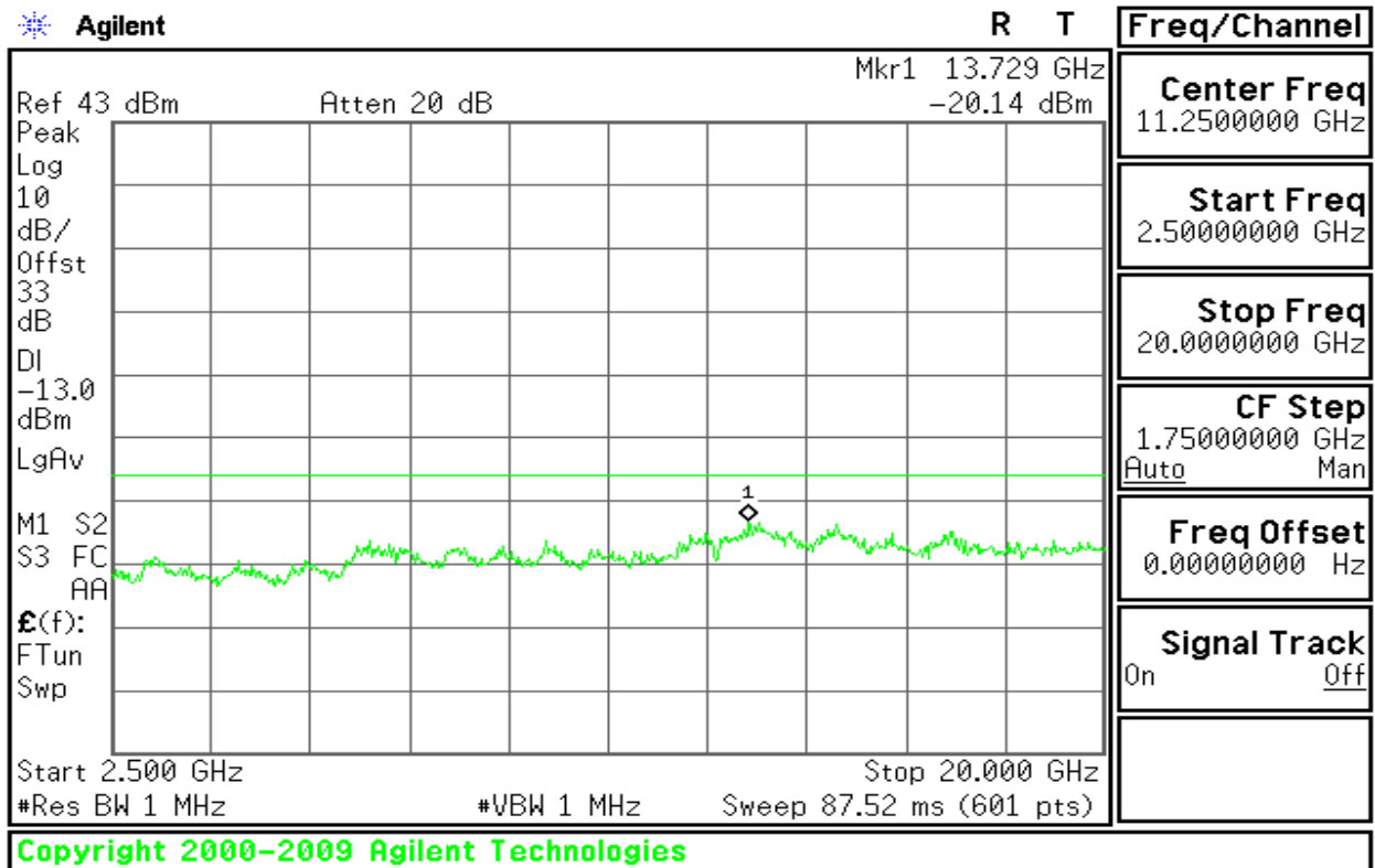
Figure 8-16: Out of Band emission at antenna terminals – EDGE CH Middle
