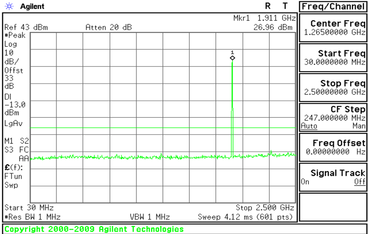
Figure 8-12: Out of Band emission at antenna terminals – GPRS CH High
