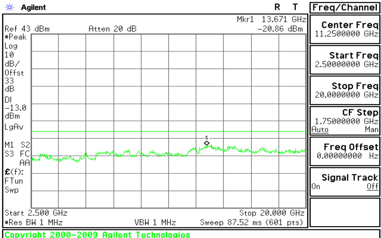
Figure 8-8: Out of Band emission at antenna terminals – GPRS CH Low
