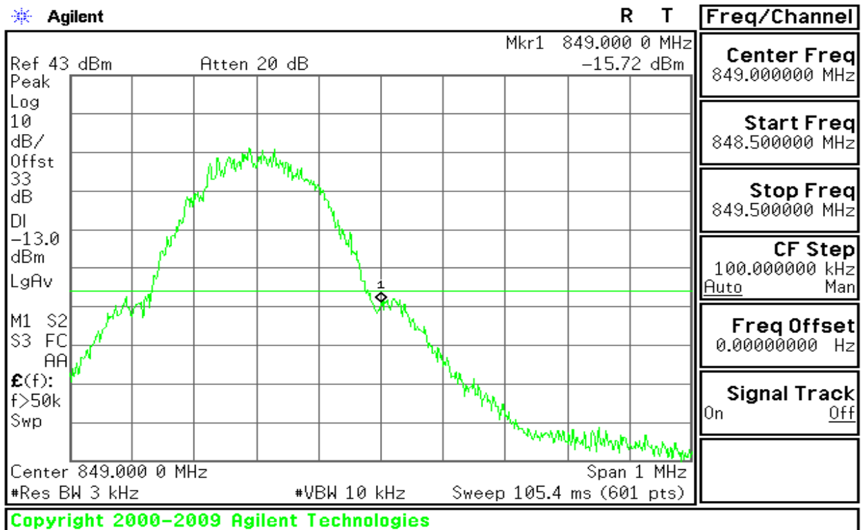
Figure 9-6: Band Edge emissions – EDGE CH High
