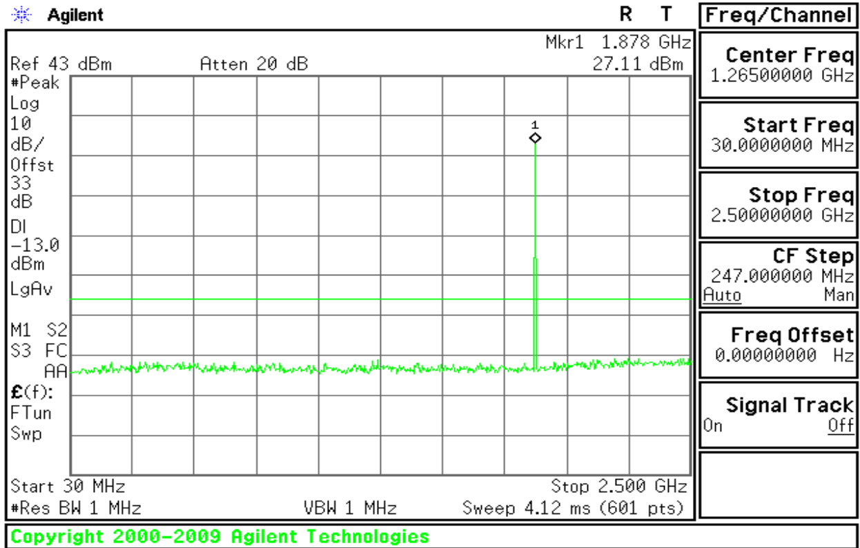
Figure 8-10: Out of Band emission at antenna terminals – GPRS CH Middle
