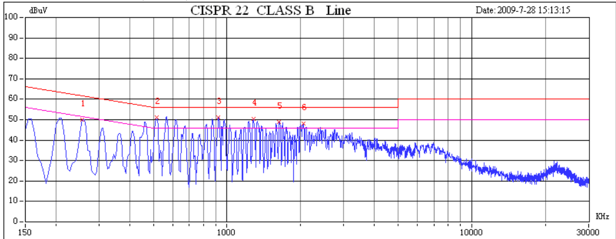
Conducted emissions (Line 1)
