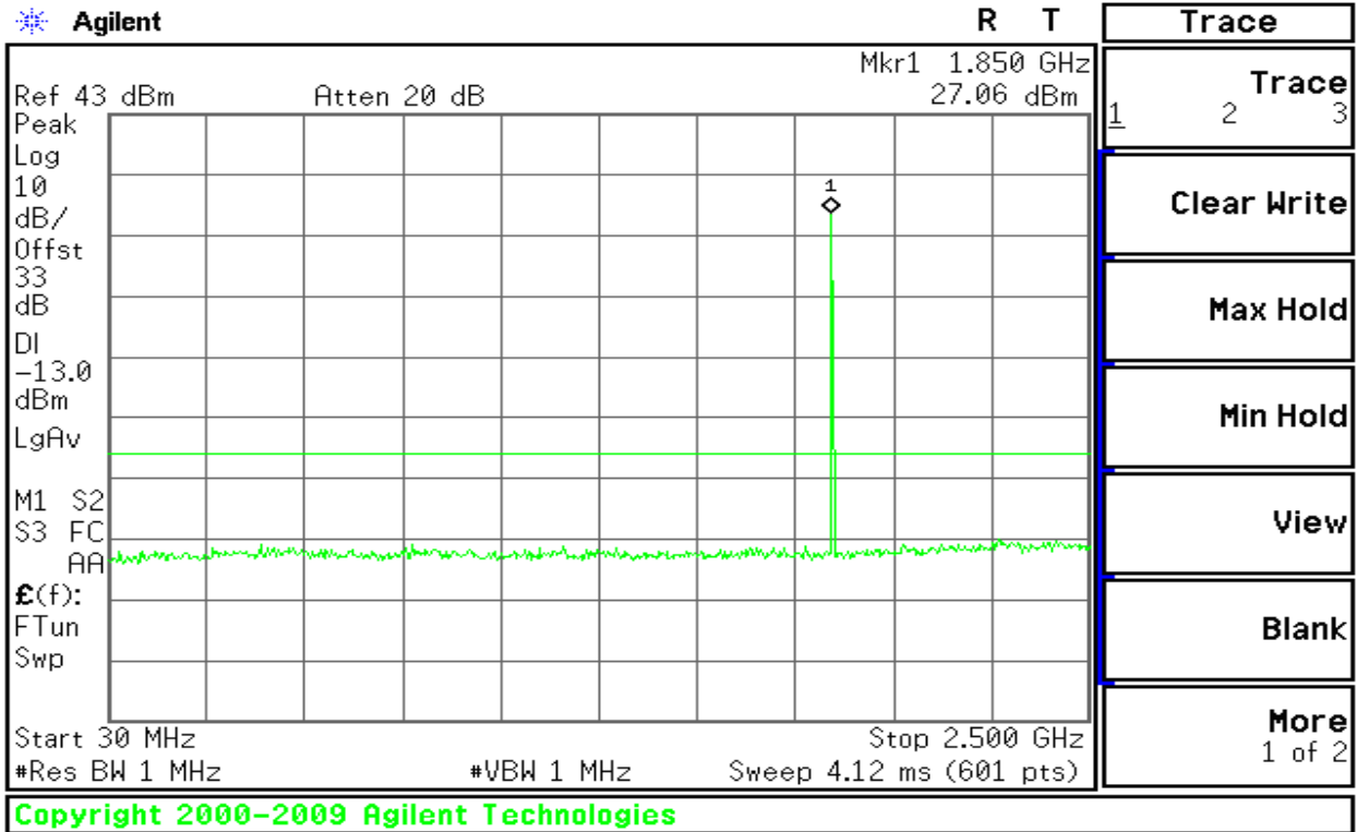
Figure 8-14: Out of Band emission at antenna terminals – EDGE CH Low
