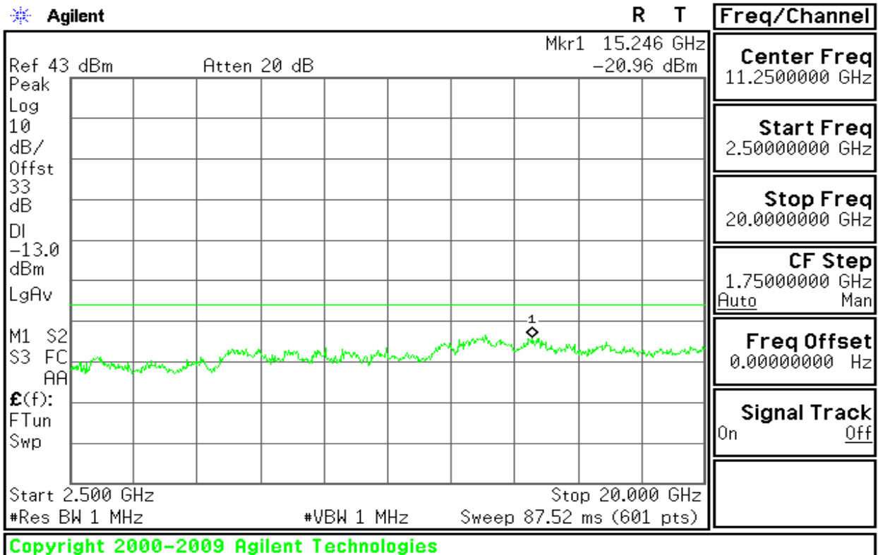
Figure 8-14: Out of Band emission at antenna terminals – EDGE CH Low
