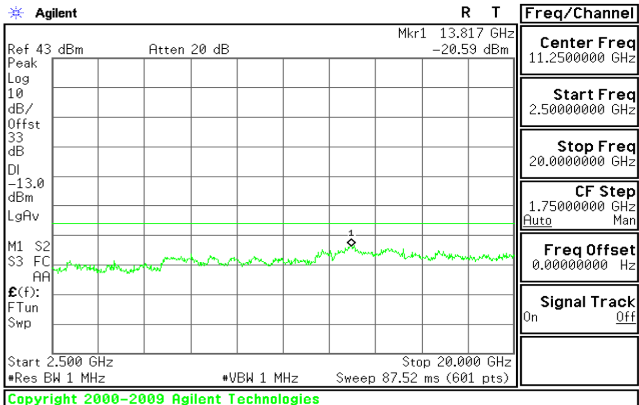
Figure 8-18: Out of Band emission at antenna terminals – EDGE CH High
