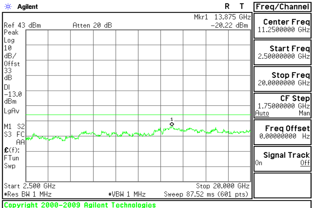
Figure 7-16: Out of Band emission at antenna terminals – EDGE CH Middle
