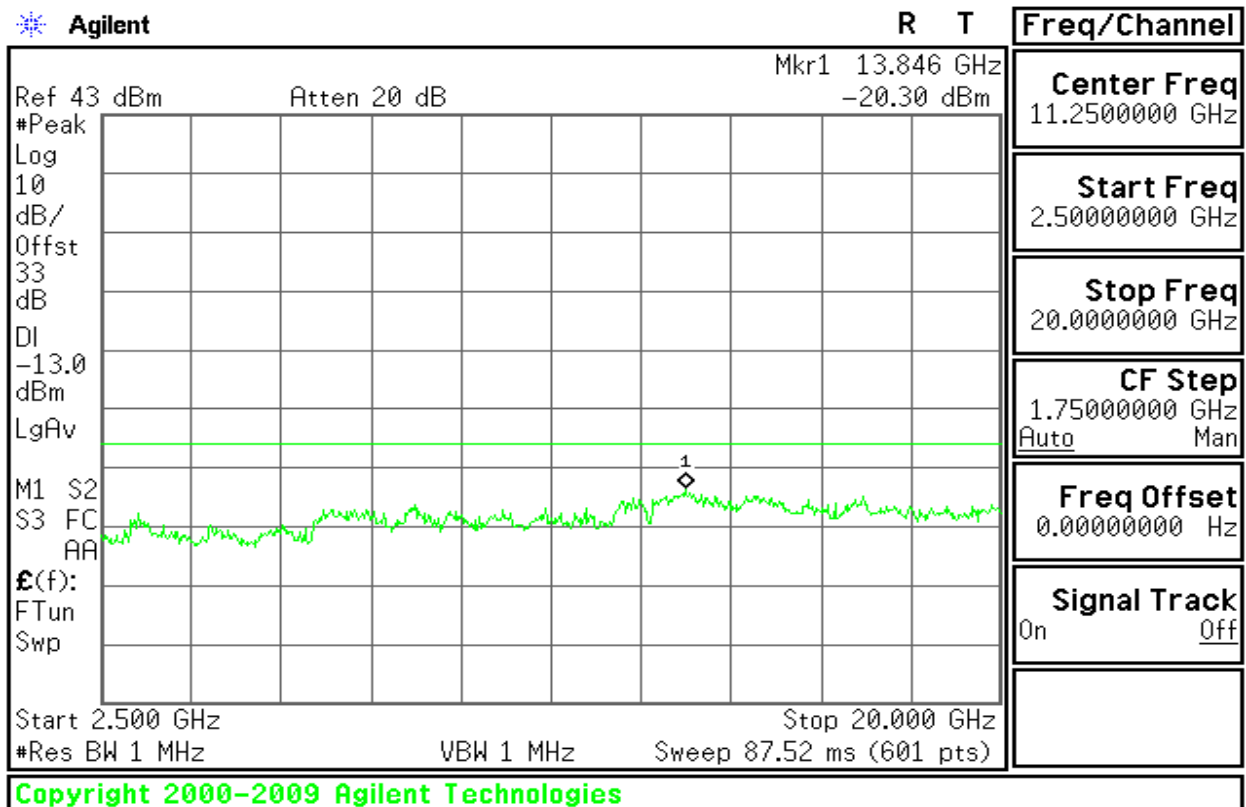
Figure 7-10: Out of Band emission at antenna terminals – GPRS CH Middle
