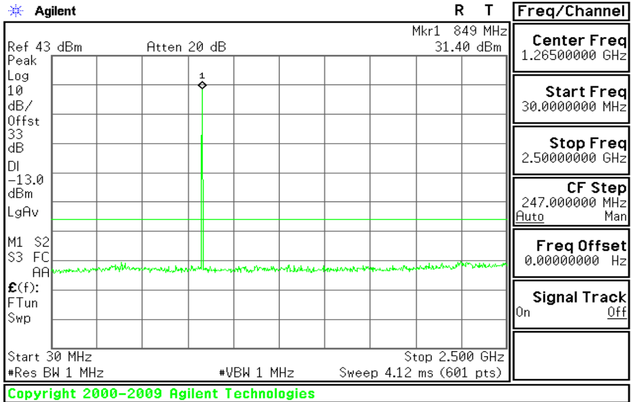
Figure 7-18: Out of Band emission at antenna terminals – EDGE CH High
