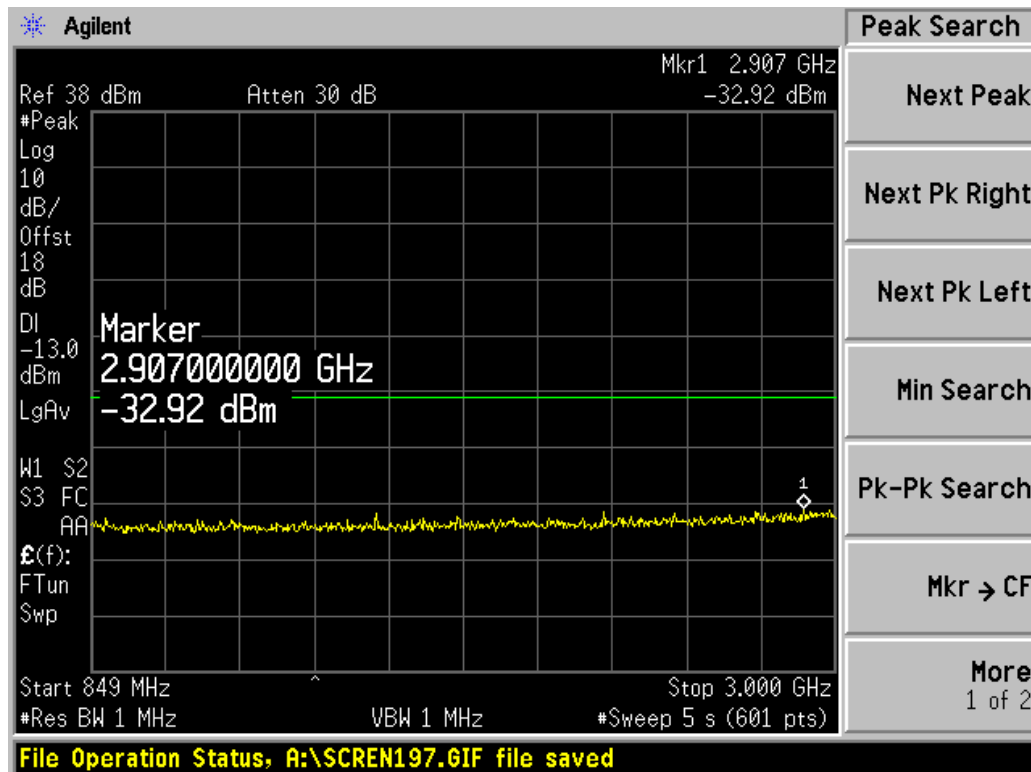
Channel 189, 849MHz~3GHz
