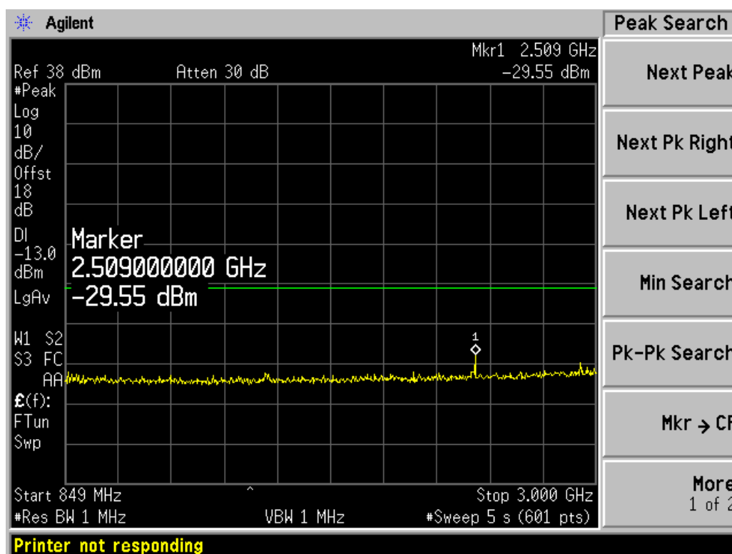
Channel 189, 849MHz~3GHz
