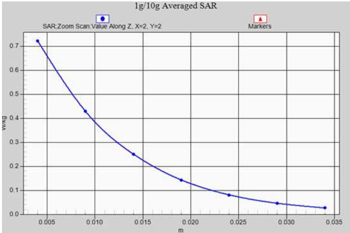
GSM1900/Back side with headset-Low_ z-axis scan
