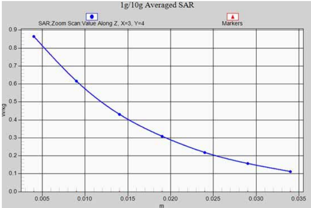
GSM850/Back side with headset-High_ z-axis scan
