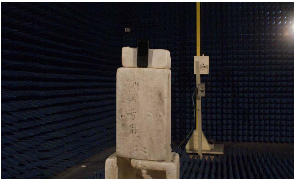
RADIATED EMISSION TEST SETUP
