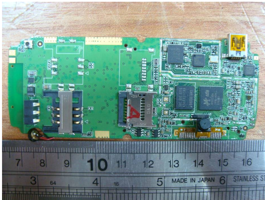
EUT – Main Board without Shielded View
