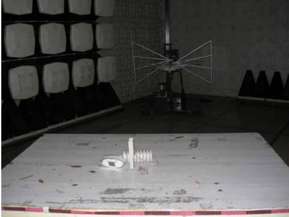
The Field Strength of Radiation Emission (Below 1GHz)
