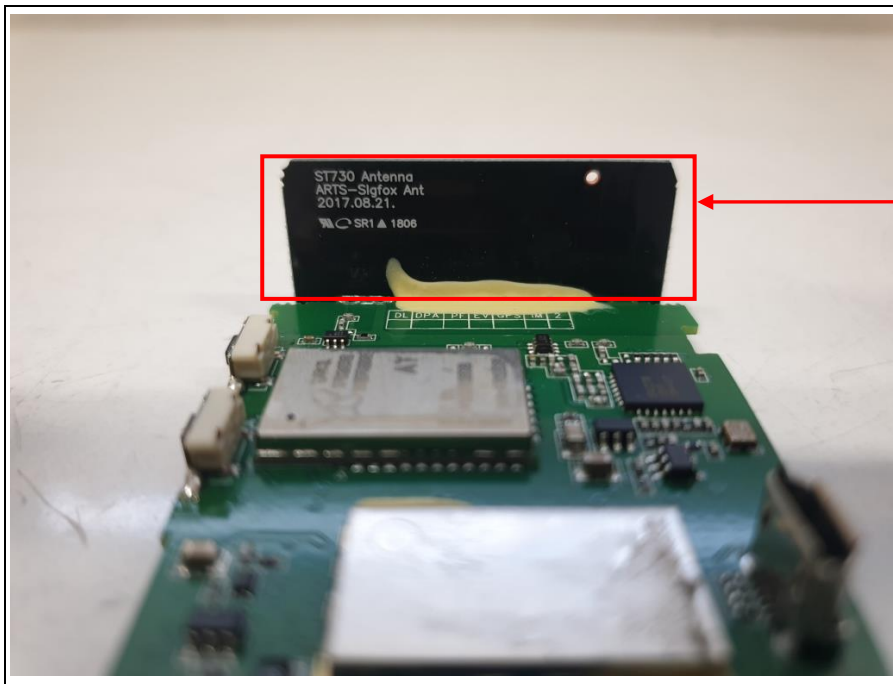
PCB Antenna
