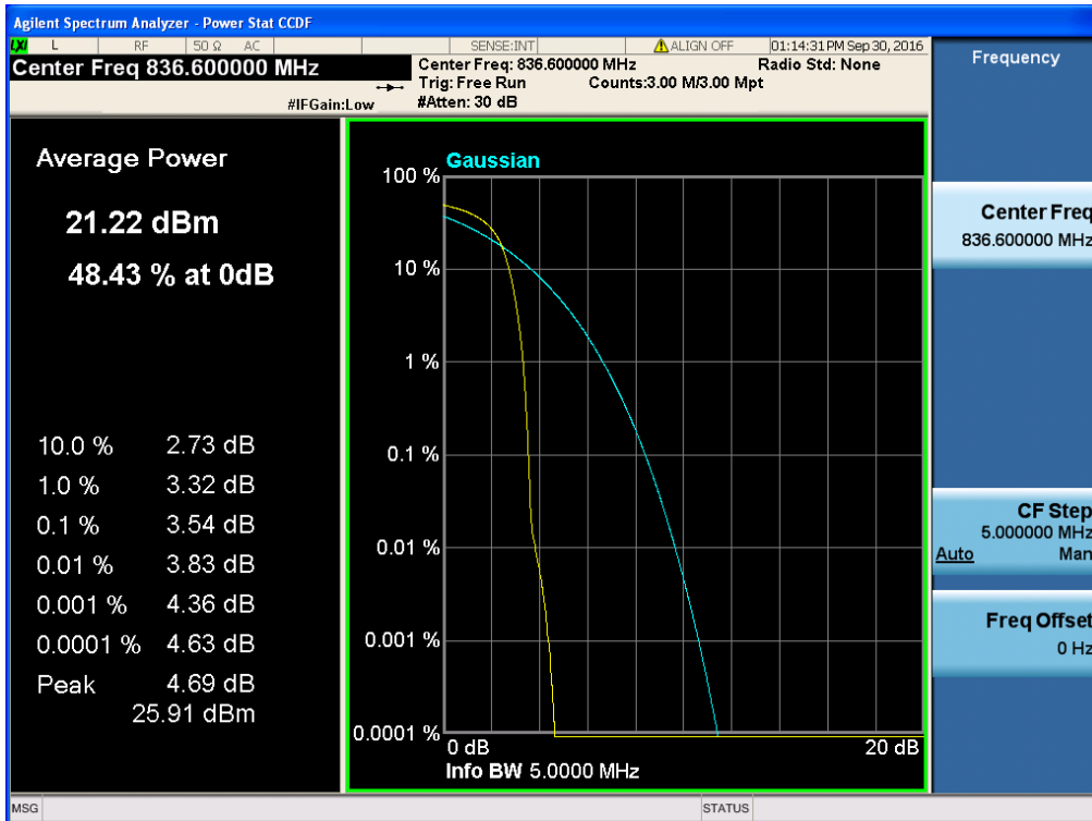
HSUPA850 & Channel: 4183
