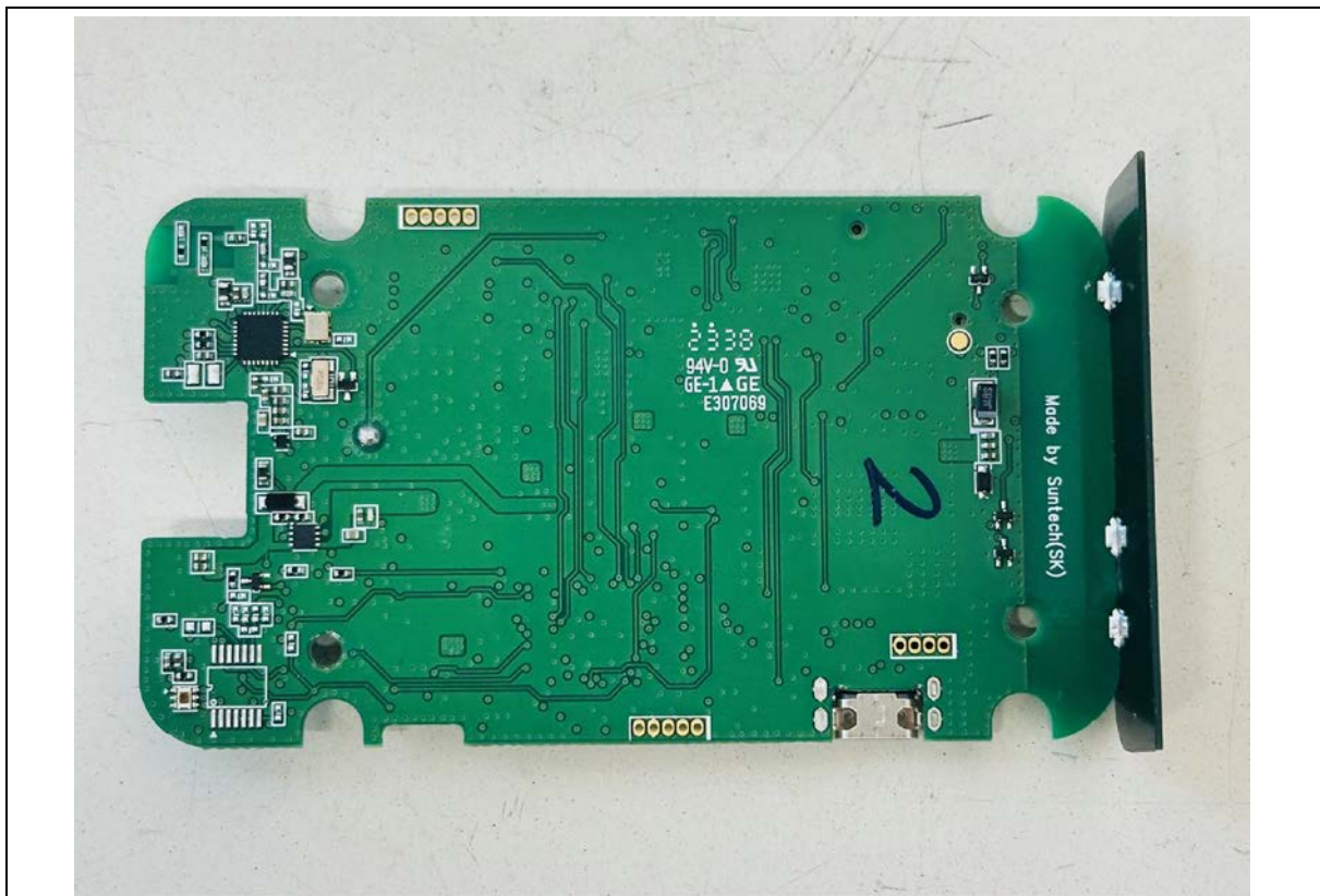
Bottom view of Main PCB
