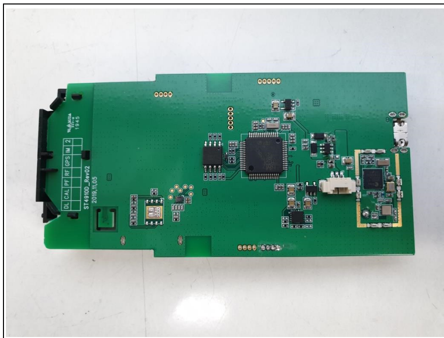
Bottom view of Main PCB without shield
