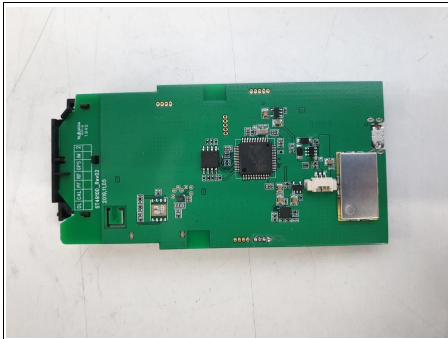
Bottom view of Main PCB with shield
