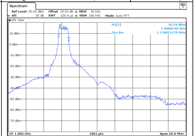
16QAM High Channel (99 % Occupied Bandwidth)
