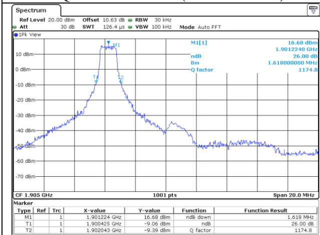
16QAM High Channel (26 dB Bandwidth)
