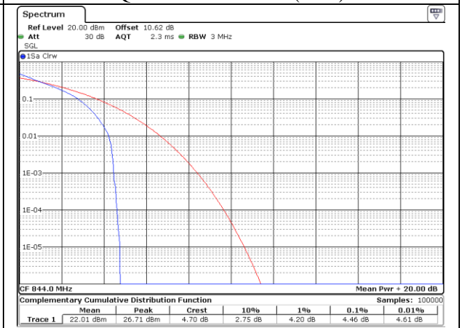
QPSK High Channel (6 RB)
