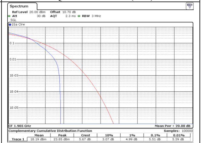
16QAM High Channel (6 RB)
