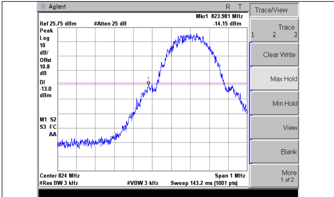
- Lower band Edge emissions, GSM850 -
