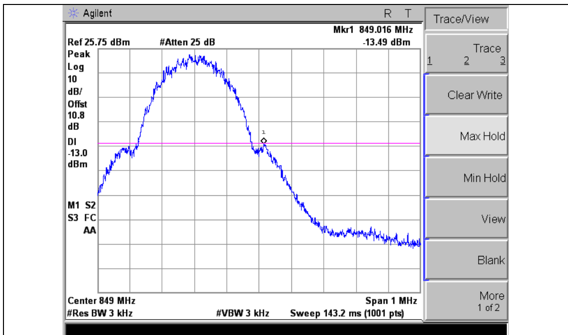
- Upper band Edge emissions, GSM850 -
