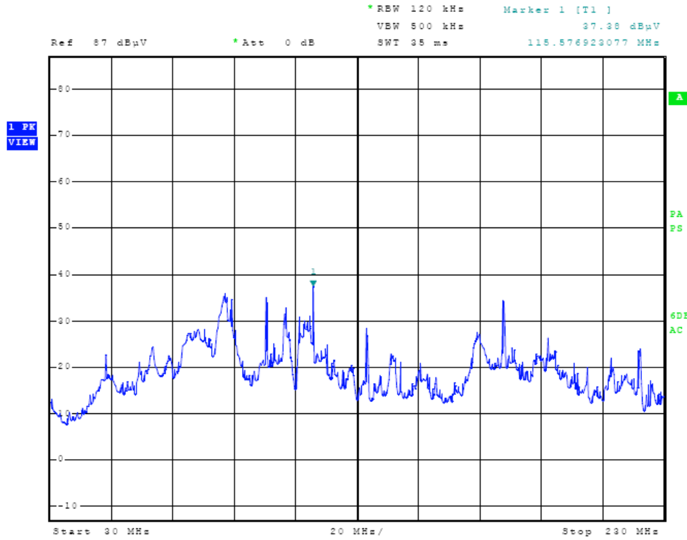
Figure Three Radiated Emissions in screen room
