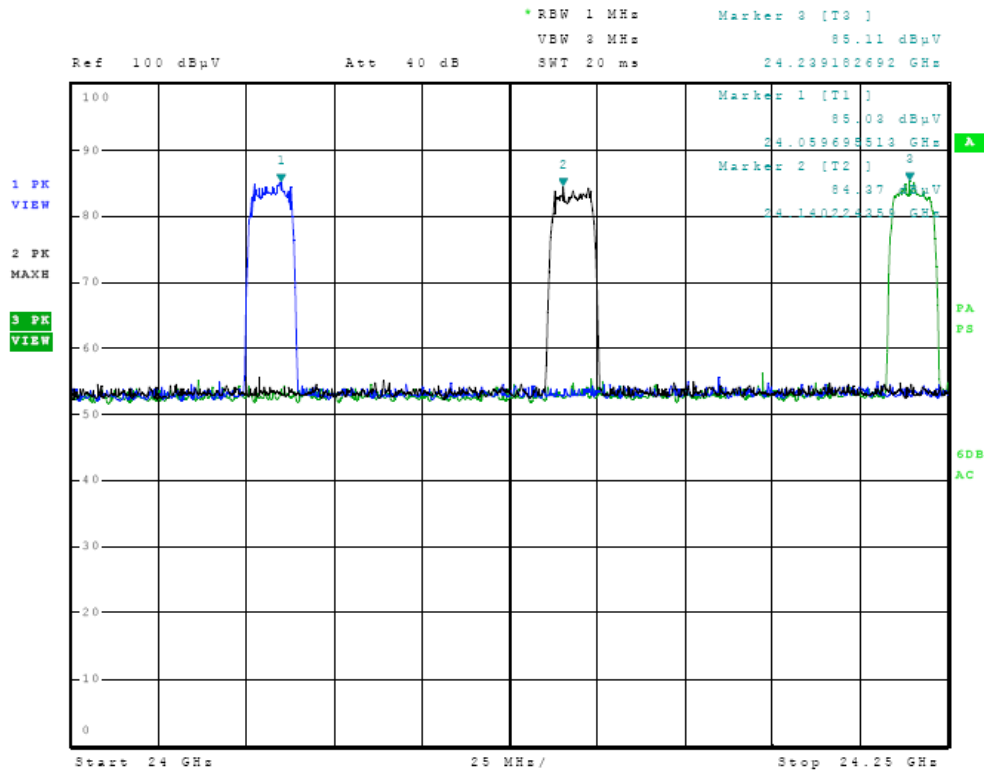
Figure Thirteen Output power across band
