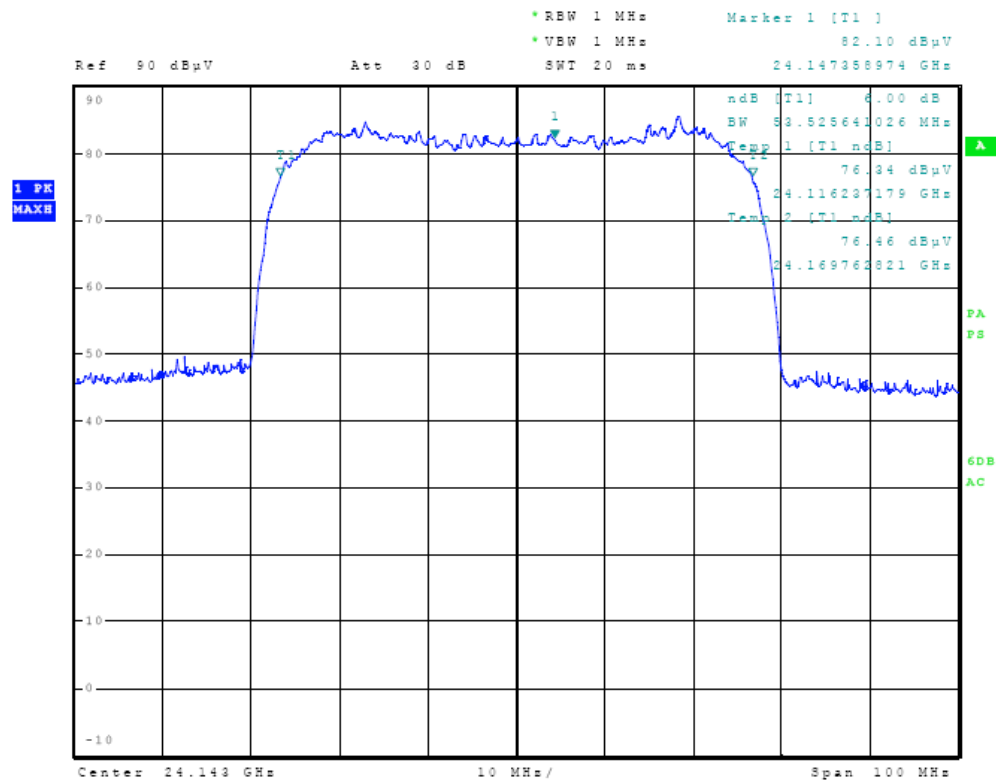
Figure Sixteen Occupied Bandwidth (56 MHz Bandwidth Operation)
