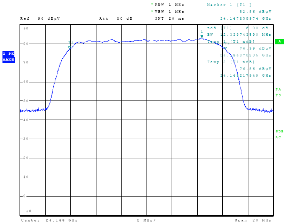
Figure Fourteen Occupied Bandwidth (14 MHz Bandwidth Operation)
