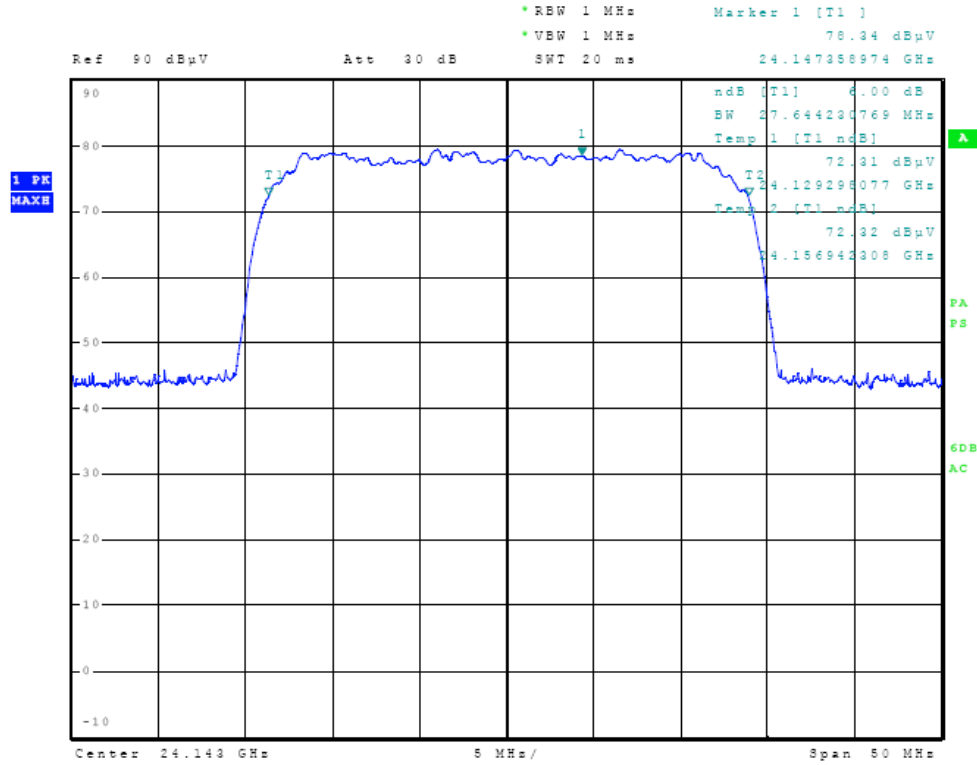
Figure Fifteen Occupied Bandwidth (30 MHz Bandwidth Operation)
