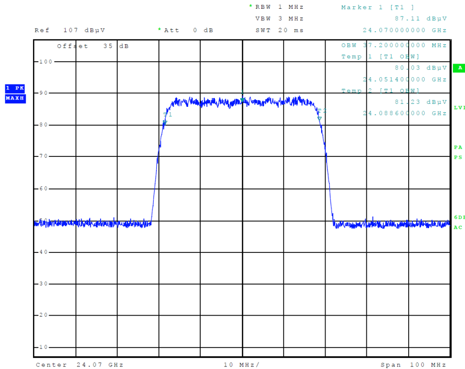
Figure Six 99% Occupied Bandwidth (40 MHz Operation)
