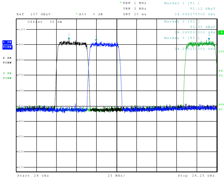
Figure Three Radiated Emissions in Band (40 MHz Channels Across the Frequency Band)
