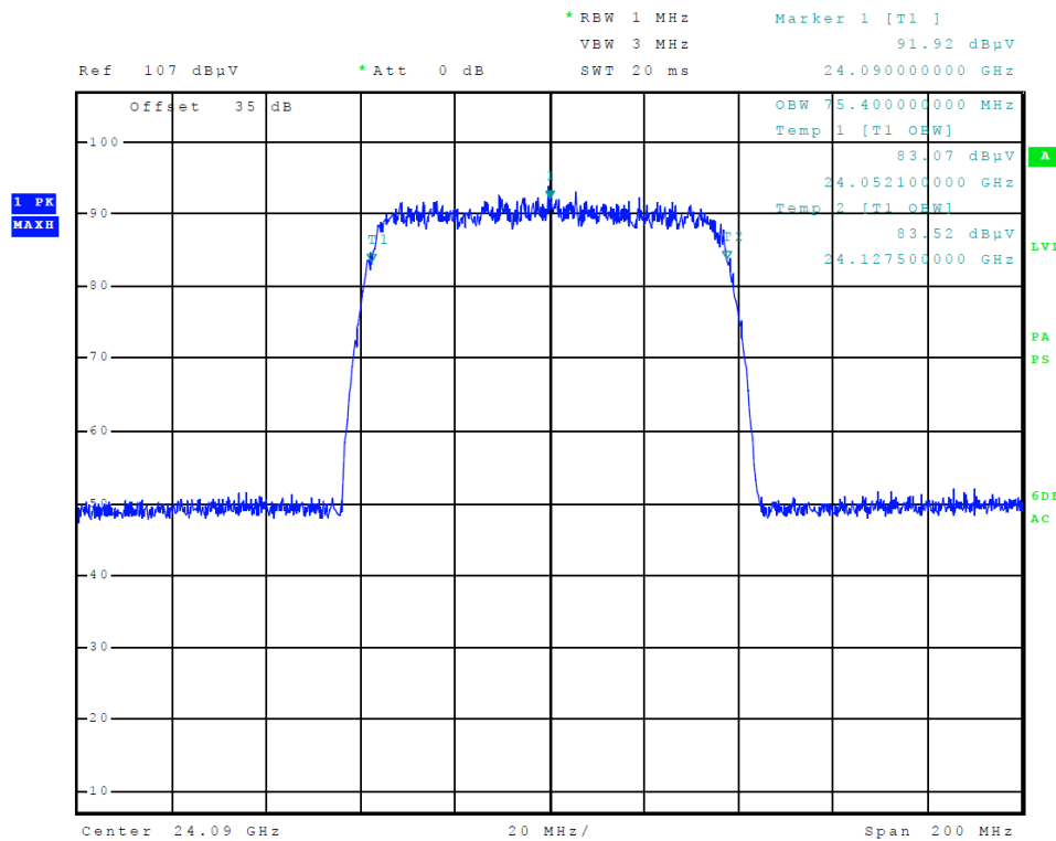
Figure Eight 99% Occupied Bandwidth (80 MHz Operation)
