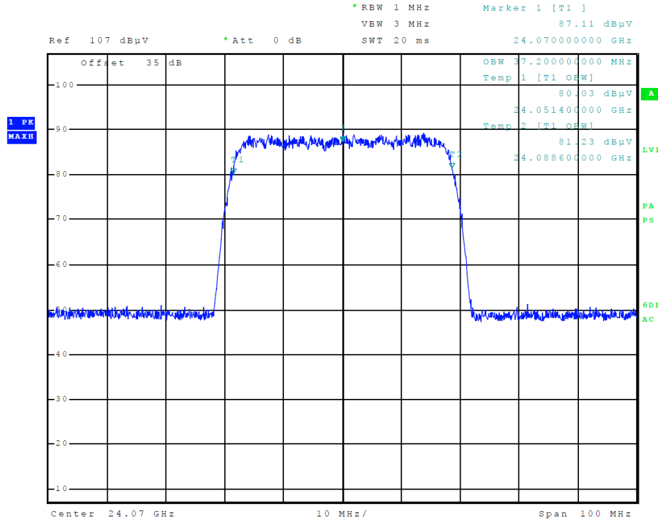
Figure Five 99% Occupied Bandwidth (40 MHz Operation)
