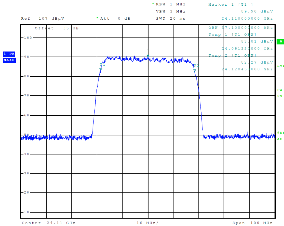
Figure Seven 99% Occupied Bandwidth (40 MHz Operation)
