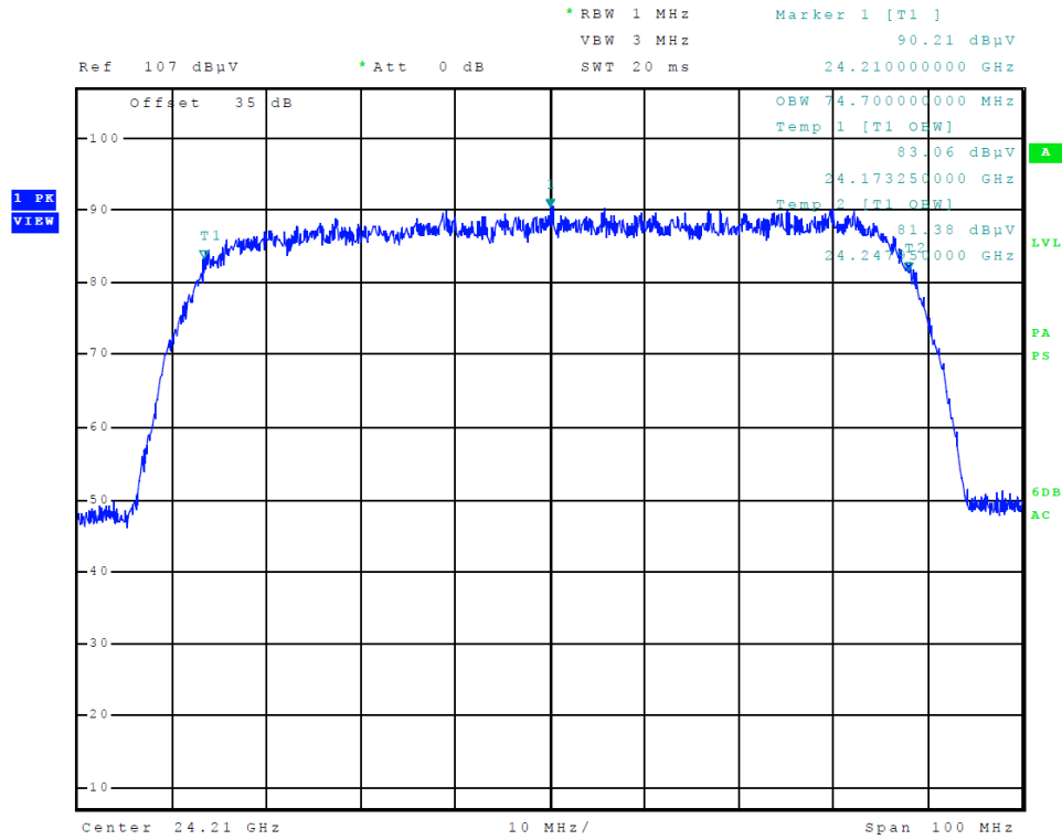
Figure Nine 99% Occupied Bandwidth (80 MHz Operation)
