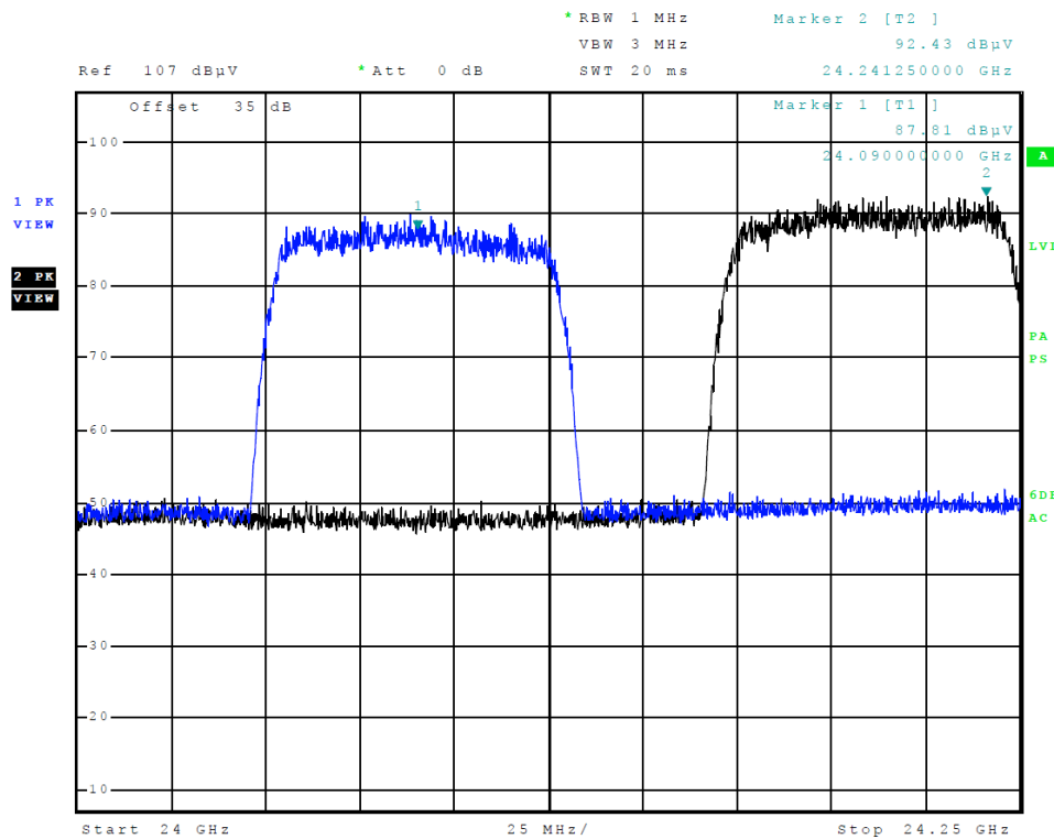
Figure Four Radiated Emissions in Band (80 MHz Channels Across the Frequency Band)
