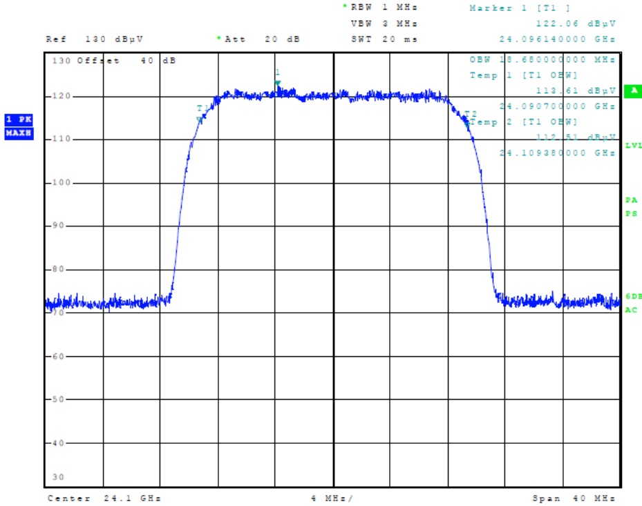
Figure Seventeen 99% Occupied Bandwidth (20 MHz Operation)
