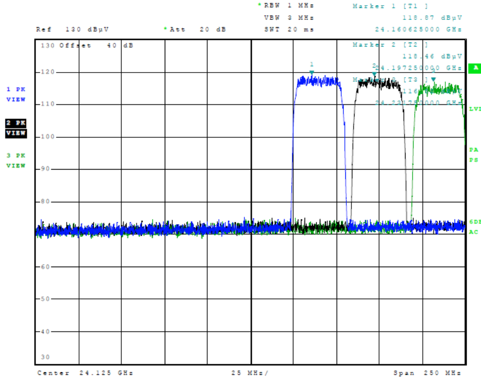
Figure Thirteen Radiated Emissions in Band (30 MHz Channels High)
