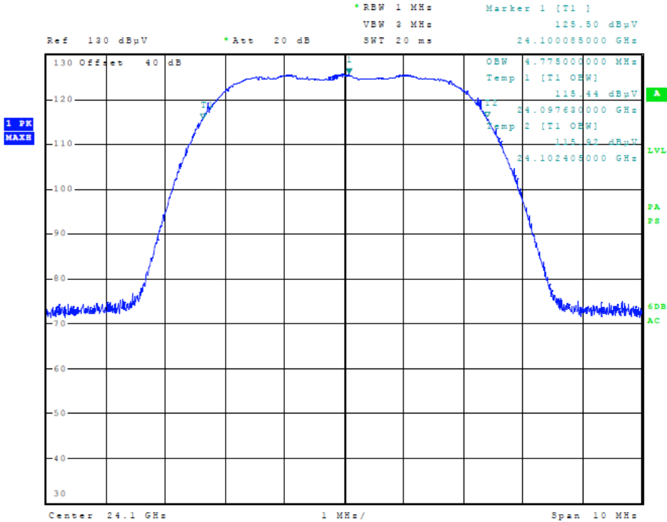
Figure Fifteen 99% Occupied Bandwidth (5 MHz Operation)
