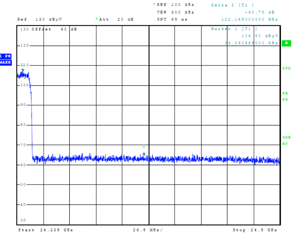
Figure Twenty-Five Out-Of-Band Emissions (30 MHz Operation)
