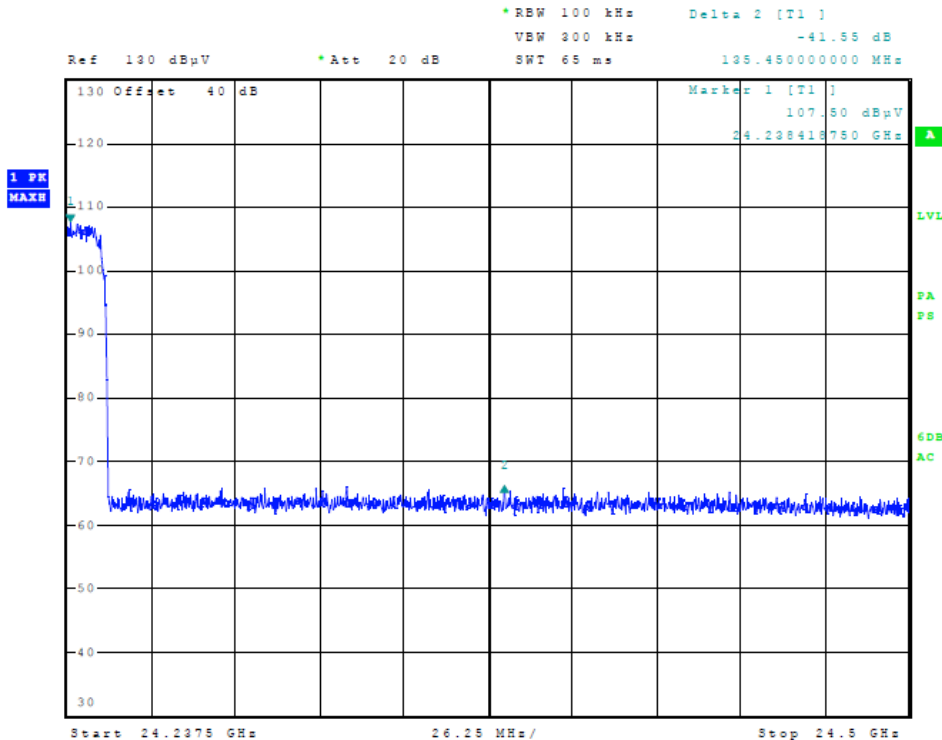
Figure Twenty-Four Out-Of-Band Emissions (25 MHz Operation)
