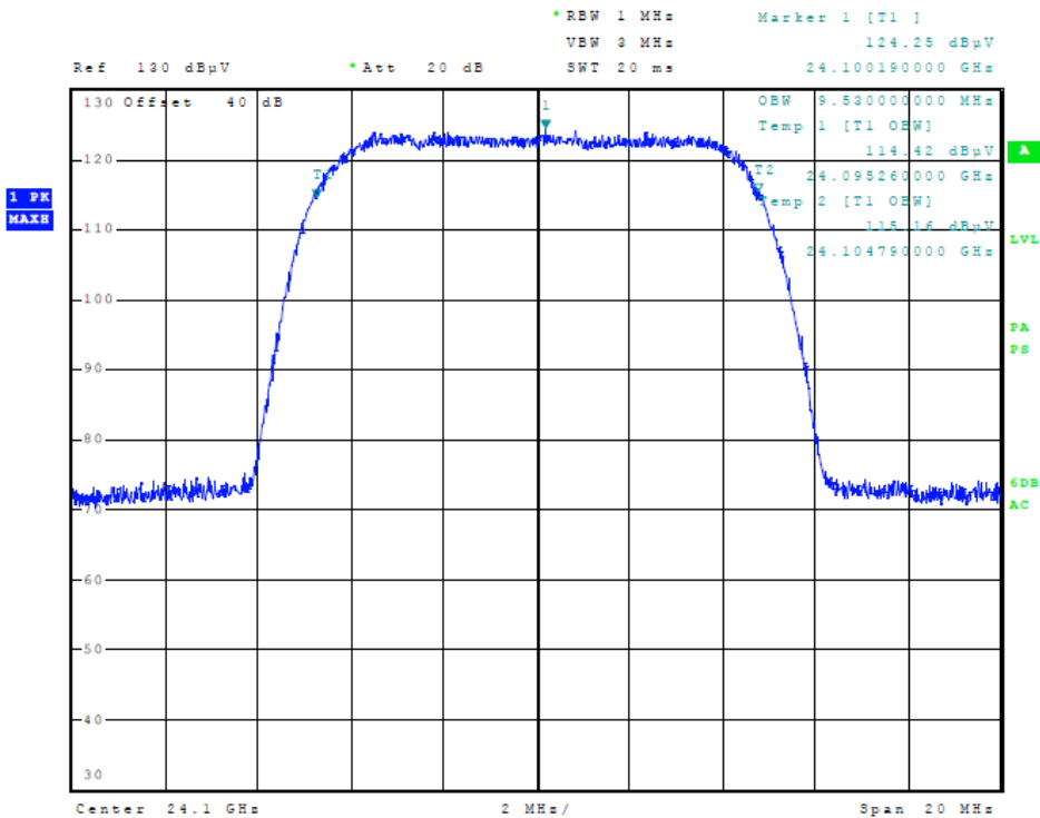
Figure Sixteen 99% Occupied Bandwidth (10 MHz Operation)
