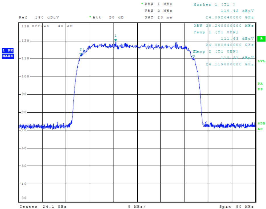
Figure Twenty 99% Occupied Bandwidth (40 MHz Operation)
