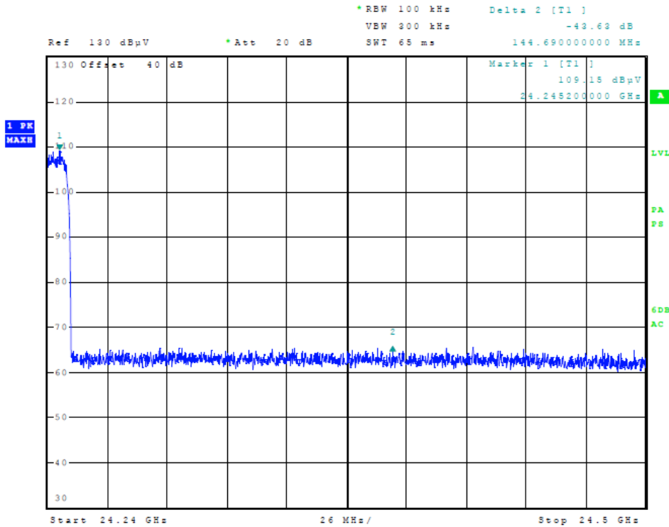
Figure Twenty-Three Out-Of-Band Emissions (20 MHz Operation)
