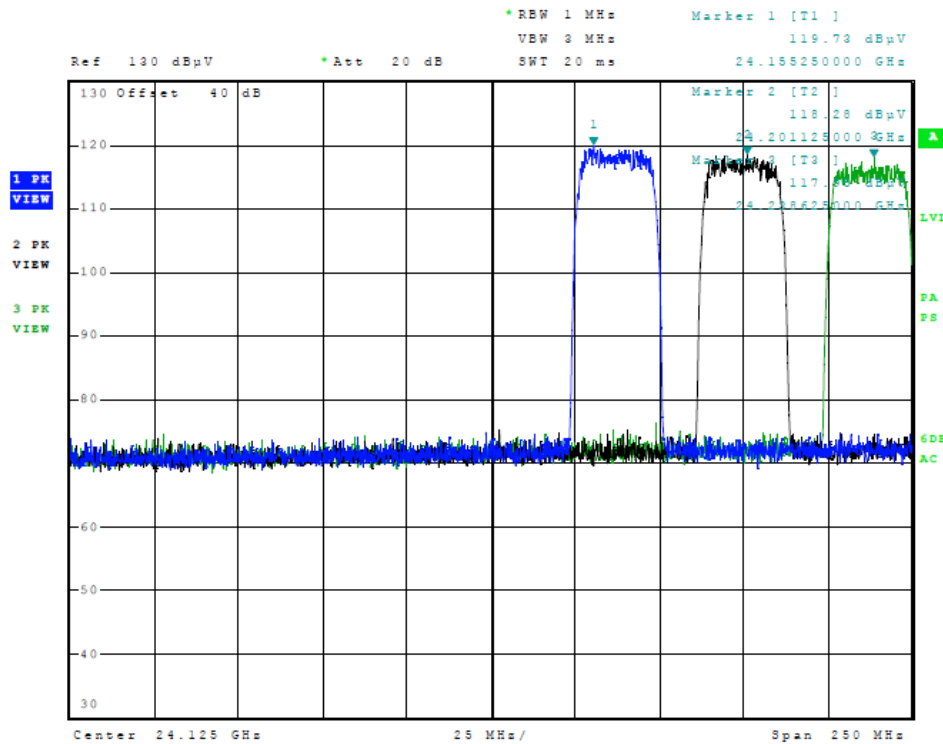
Figure Twelve Radiated Emissions in Band (25 MHz Channels High)
