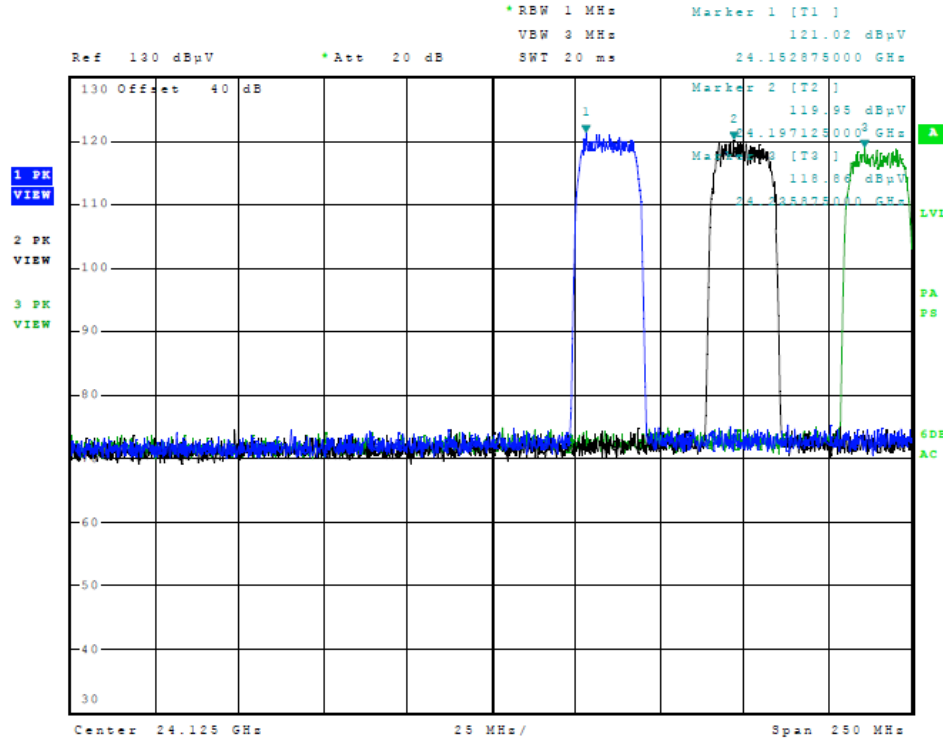
Figure Eleven Radiated Emissions in Band (20 MHz Channels High)
