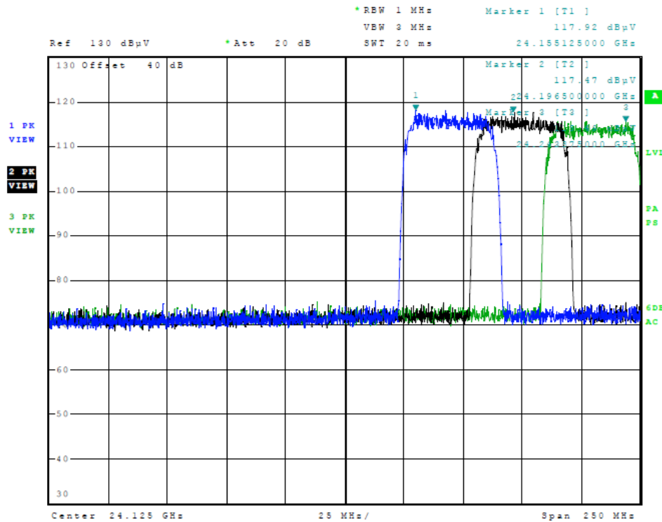
Figure Fourteen Radiated Emissions in Band (40 MHz Channels High)
