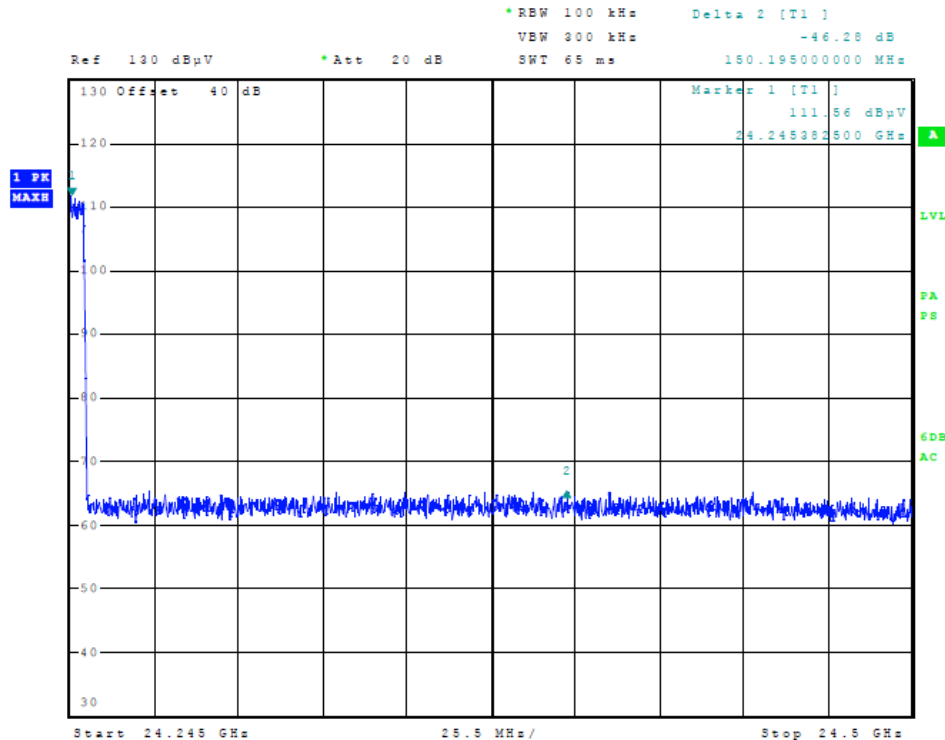
Figure Twenty-Two Out-Of-Band Emissions (10 MHz Operation)
