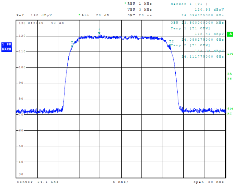
Figure Eighteen 99% Occupied Bandwidth (25 MHz Operation)
