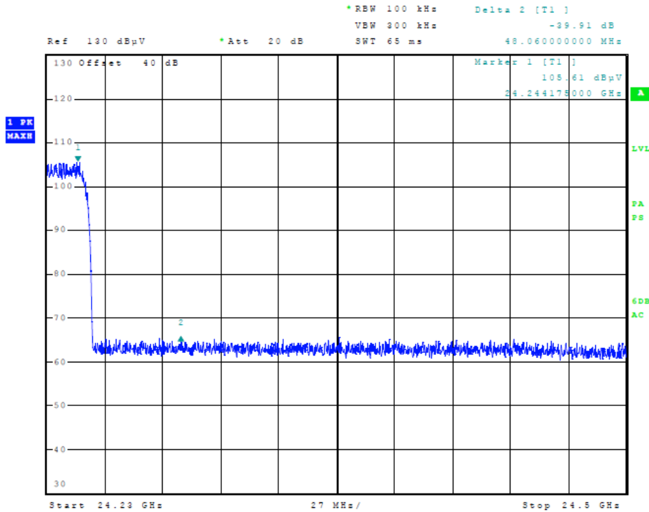
Figure Twenty-Six Out-Of-Band Emissions (40 MHz Operation)
