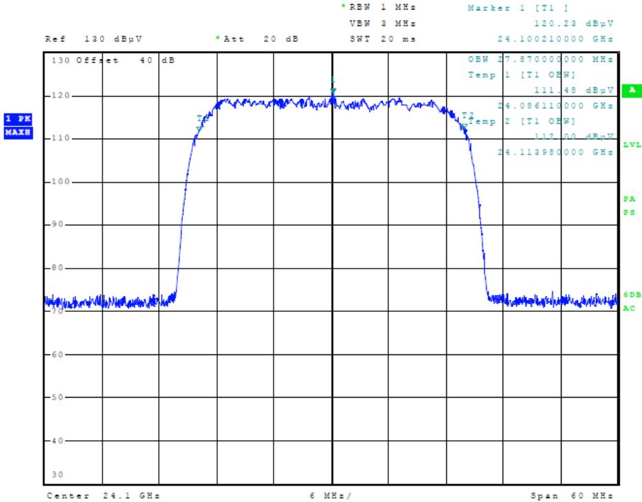
Figure Nineteen 99% Occupied Bandwidth (30 MHz Operation)
