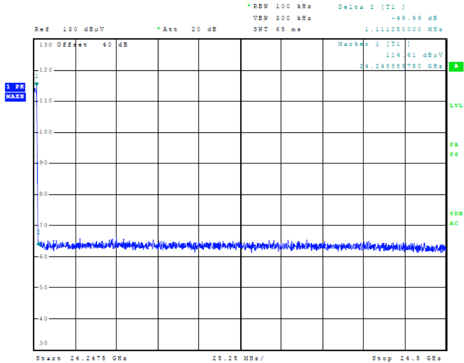
Figure Twenty-One Out-Of-Band Emissions (5 MHz Operation)
