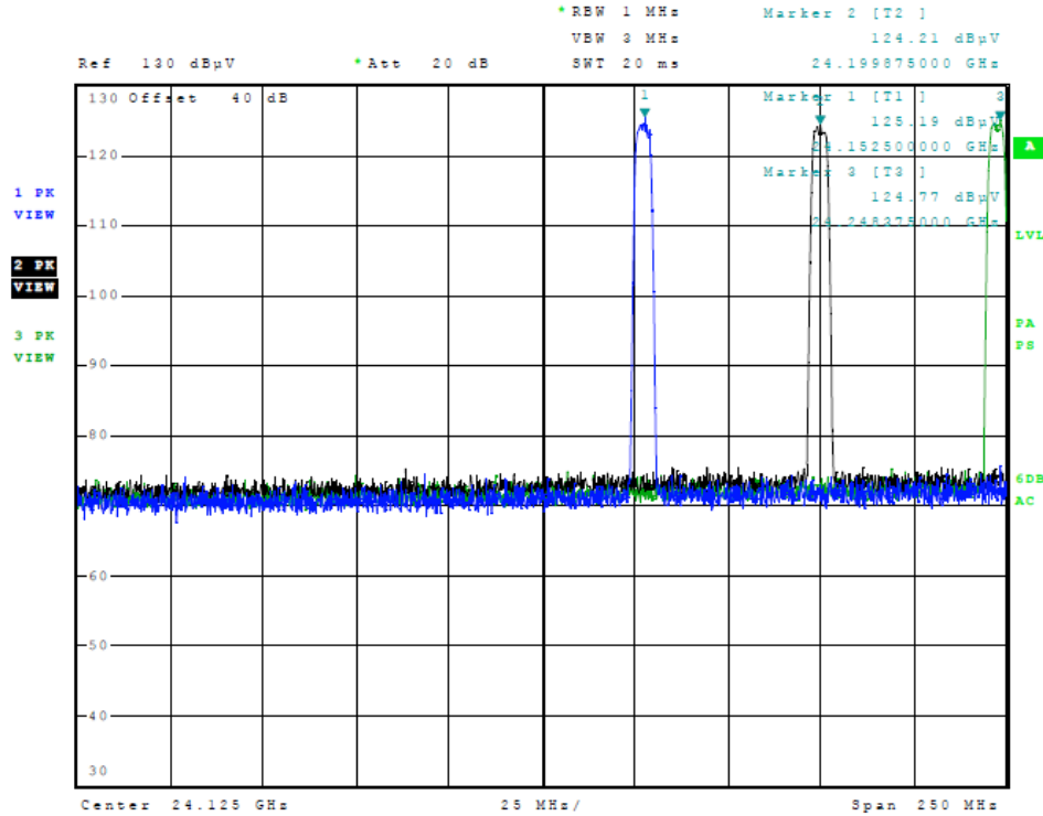
Figure Nine Radiated Emissions in Band (5 MHz Channels High)
