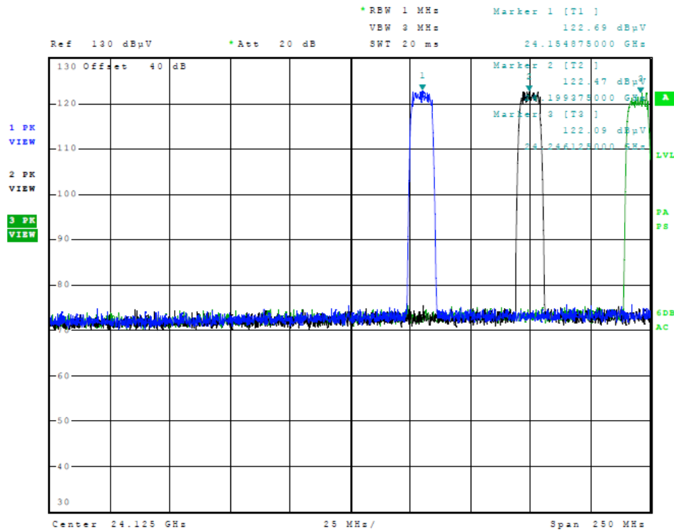
Figure Ten Radiated Emissions in Band (10 MHz Channels High)
