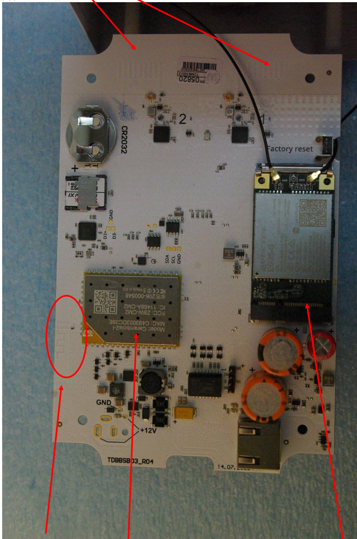
2.4 GHz Antenna and module
