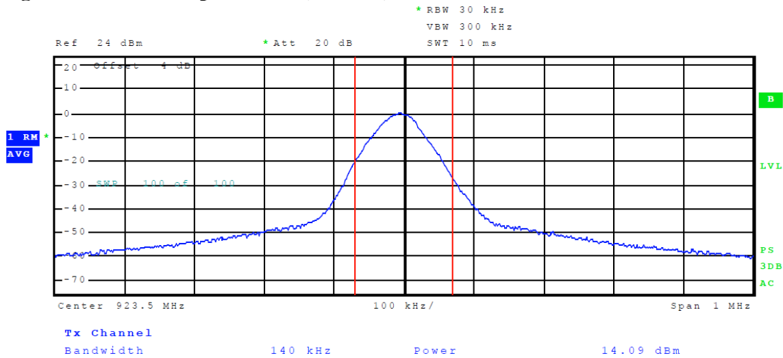
Figure 22 Plot of Output Power (P-Mode)
