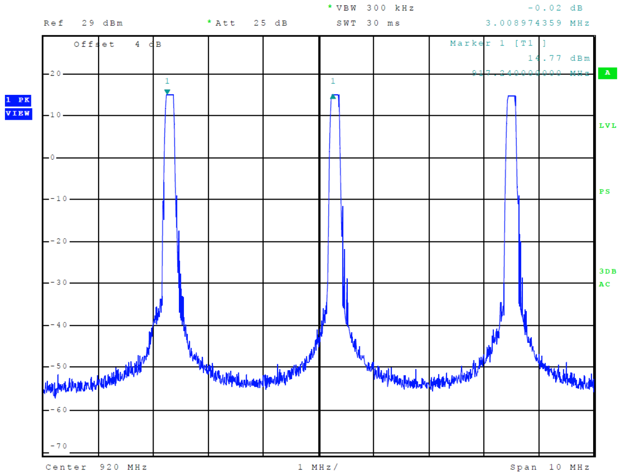
Figure 12 Plot of Channel Separation (P-mode)
