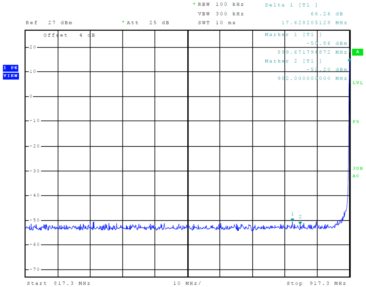
Figure 6 Plot of Lower Band Edge (P-mode)
