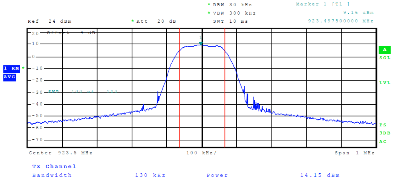
Figure 15 Plot of Output Power (P-Mode)
