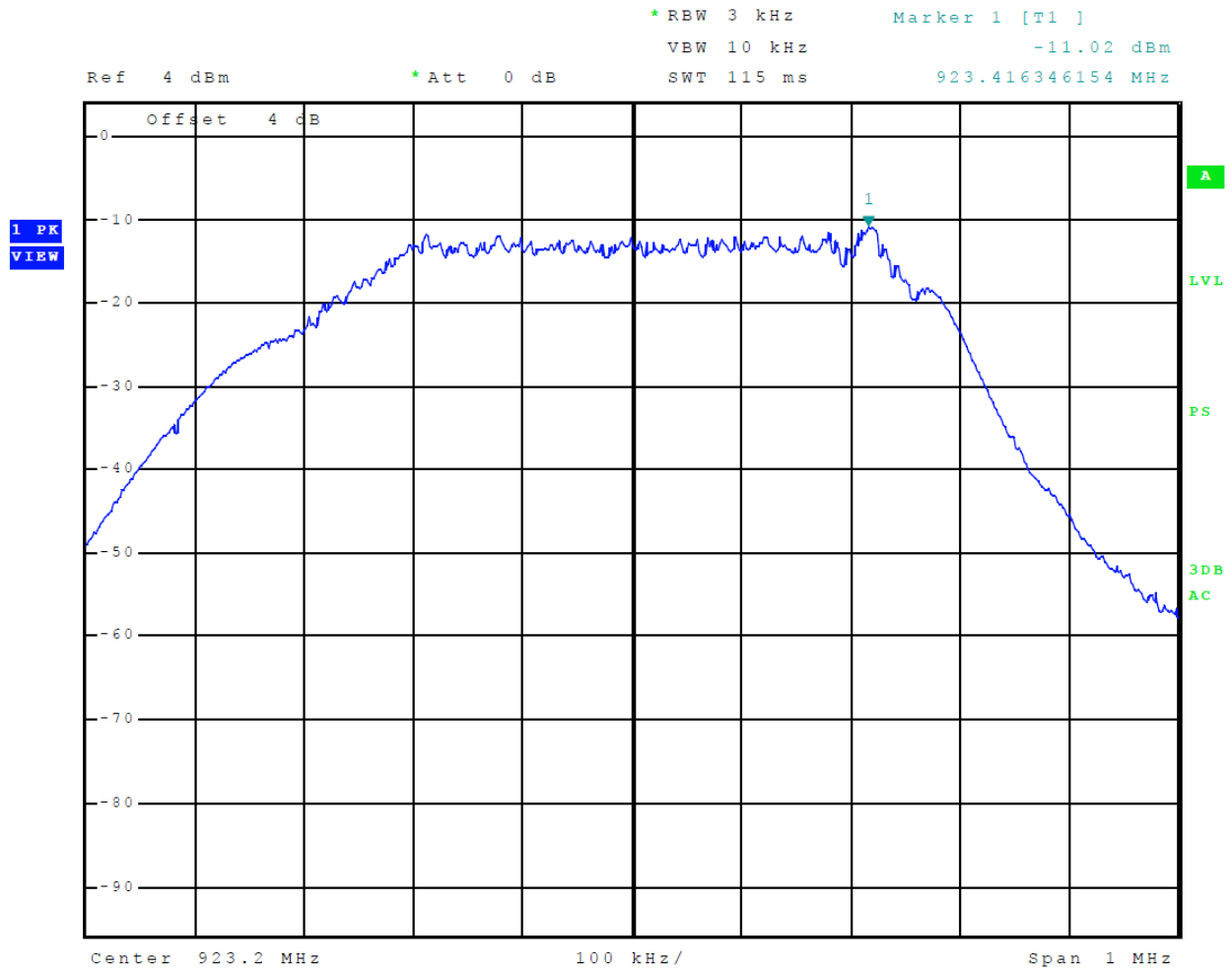
Figure 4 Plot of Power Spectral Density (Pairing)
