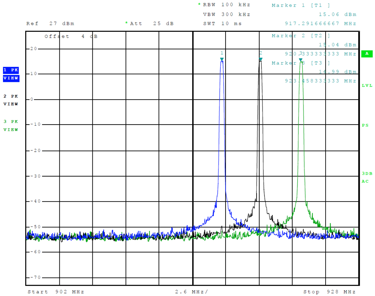
Figure 5 Plot of Transmitter Emissions in Operational Frequency Band (P-Mode)
