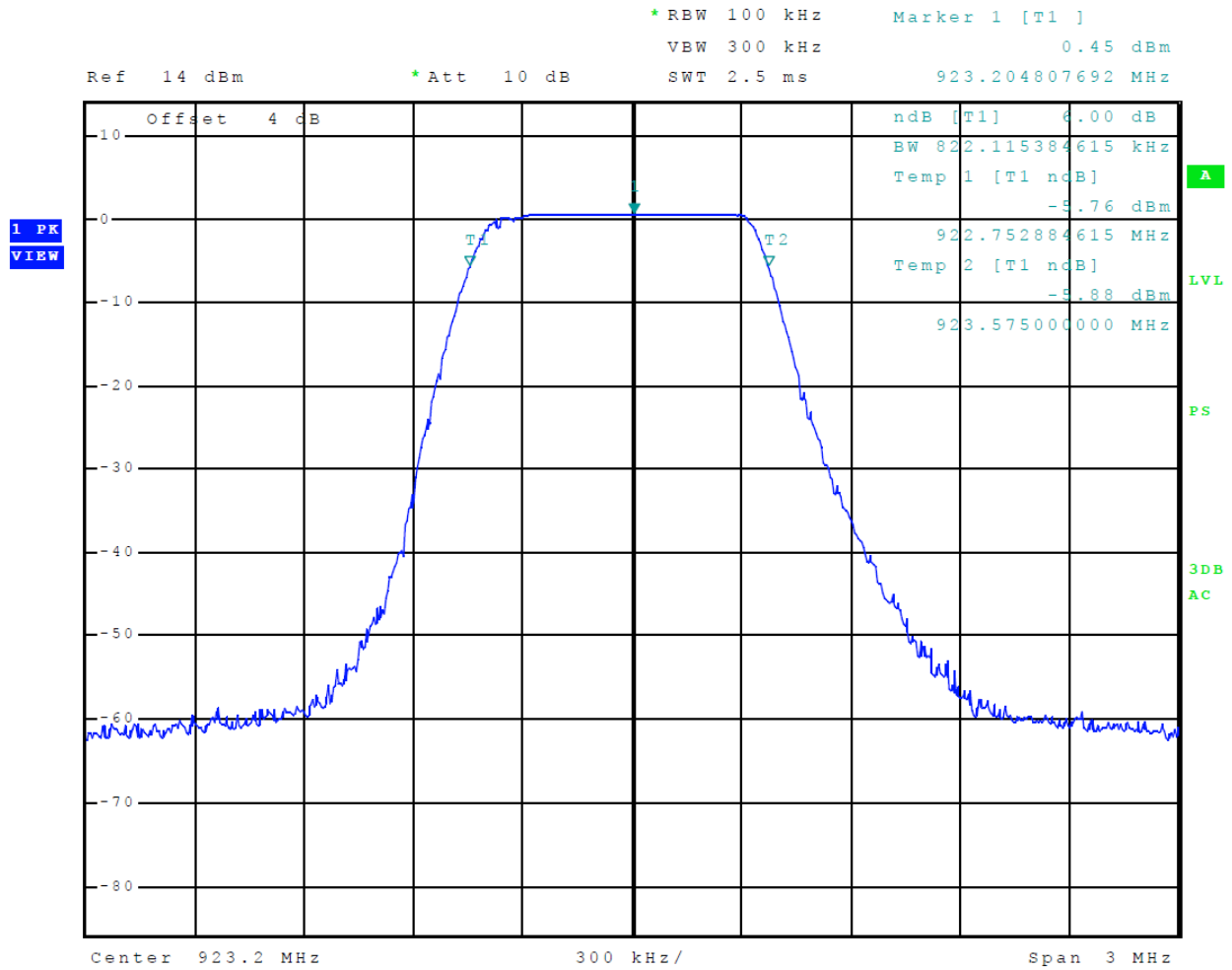
Figure 2 Plot of Transmitter 6-dB Occupied Bandwidth (Pairing)
