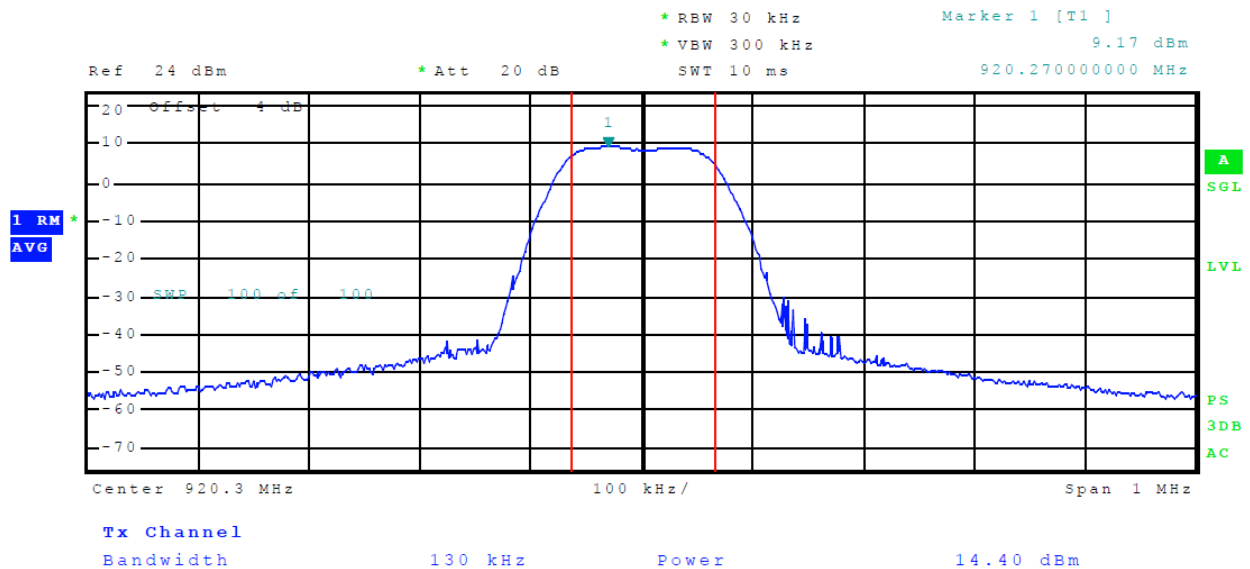
Figure 14 Plot of Output Power (P-Mode)
