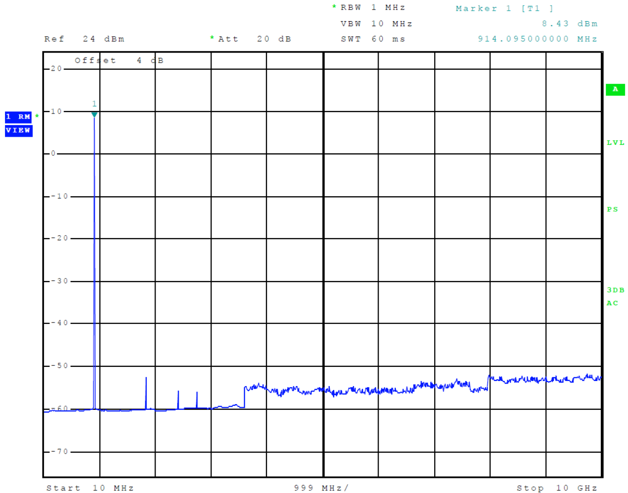
Figure 16 Plot of Out of Band Emissions
