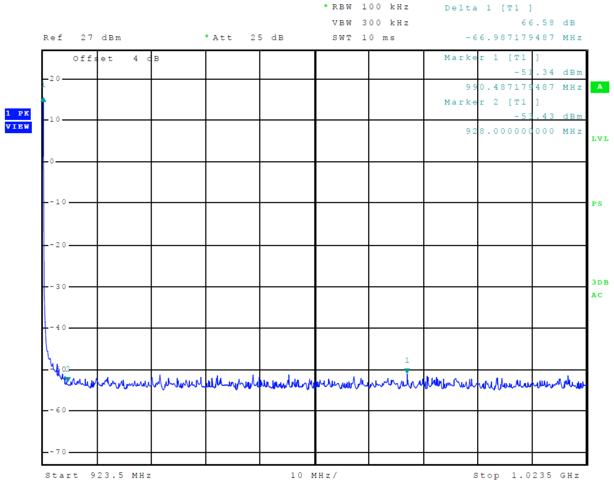
Figure 7 Plot of Upper Band Edge (P-mode)
