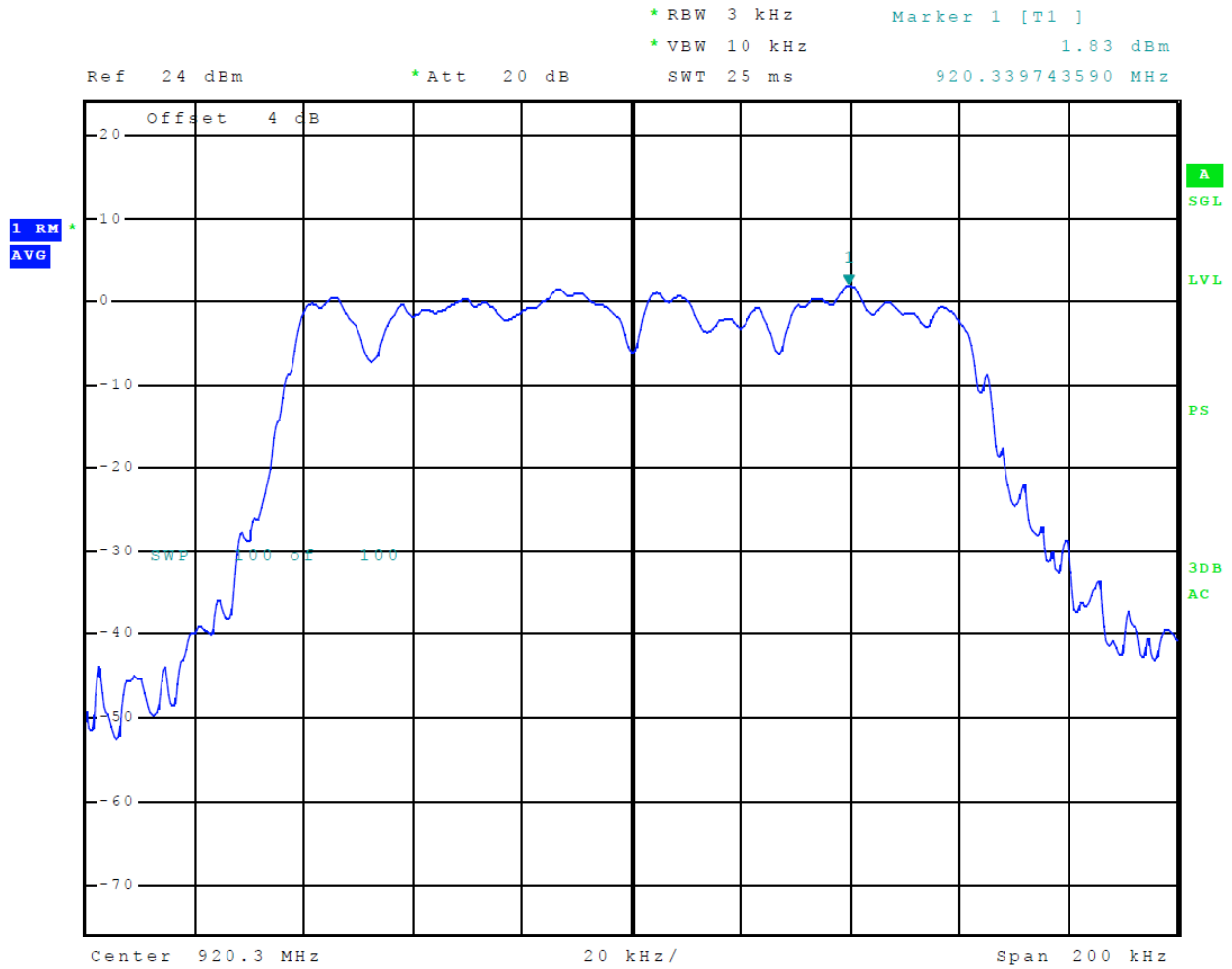
Figure 10 Plot of Power Spectral Density (P-Mode)
