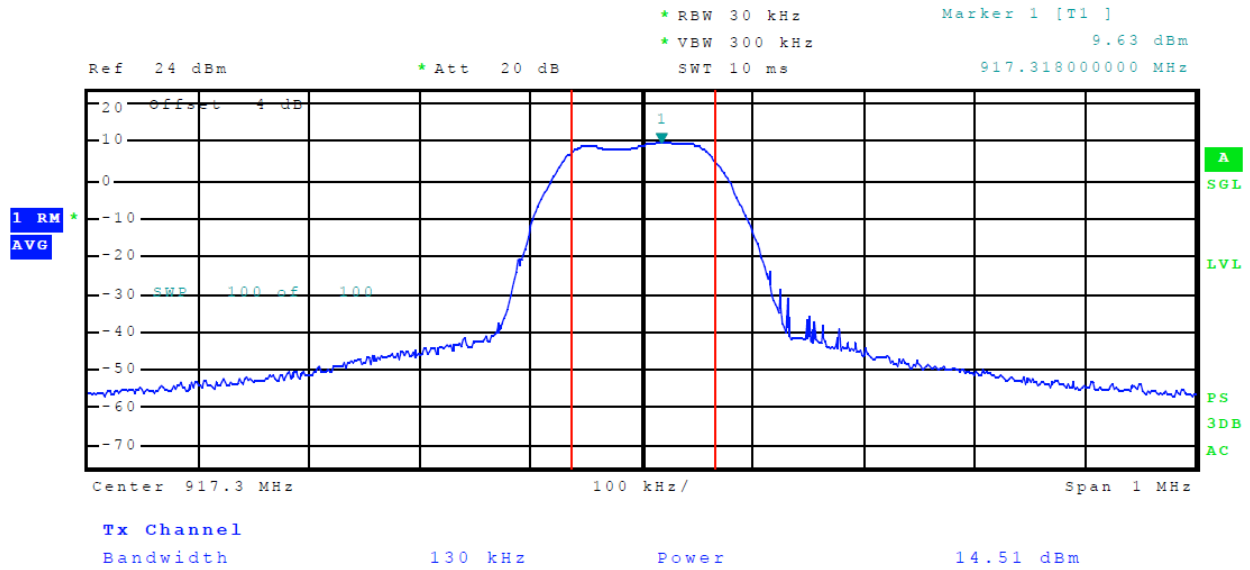
Figure 13 Plot of Output Power (P-Mode)
