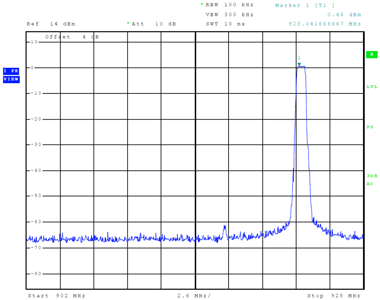
Figure 1 Plot of Transmitter Emissions in Operational Frequency Band (Pairing)
