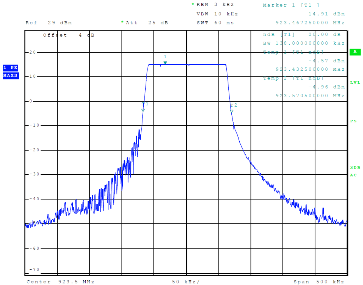
Figure 8 Plot of Transmitter 20-dB Occupied Bandwidth (P-mode)
