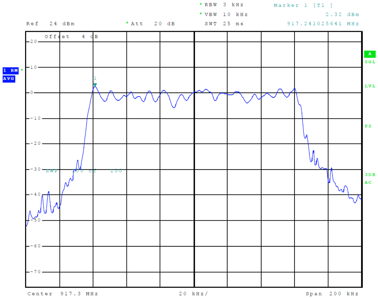
Figure 9 Plot of Power Spectral Density (P-Mode)
