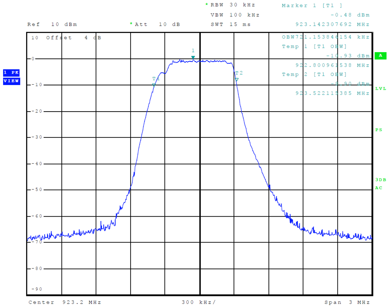
Figure 3 Plot of Transmitter 99% Occupied Bandwidth (Pairing)
