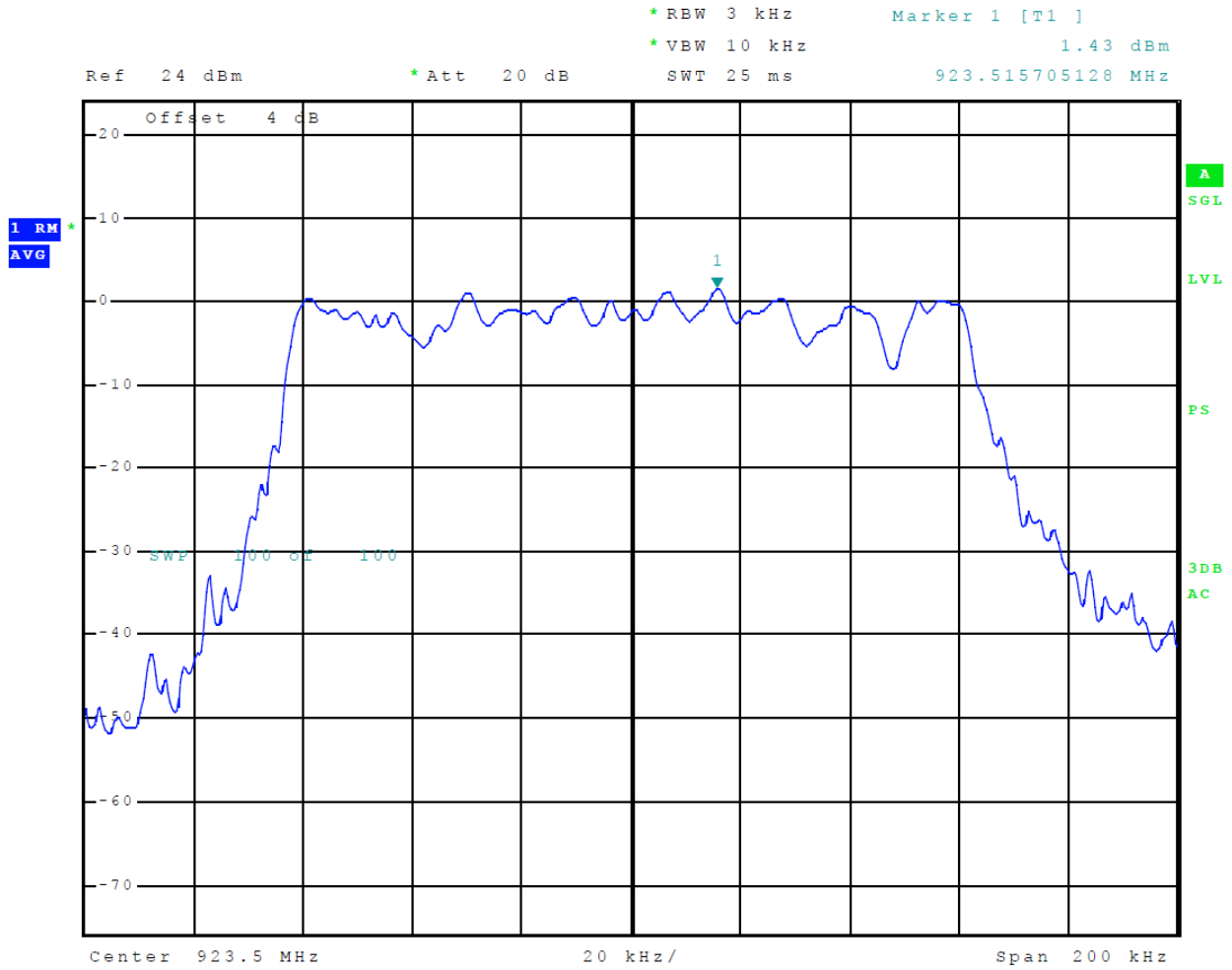
Figure 11 Plot of Power Spectral Density (P-Mode)
