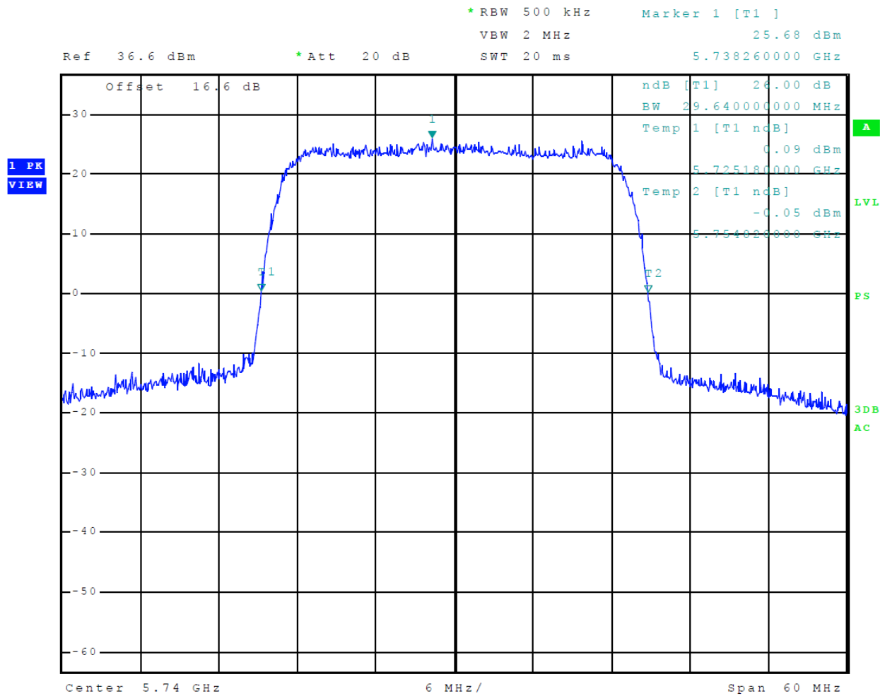
Figure 32 Plot of 26-dB OBW (30 MHz Channel)
