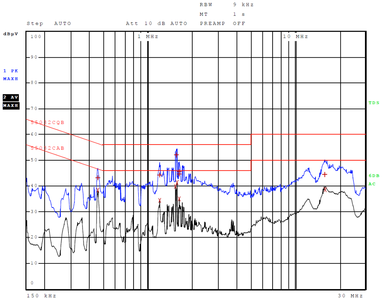
Figure 33 Plot of AC Line Conducted Emissions Line 1
