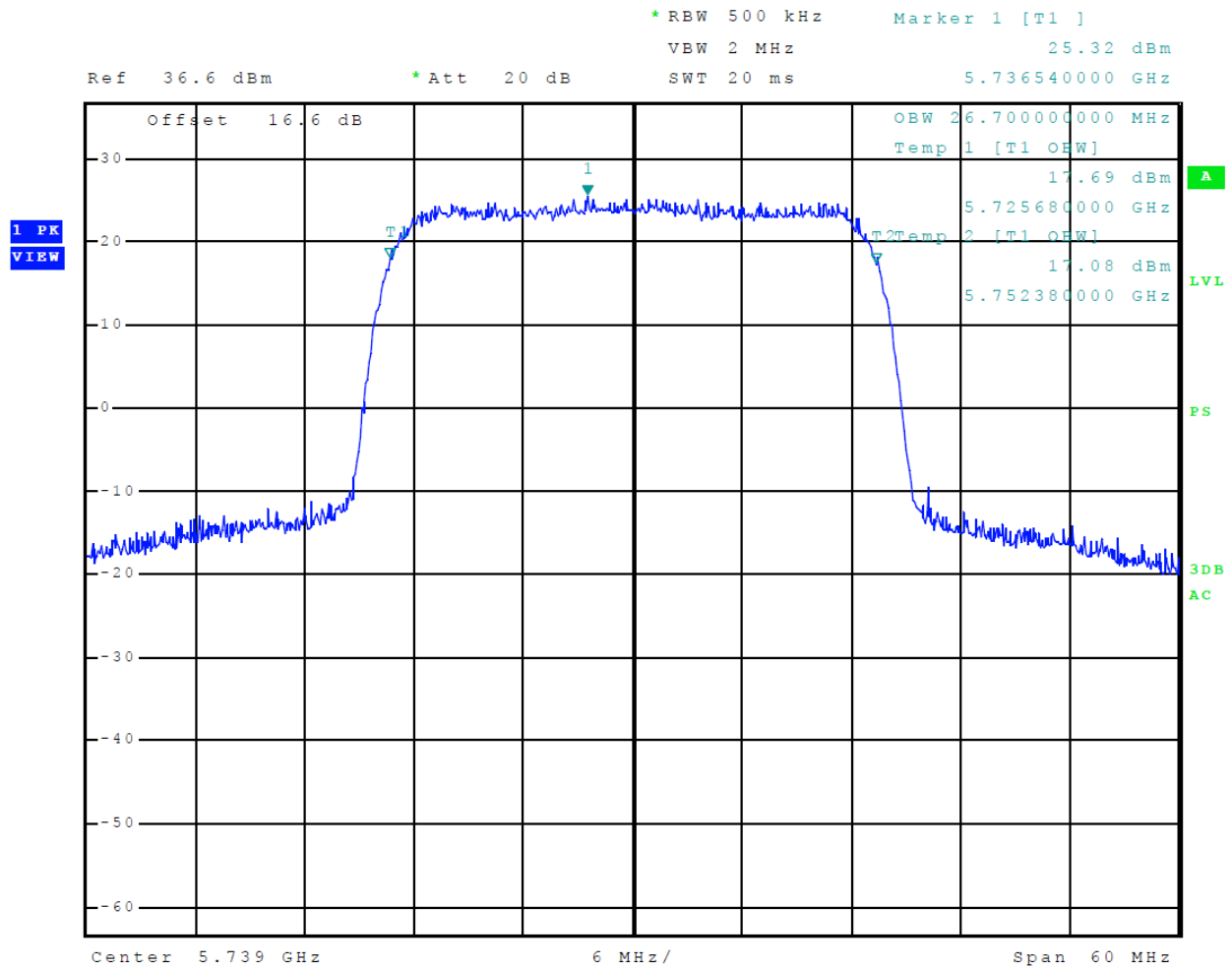
Figure 28 Plot of 99% OBW (28 MHz Channel)
