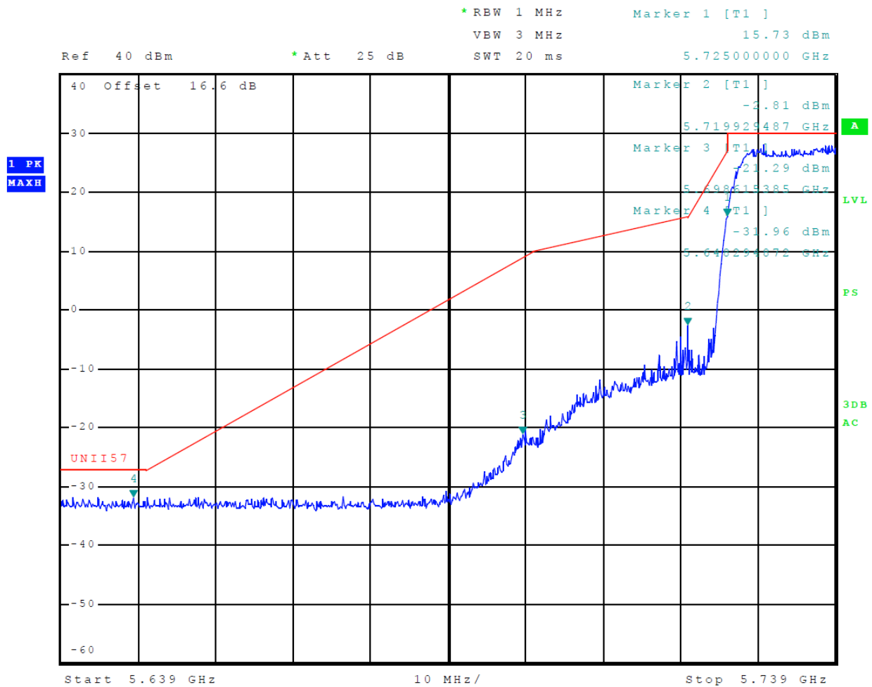
Figure 23 Plot of Undesirable emissions (28 MHz Channel)
