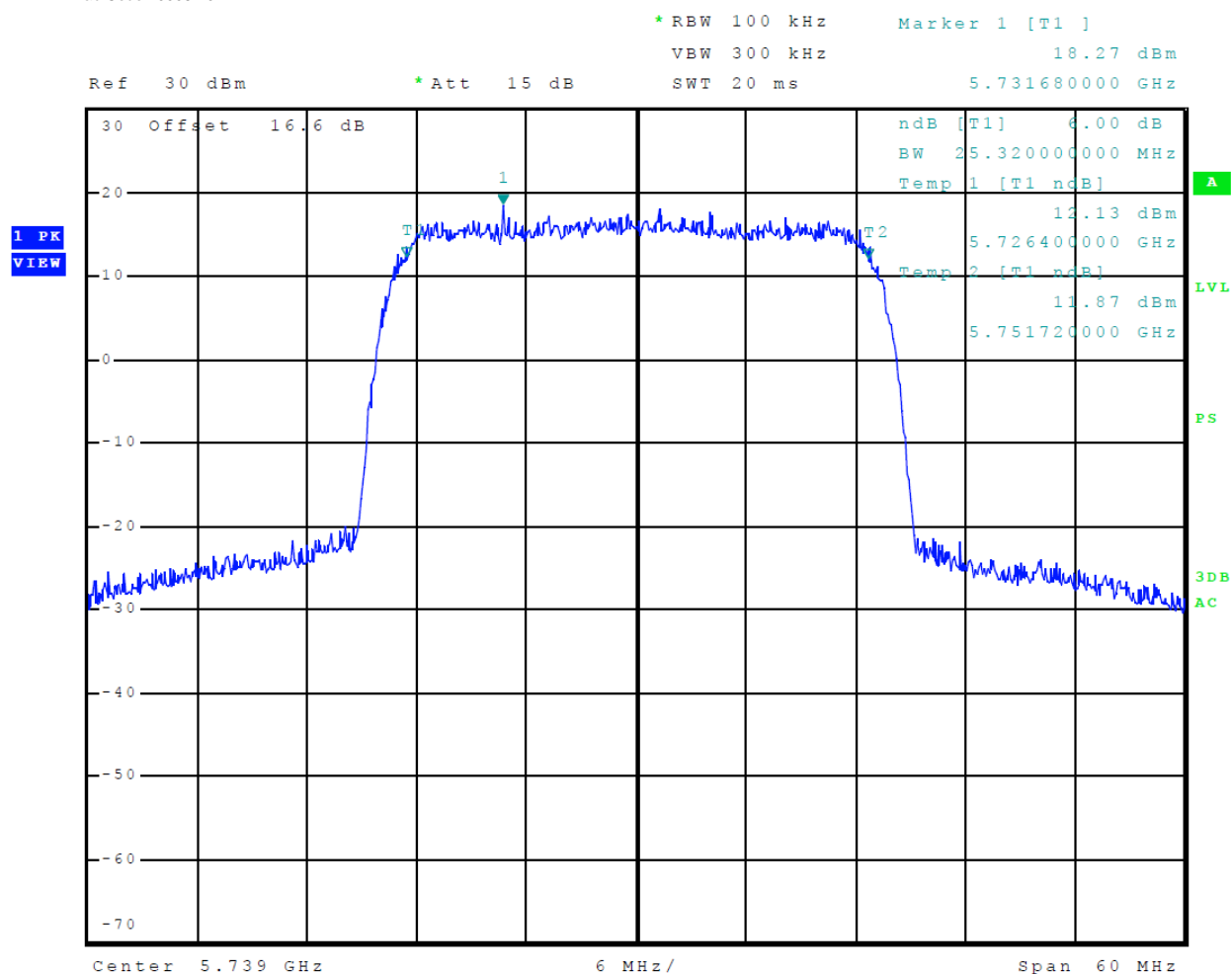
Figure 27 Plot of Minimum 6-dB Bandwidth (28 MHz Channel)
