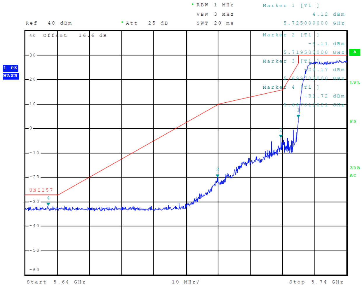
Figure 24 Plot of Undesirable emissions (30 MHz Channel)
