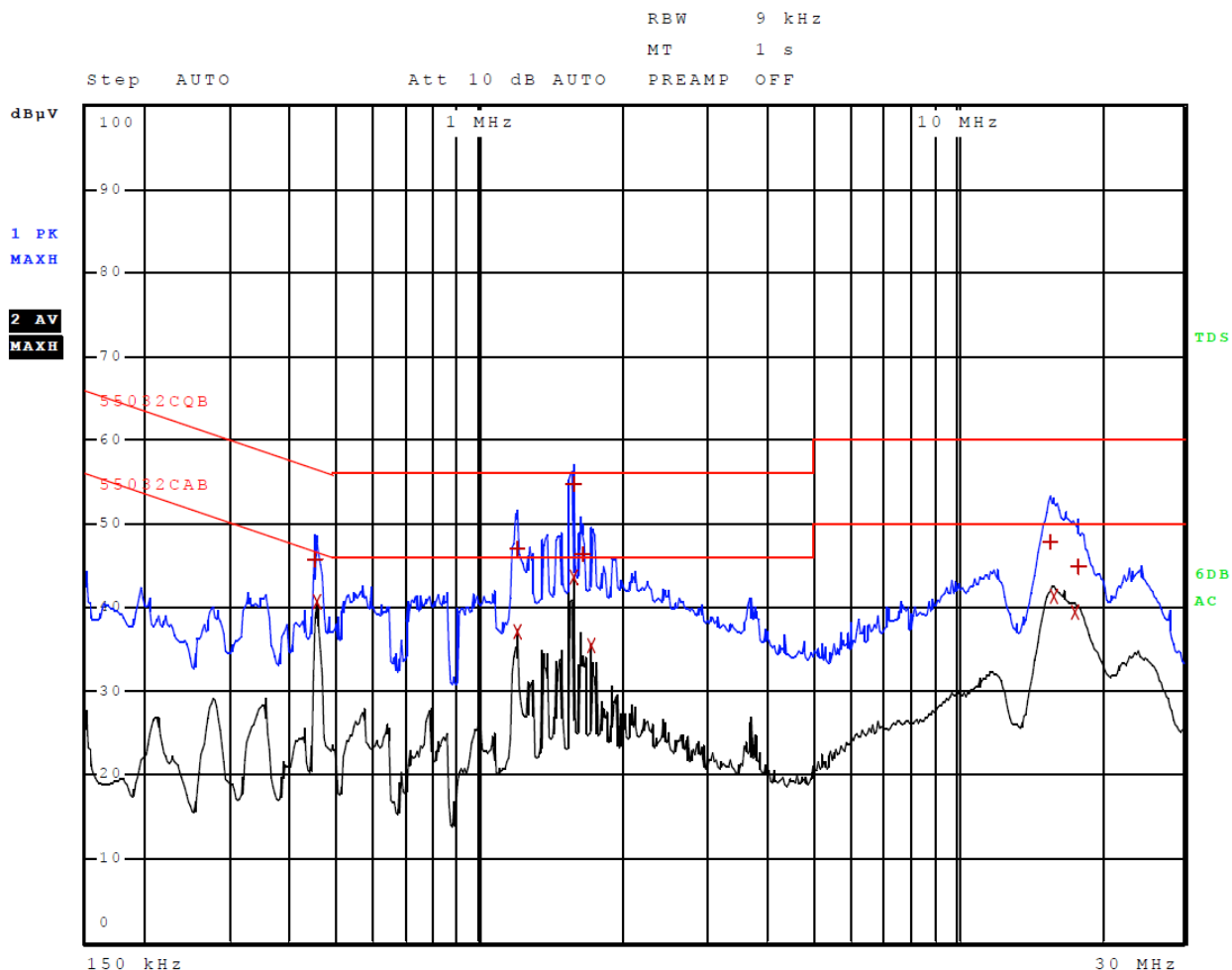
Figure 34 Plot of AC Line Conducted Emissions Line 2
