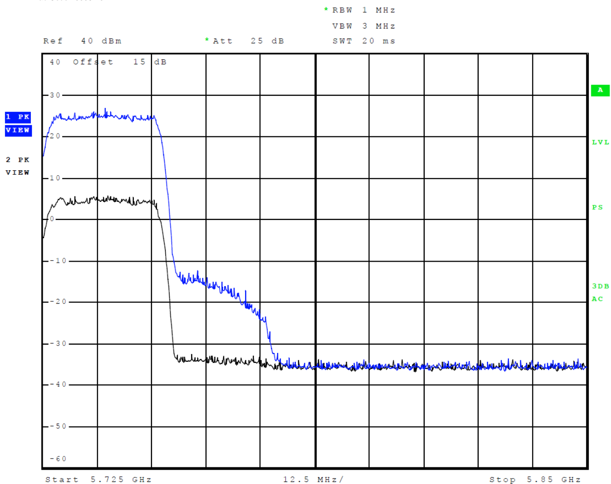
Figure 11 Plot of Transmitter Operation in Band (28 MHz Channel) power levels
