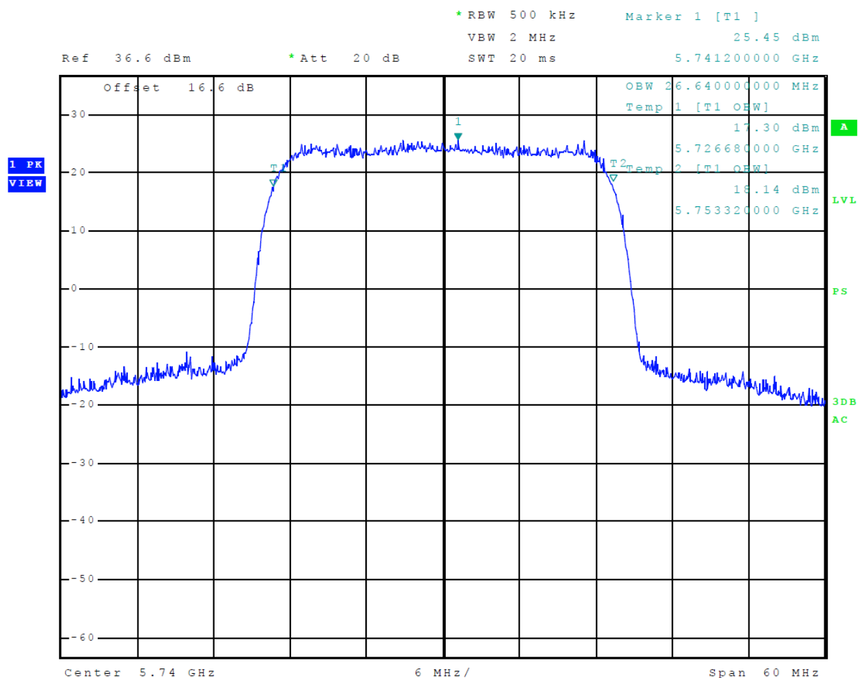
Figure 31 Plot of Transmitter 99% OBW (30 MHz Channel)
