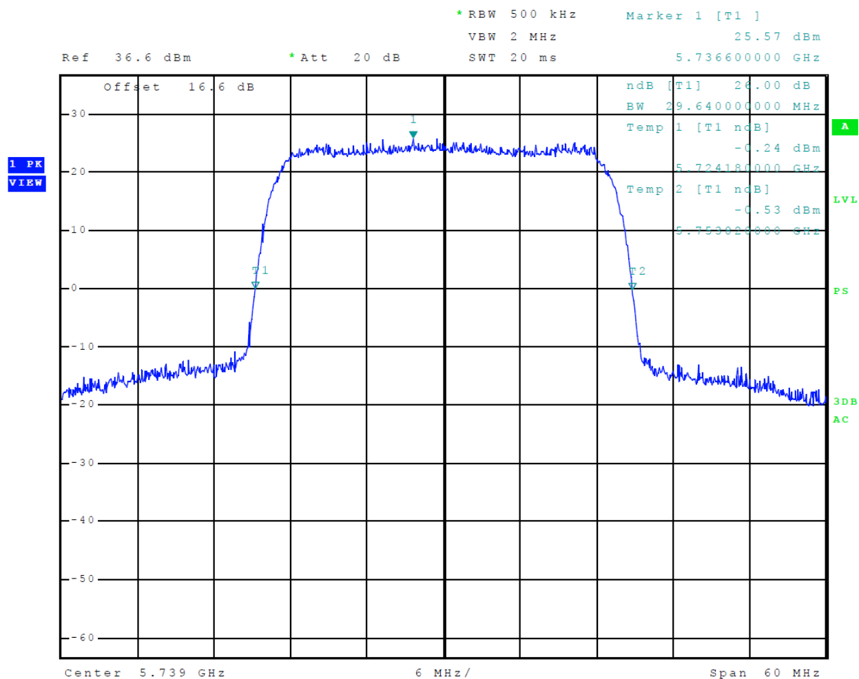
Figure 29 Plot of 26-dB OBW (28 MHz Channel)
