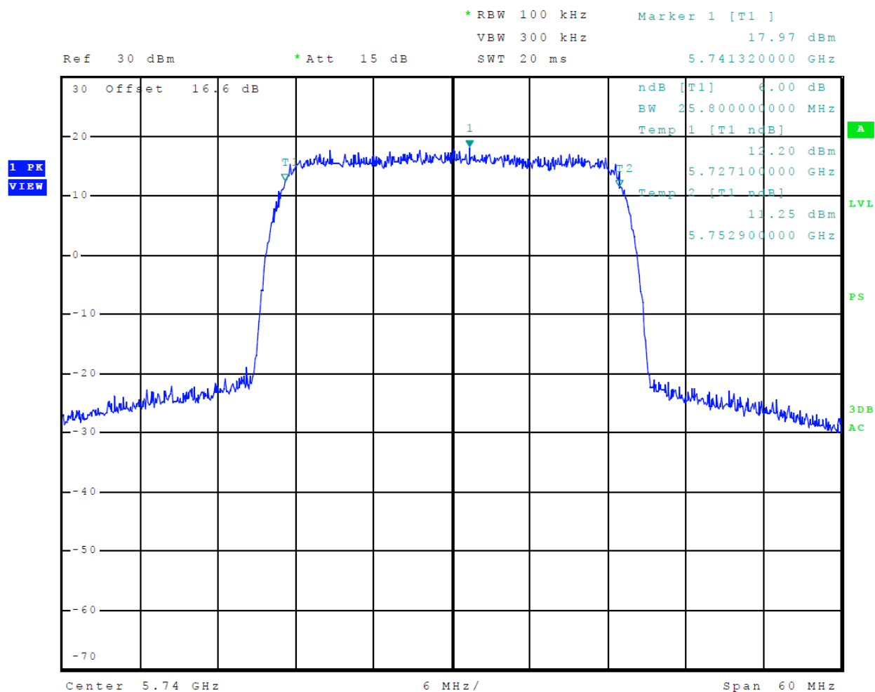
Figure 30 Plot of Minimum 6-dB Bandwidth (30 MHz Channel)
