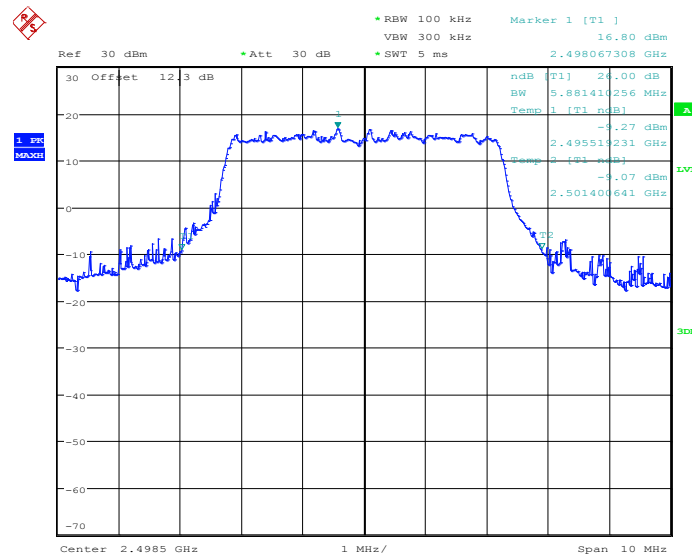
26dB Bandwidth Plot on Channel 39675
