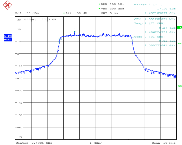
99% Occupied Bandwidth Plot on Channel 39675
