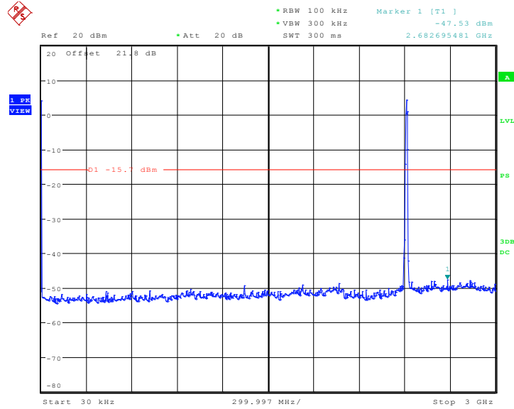
Conducted Spurious Emission Plot between 30kHz ~ 3 GHz
