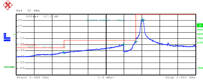
Lower Band Edge Plot for QPSK-RB Size 1, RB Offset 0
