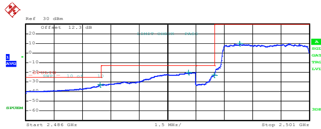
Lower Band Edge Plot for QPSK-RB Size 25, RB Offset 0
