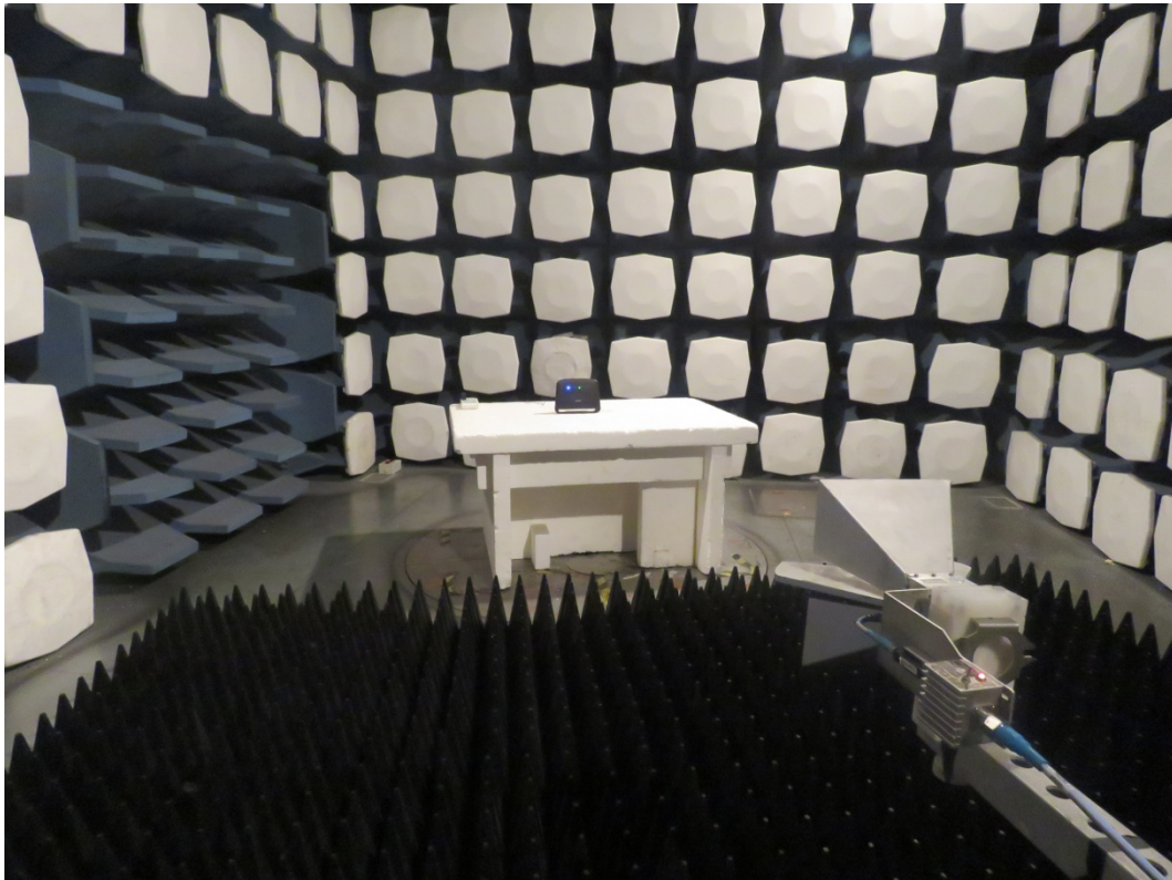
Above 1GHz Radiated Emission Test Setup
