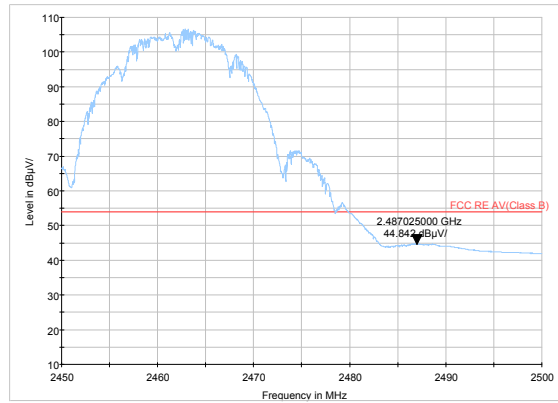
802.11b-Channel 11 Average
