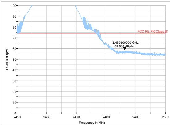
802.11b-Channel 11 Peak
