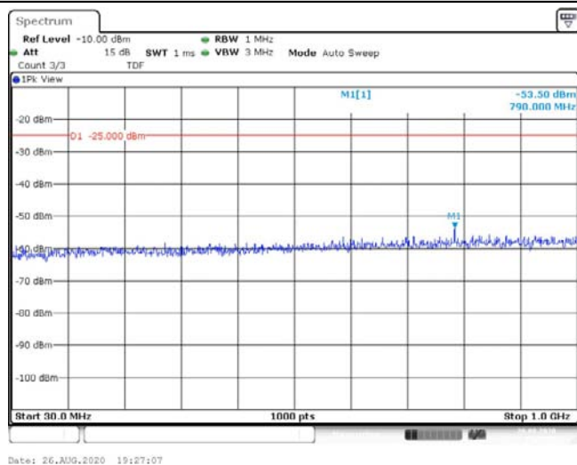
Band41-20MHz-QPSK-39750-1RB#0-Range1:30~1000MHz--53.5-PASS
