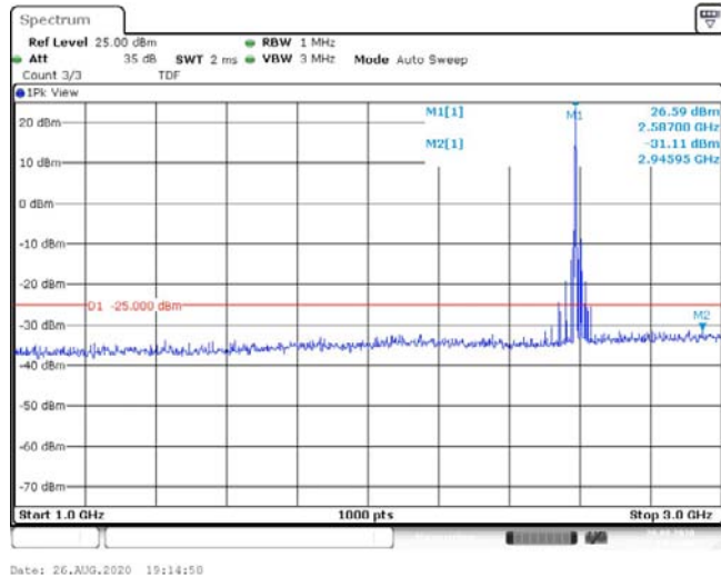
Band41-15MHz-16QAM-40620-1RB#0-Range2:1000~3000MHz--31.11-PASS
