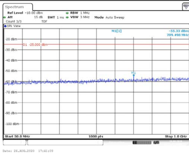
Band41-5MHz-QPSK-41565-1RB#0-Range1:30~1000MHz--55.33-PASS
