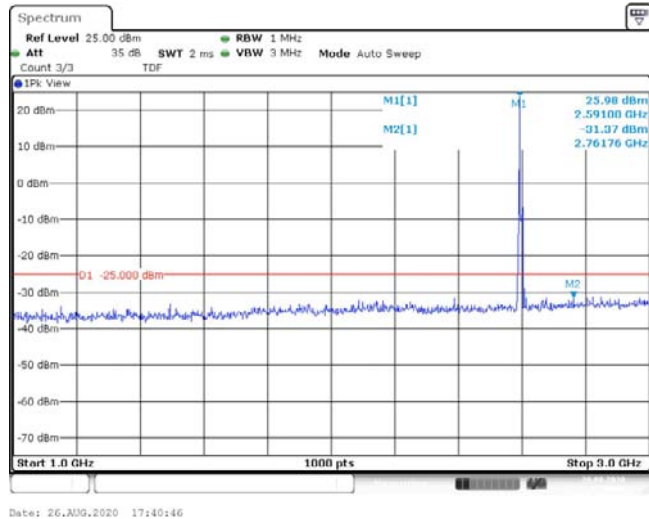
Band41-5MHz-16QAM-40620-1RB#0-Range2:1000~3000MHz--31.37-PASS
