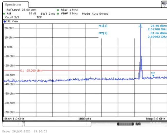
Band41-15MHz-16QAM-41515-1RB#0-Range2:1000~3000MHz--31.56-PASS
