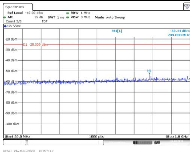
Band41-10MHz-16QAM-39700-1RB#0-Range1:30~1000MHz--53.44-PASS
