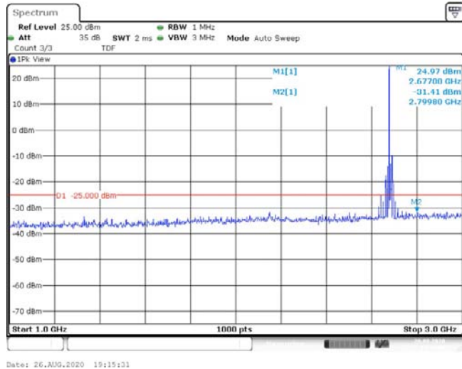
Band41-15MHz-QPSK-41515-1RB#0-Range2:1000~3000MHz--31.41-PASS
