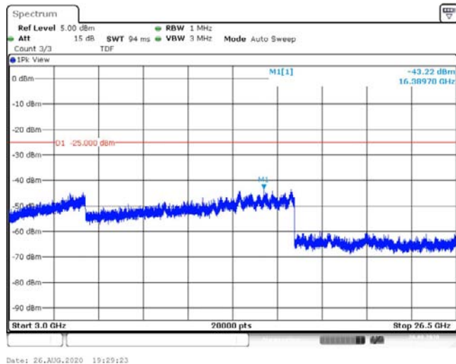
Band41-20MHz-16QAM-40620-1RB#0-Range3:3000~26500MHz--43.22-PASS
