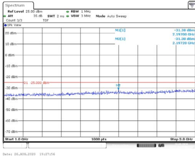
Band41-20MHz-16QAM-39750-1RB#0-Range2:1000~3000MHz--31.38-PASS
