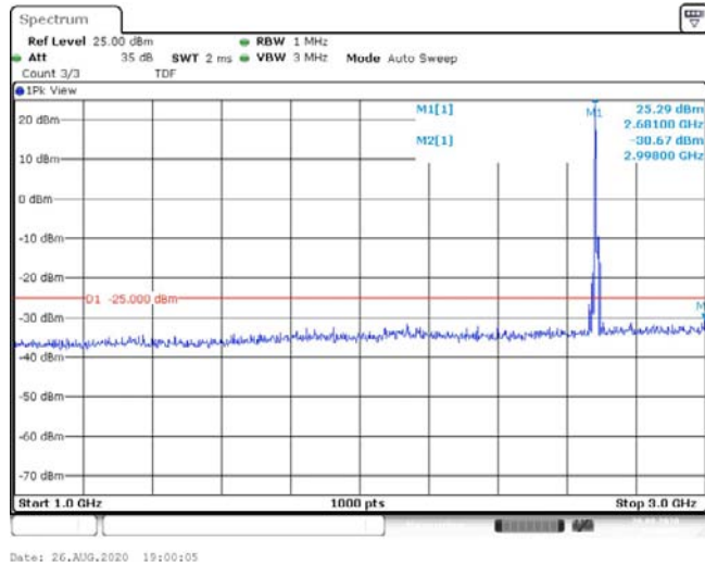
Band41-10MHz-16QAM-41540-1RB#0-Range2:1000~3000MHz--30.67-PASS
