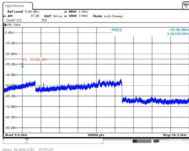
Band41-10MHz-QPSK-41540-1RB#0-Range3:3000~26500MHz--33.56-PASS
