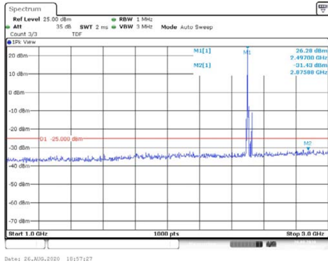
Band41-10MHz-16QAM-39700-1RB#0-Range2:1000~3000MHz--31.43-PASS
