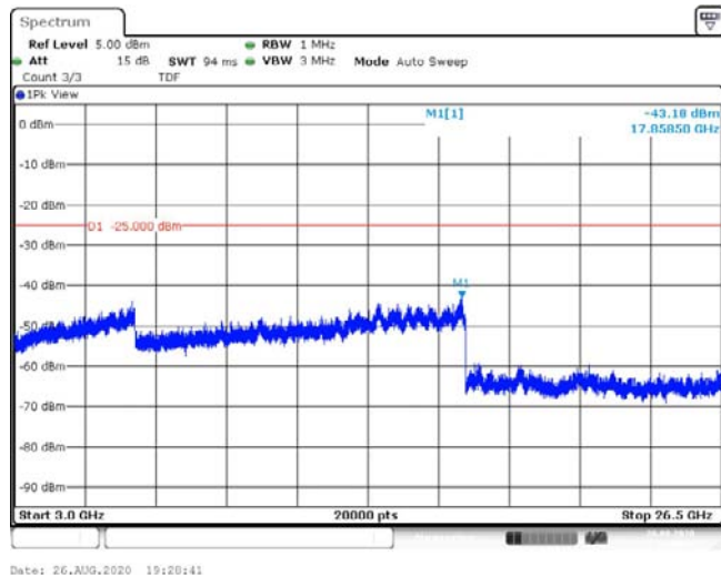
Band41-20MHz-QPSK-40620-1RB#0-Range3:3000~26500MHz--43.18-PASS
