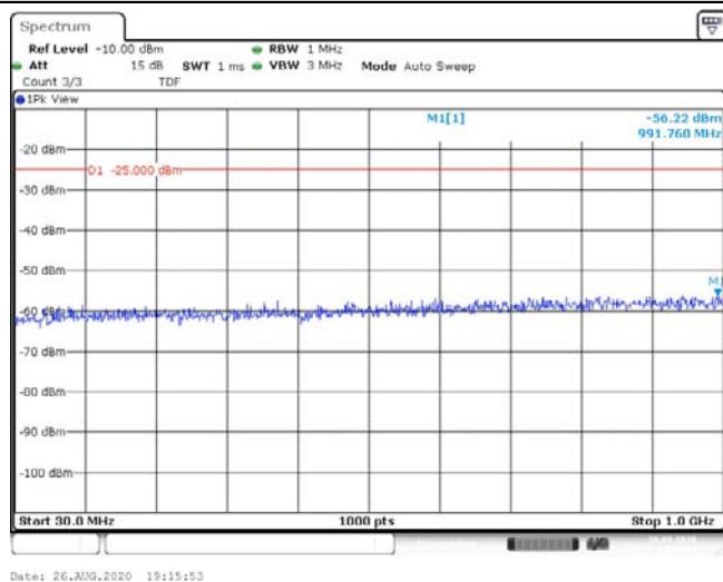
Band41-15MHz-16QAM-41515-1RB#0-Range1:30~1000MHz--56.22-PASS
