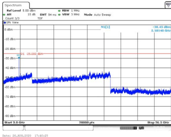
Band41-5MHz-QPSK-40620-1RB#0-Range3:3000~26500MHz--30.45-PASS
