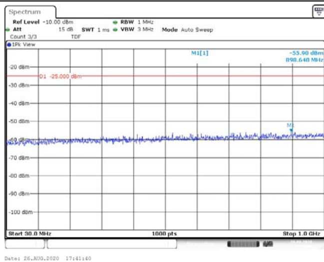
Band41-5MHz-16QAM-41565-1RB#0-Range1:30~1000MHz--55.9-PASS
