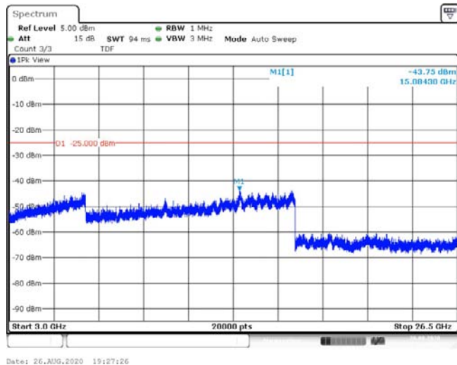
Band41-20MHz-QPSK-39750-1RB#0-Range3:3000~26500MHz--43.75-PASS
