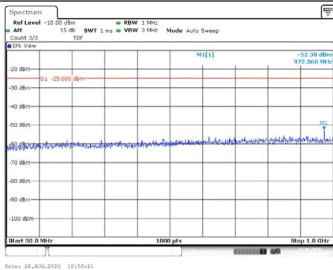
Band41-10MHz-16QAM-40620-1RB#0-Range1:30~1000MHz--52.38-PASS
