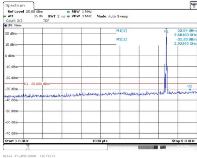
Band41-10MHz-QPSK-41540-1RB#0-Range2:1000~3000MHz--31.53-PASS
