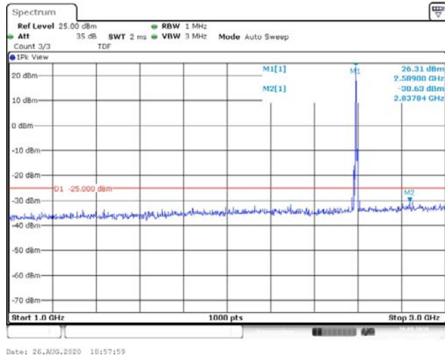
Band41-10MHz-QPSK-40620-1RB#0-Range2:1000~3000MHz--30.63-PASS
