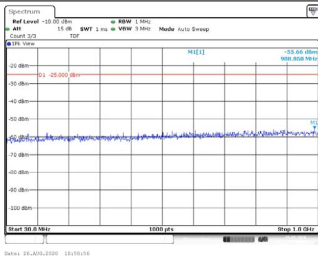
Band41-10MHz-QPSK-41540-1RB#0-Range1:30~1000MHz--55.66-PASS
