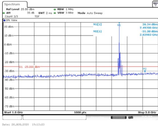
Band41-15MHz-QPSK-39725-1RB#0-Range2:1000~3000MHz--31.3-PASS
