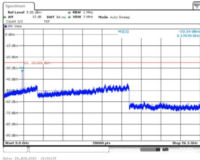
Band41-10MHz-QPSK-40620-1RB#0-Range3:3000~26500MHz--33.54-PASS
