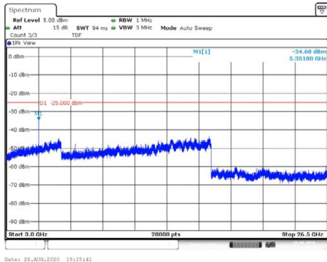
Band41-15MHz-QPSK-41515-1RB#0-Range3:3000~26500MHz--34.68-PASS
