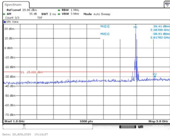
Band41-15MHz-QPSK-40620-1RB#0-Range2:1000~3000MHz--30.91-PASS
