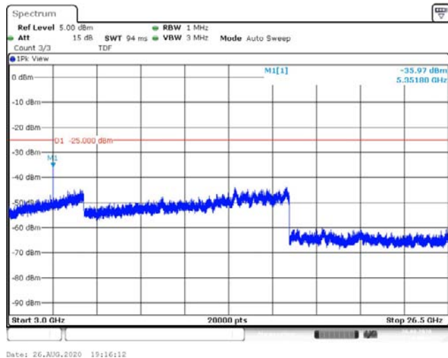
Band41-15MHz-16QAM-41515-1RB#0-Range3:3000~26500MHz--35.97-PASS
