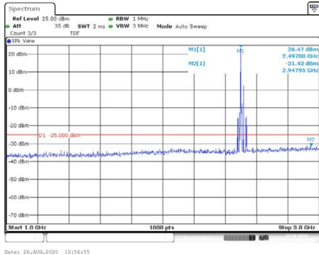
Band41-10MHz-QPSK-39700-1RB#0-Range2:1000~3000MHz--31.43-PASS
