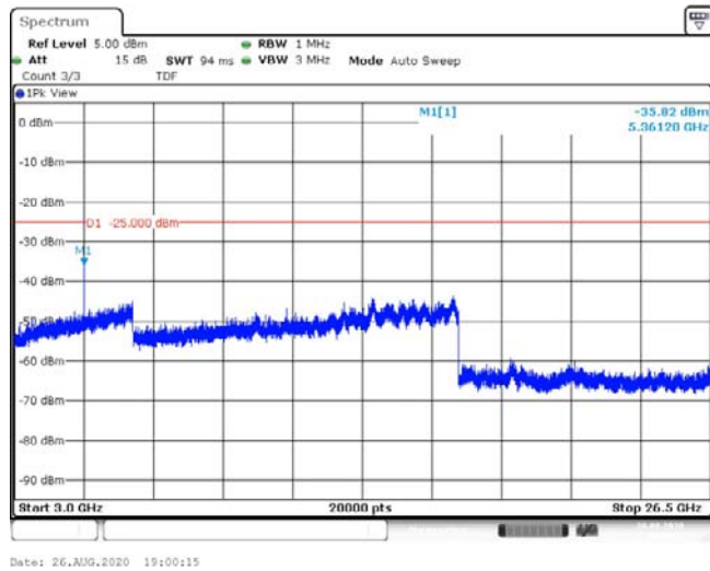
Band41-10MHz-16QAM-41540-1RB#0-Range3:3000~26500MHz--35.82-PASS
