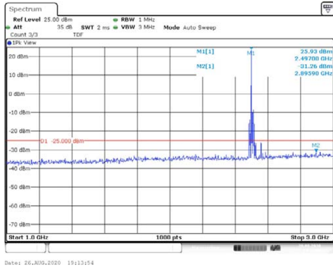
Band41-15MHz-16QAM-39725-1RB#0-Range2:1000~3000MHz--31.26-PASS
