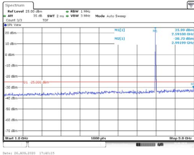
Band41-5MHz-QPSK-40620-1RB#0-Range2:1000~3000MHz--30.73-PASS
