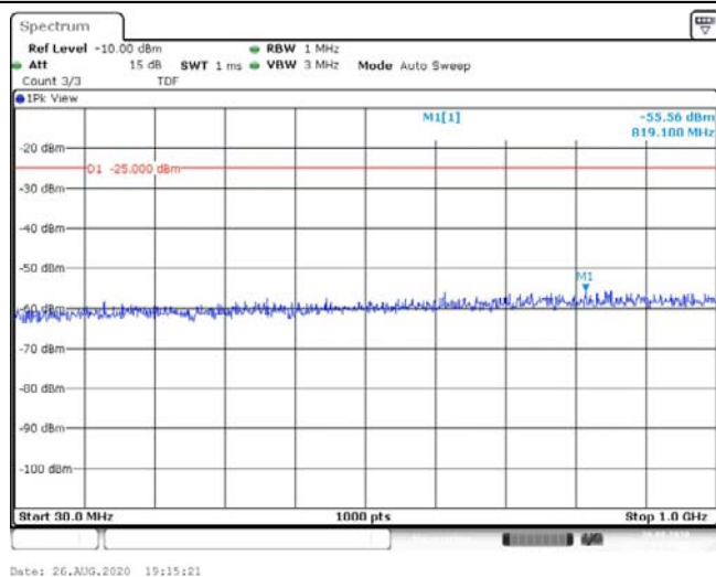
Band41-15MHz-QPSK-41515-1RB#0-Range1:30~1000MHz--55.56-PASS
