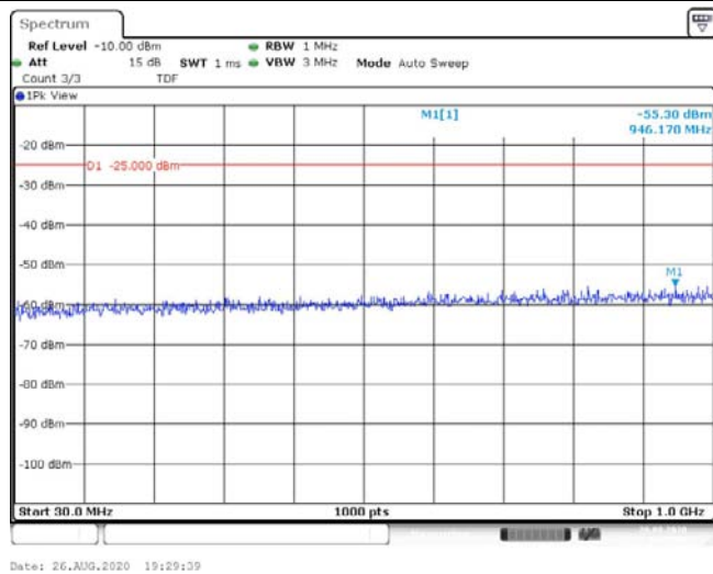
Band41-20MHz-QPSK-41490-1RB#0-Range1:30~1000MHz--55.3-PASS
