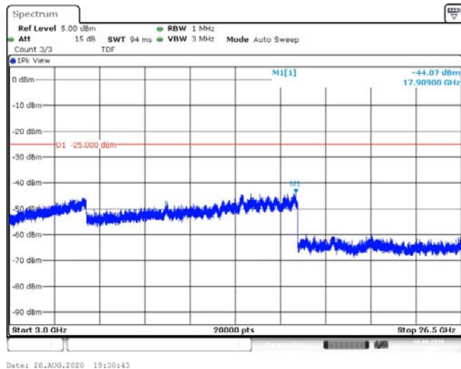
Band41-20MHz-16QAM-41490-1RB#0-Range3:3000~26500MHz--44.07-PASS
