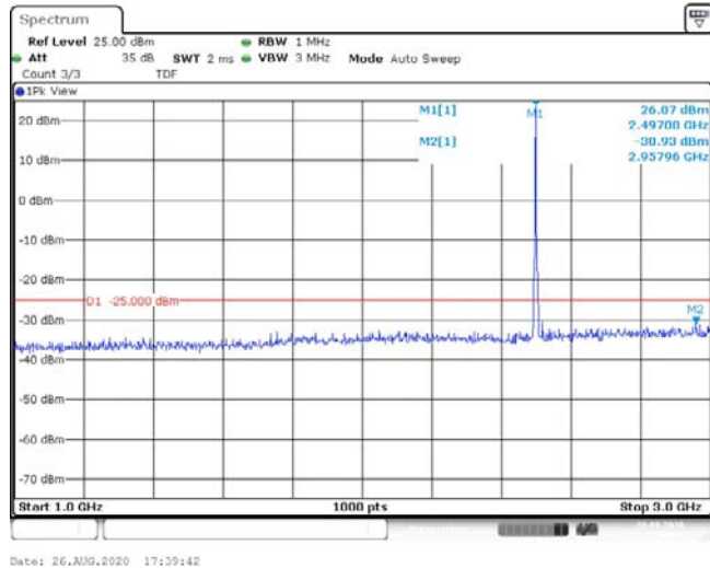
Band41-5MHz-16QAM-39675-1RB#0-Range2:1000~3000MHz--30.93-PASS
