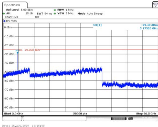
Band41-15MHz-16QAM-40620-1RB#0-Range3:3000~26500MHz--29.49-PASS
