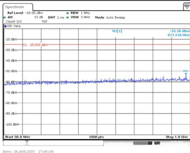
Band41-5MHz-QPSK-40620-1RB#0-Range1:30~1000MHz--53.58-PASS
