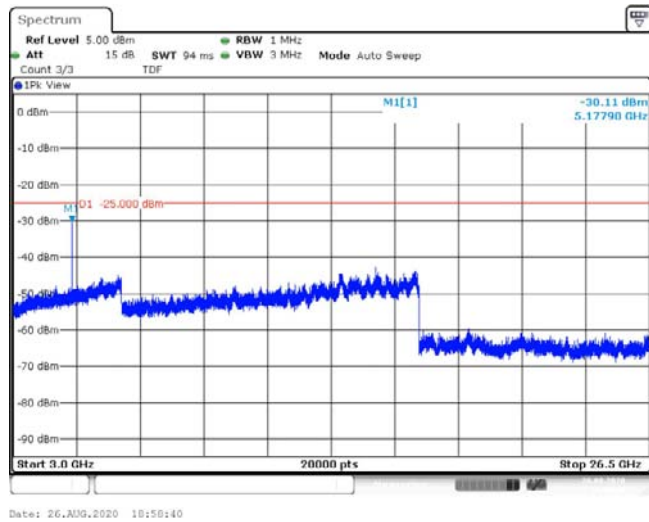
Band41-10MHz-16QAM-40620-1RB#0-Range3:3000~26500MHz--30.11-PASS
