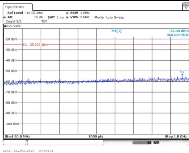
Band41-20MHz-16QAM-40620-1RB#0-Range1:30~1000MHz--54.45-PASS
