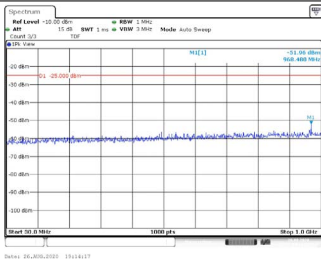
Band41-15MHz-QPSK-40620-1RB#0-Range1:30~1000MHz--51.96-PASS
