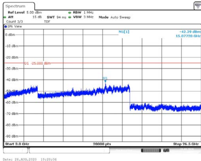
Band41-20MHz-16QAM-39750-1RB#0-Range3:3000~26500MHz--42.29-PASS
