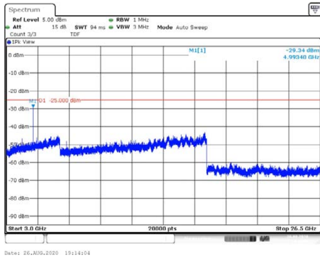
Band41-15MHz-16QAM-39725-1RB#0-Range3:3000~26500MHz--29.34-PASS
