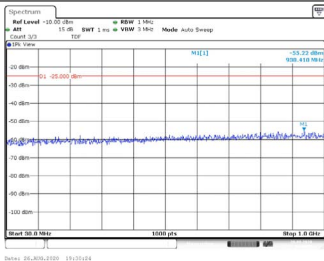
Band41-20MHz-16QAM-41490-1RB#0-Range1:30~1000MHz--55.22-PASS
