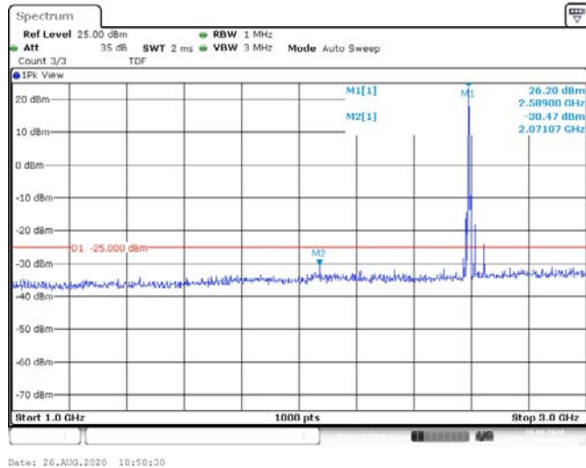
Band41-10MHz-16QAM-40620-1RB#0-Range2:1000~3000MHz--30.47-PASS
