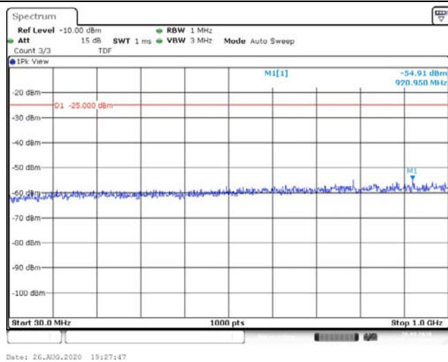
Band41-20MHz-16QAM-39750-1RB#0-Range1:30~1000MHz--54.91-PASS
