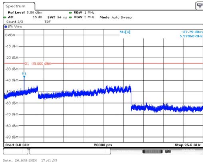
Band41-5MHz-16QAM-41565-1RB#0-Range3:3000~26500MHz--37.79-PASS
