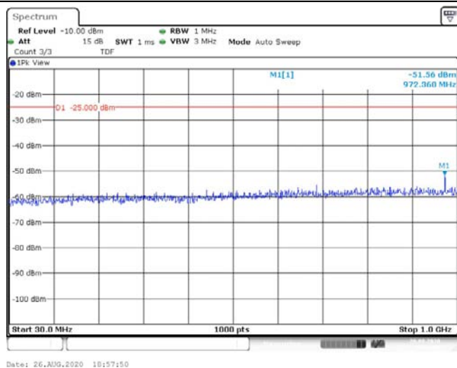
Band41-10MHz-QPSK-40620-1RB#0-Range1:30~1000MHz--51.56-PASS
