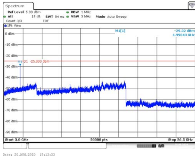
Band41-15MHz-QPSK-39725-1RB#0-Range3:3000~26500MHz--29.32-PASS
