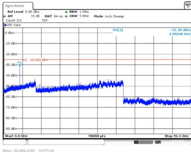
Band41-10MHz-16QAM-39700-1RB#0-Range3:3000~26500MHz--31.56-PASS
