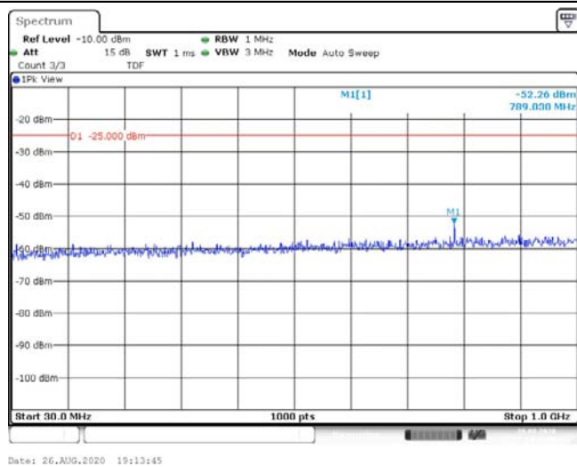
Band41-15MHz-16QAM-39725-1RB#0-Range1:30~1000MHz--52.26-PASS
