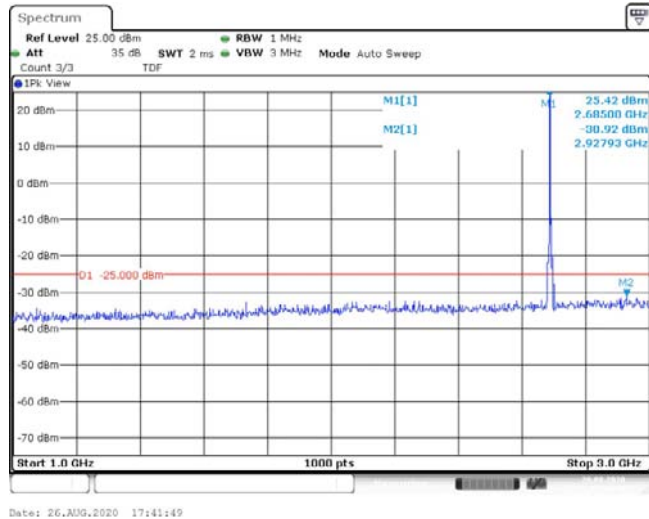
Band41-5MHz-16QAM-41565-1RB#0-Range2:1000~3000MHz--30.92-PASS
