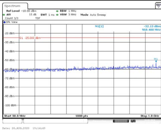
Band41-15MHz-16QAM-40620-1RB#0-Range1:30~1000MHz--52.13-PASS
