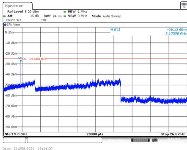
Band41-15MHz-QPSK-40620-1RB#0-Range3:3000~26500MHz--28.15-PASS
