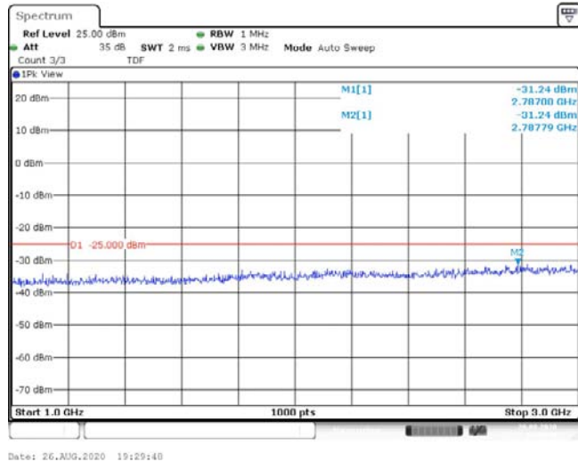
Band41-20MHz-QPSK-41490-1RB#0-Range2:1000~3000MHz--31.24-PASS
