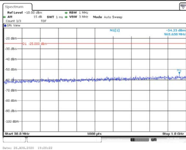
Band41-20MHz-QPSK-40620-1RB#0-Range1:30~1000MHz--54.25-PASS
