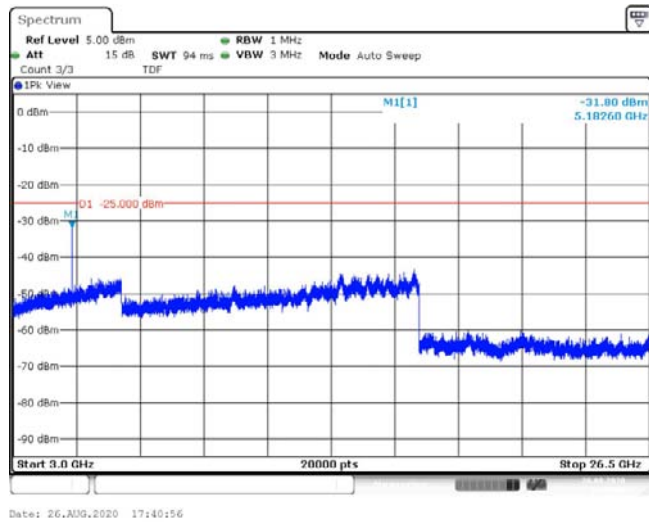
Band41-5MHz-16QAM-40620-1RB#0-Range3:3000~26500MHz--31.8-PASS
