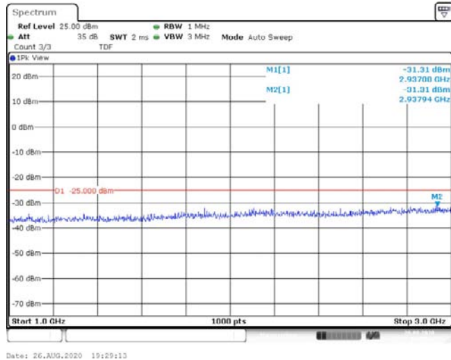
Band41-20MHz-16QAM-40620-1RB#0-Range2:1000~3000MHz--31.31-PASS
