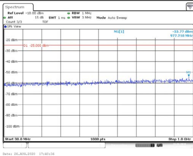
Band41-5MHz-16QAM-40620-1RB#0-Range1:30~1000MHz--53.77-PASS
