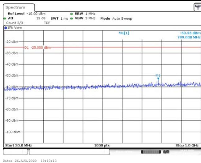
Band41-15MHz-QPSK-39725-1RB#0-Range1:30~1000MHz--53.55-PASS
