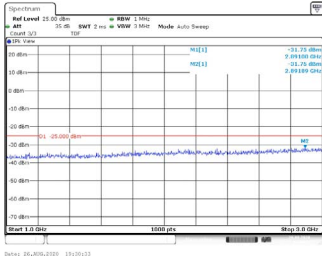
Band41-20MHz-16QAM-41490-1RB#0-Range2:1000~3000MHz--31.75-PASS
