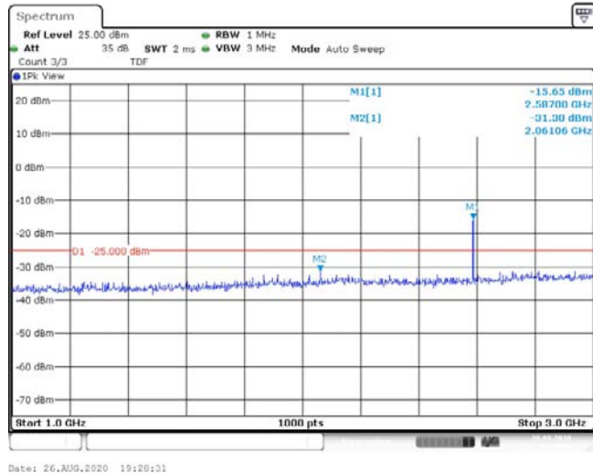
Band41-20MHz-QPSK-40620-1RB#0-Range2:1000~3000MHz--31.3-PASS
