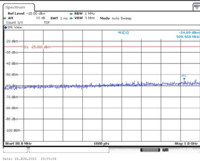
Band41-10MHz-16QAM-41540-1RB#0-Range1:30~1000MHz--54.69-PASS
