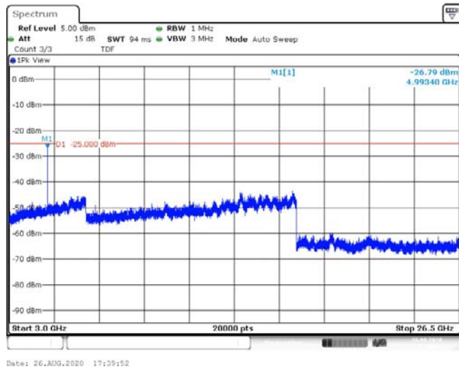
Band41-5MHz-16QAM-39675-1RB#0-Range3:3000~26500MHz--26.79-PASS
