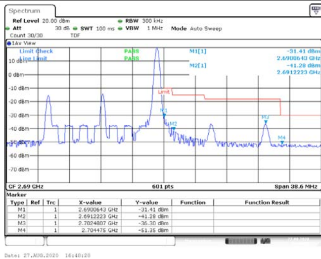
Band41-15MHz-16QAM-41515-1RB#74--31.41,-41.28,-36.30,-51.35-PASS
