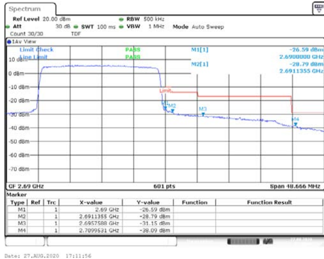
Band41-20MHz-QPSK-41490-100RB#0--26.59,-28.79,-31.15,-38.09-PASS
