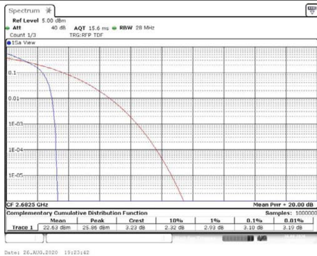
Band41-15MHz-16QAM-41515-1RB#0-3.10-13-PASS
