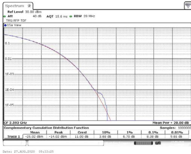
Band41-20MHz-16QAM-40620-100RB#0-8.38-13-PASS
