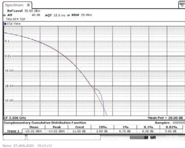
Band41-20MHz-16QAM-39750-1RB#0-8.38-13-PASS
