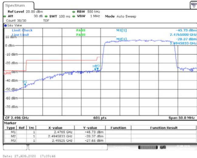
Band41-20MHz-16QAM-39750-100RB#0--45.73,-28.37,-27.65-PASS
