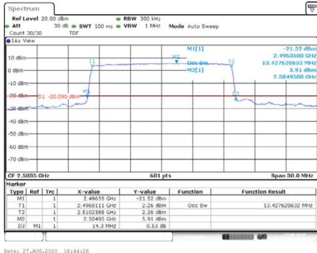
Band41-15MHz-16QAM-39725-75RB#0-13.428-14.300-PASS
