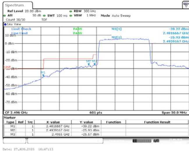
Band41-15MHz-16QAM-39725-75RB#0--39.22,-25.93,-25.57-PASS
