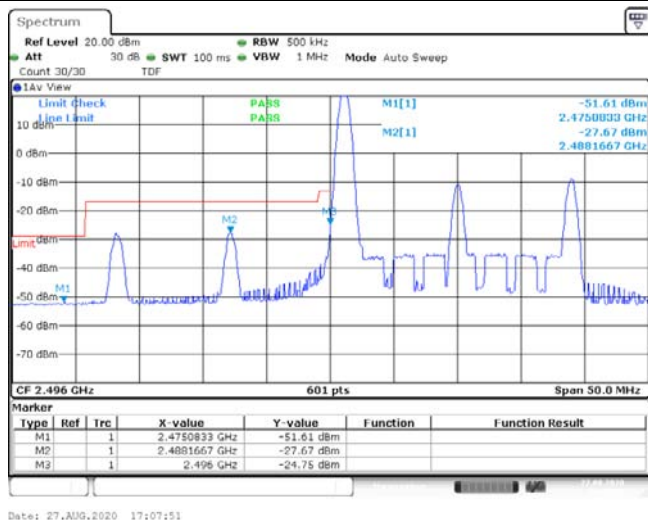
Band41-20MHz-QPSK-39750-1RB#0--51.61,-27.67,-24.75-PASS
