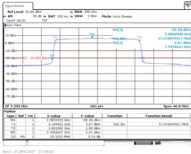
Band41-20MHz-16QAM-40620-100RB#0-17.97-19.333-PASS
