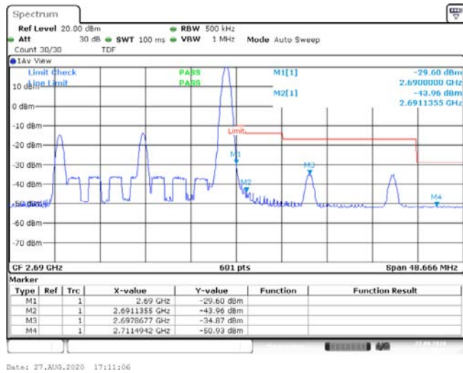
Band41-20MHz-QPSK-41490-1RB#99--29.60,-43.96,-34.87,-50.93-PASS
