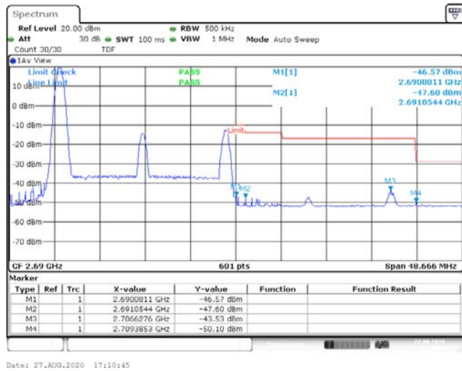
Band41-20MHz-16QAM-41490-1RB#0--46.57,-47.60,-43.53,-50.10-PASS
