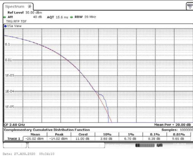
Band41-20MHz-16QAM-41490-1RB#0-8.38-13-PASS
