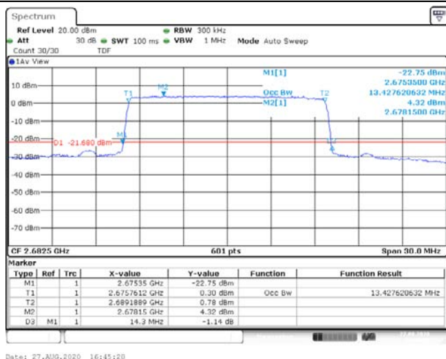
Band41-15MHz-16QAM-41515-75RB#0-13.428-14.300-PASS
