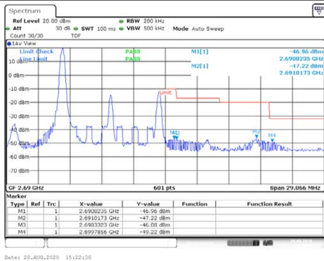
Band41-10MHz-16QAM-41540-1RB#0--46.96,-47.22,-46.08,-49.22-PASS
