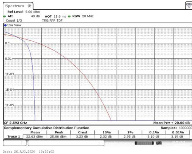
Band41-15MHz-QPSK-40620-75RB#0-3.10-13-PASS
