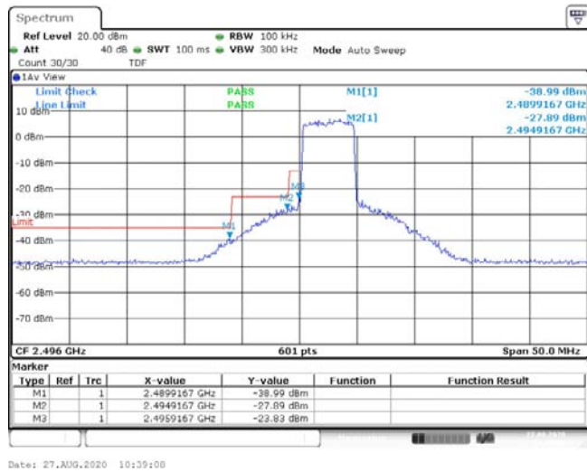
Band41-5MHz-16QAM-39675-25RB#0--38.99,-27.89,-23.83-PASS
