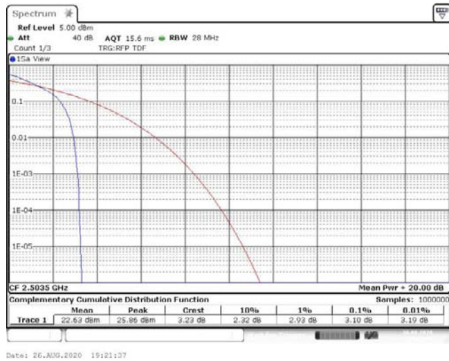
Band41-15MHz-16QAM-39725-1RB#0-3.10-13-PASS
