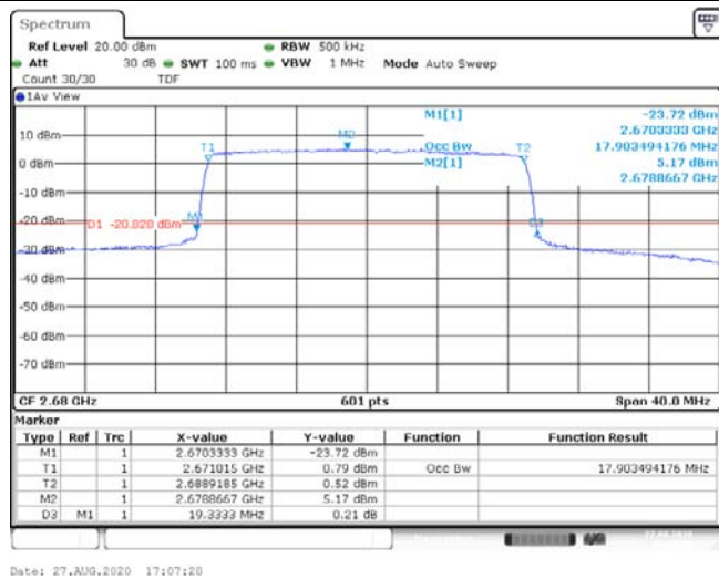
Band41-20MHz-16QAM-41490-100RB#0-17.903-19.333-PASS
