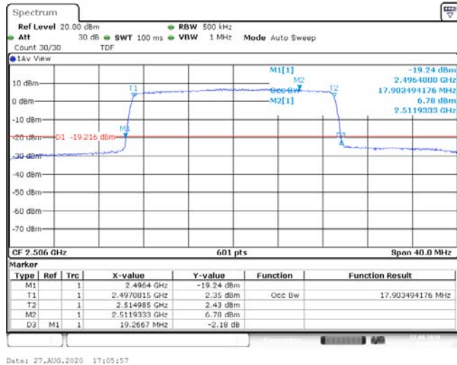
Band41-20MHz-16QAM-39750-100RB#0-17.903-19.267-PASS
