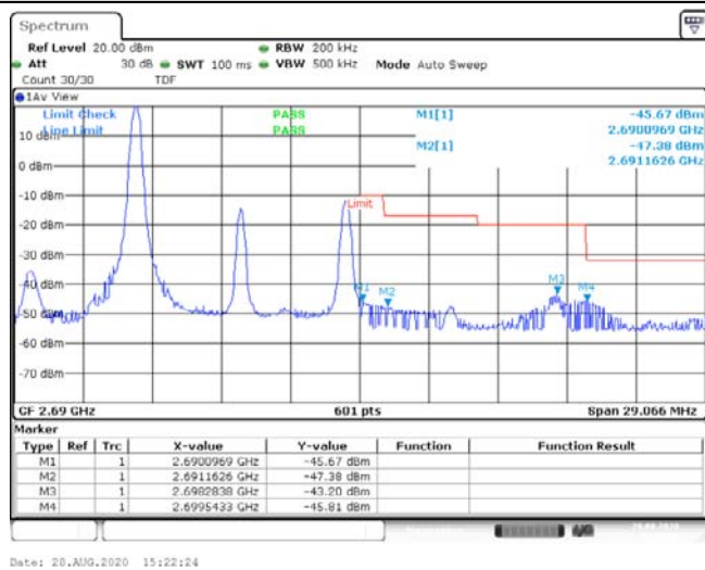
Band41-10MHz-QPSK-41540-1RB#0--45.67,-47.38,-43.20,-45.81-PASS
