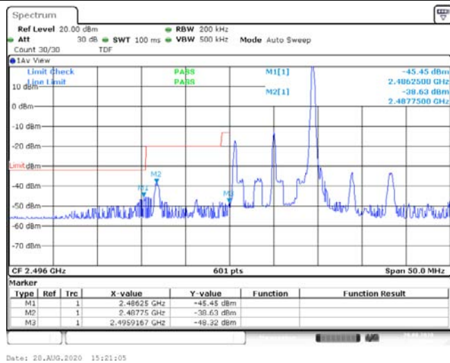
Band41-10MHz-QPSK-39700-1RB#49--45.45,-38.63,-48.32-PASS
