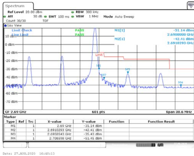
Band41-15MHz-QPSK-41515-1RB#74--31.14,-42.41,-35.43,-51.45-PASS
