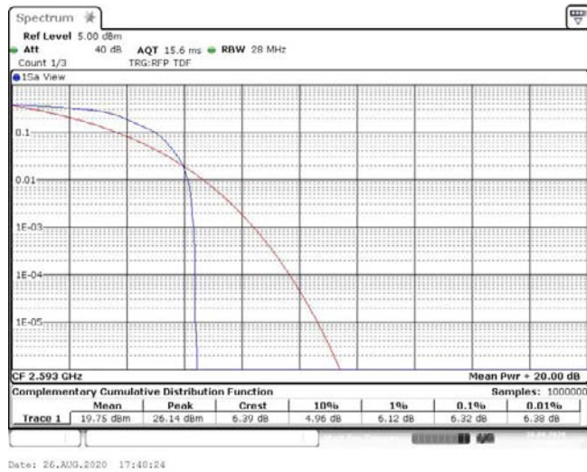
Band41-5MHz-16QAM-40620-25RB#0-6.32-13-PASS
