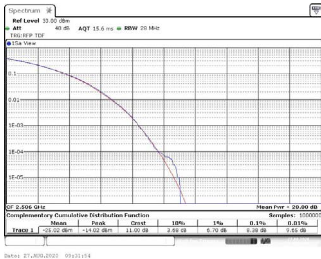
Band41-20MHz-16QAM-39750-100RB#0-8.38-13-PASS
