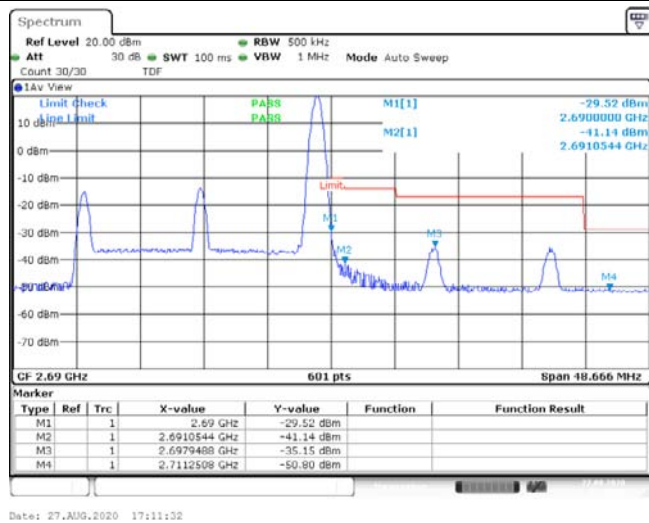
Band41-20MHz-16QAM-41490-1RB#99--29.52,-41.14,-35.15,-50.80-PASS
