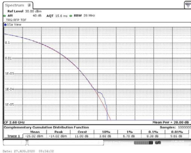
Band41-20MHz-QPSK-41490-100RB#0-8.38-13-PASS
