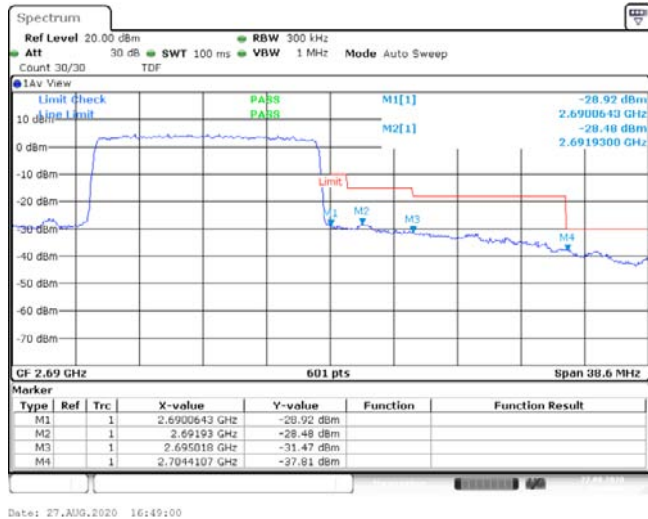
Band41-15MHz-16QAM-41515-75RB#0--28.92,-28.48,-31.47,-37.81-PASS
