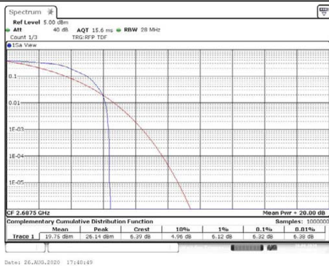
Band41-5MHz-16QAM-41565-1RB#0-6.32-13-PASS
