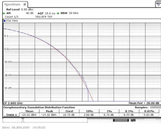
Band41-10MHz-16QAM-41540-50RB#0-8.49-13-PASS
