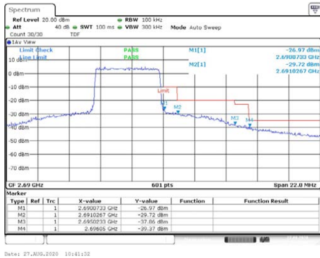
Band41-5MHz-16QAM-41565-25RB#0--26.97,-29.72,-37.86,-39.37-PASS
