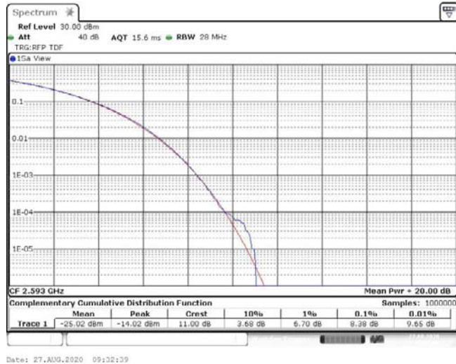
Band41-20MHz-16QAM-40620-1RB#0-8.38-13-PASS
