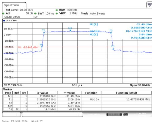
Band41-15MHz-16QAM-40620-75RB#0-13.478-14.300-PASS
