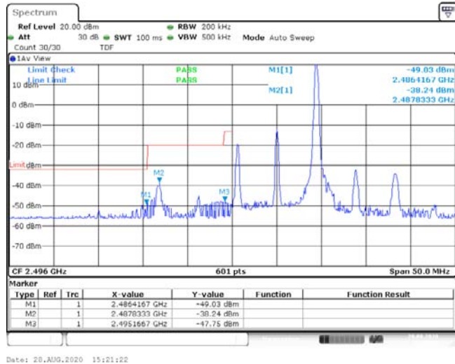
Band41-10MHz-16QAM-39700-1RB#49--49.03,-38.24,-47.75-PASS
