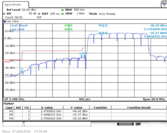
Band41-20MHz-QPSK-39750-100RB#0--46.45,-25.37,-25.18-PASS
