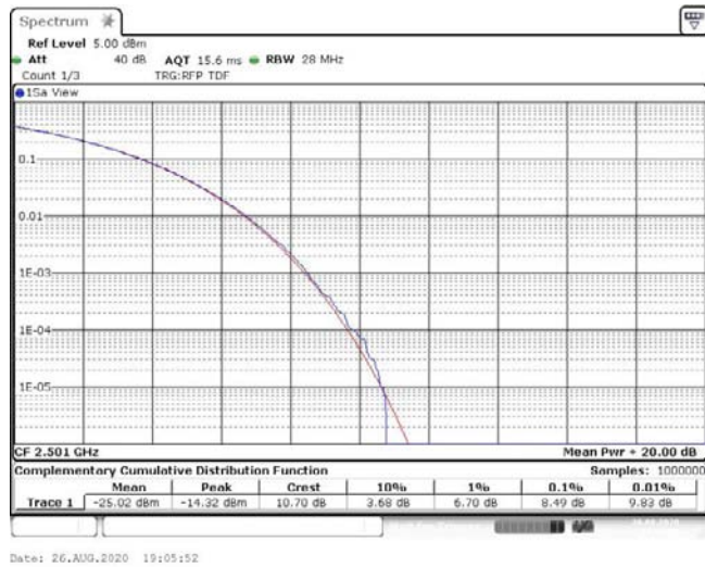
Band41-10MHz-16QAM-39700-1RB#0-8.49-13-PASS
