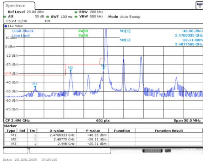
Band41-10MHz-QPSK-39700-1RB#0--46.36,-28.11,-25.71-PASS
