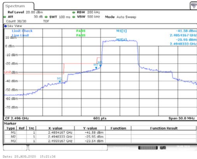
Band41-10MHz-QPSK-39700-50RB#0--41.58,-25.95,-23.54-PASS
