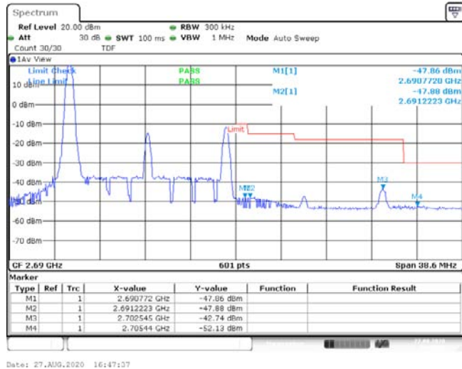
Band41-15MHz-QPSK-41515-1RB#0--47.86,-47.88,-42.74,-52.13-PASS
