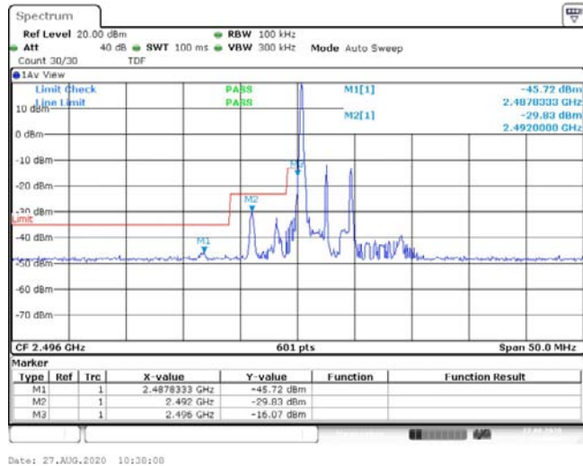
Band41-5MHz-16QAM-39675-1RB#0--45.72,-29.83,-16.07-PASS
