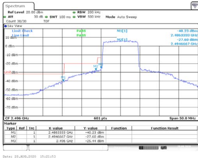
Band41-10MHz-16QAM-39700-50RB#0--40.23,-27.60,-25.44-PASS
