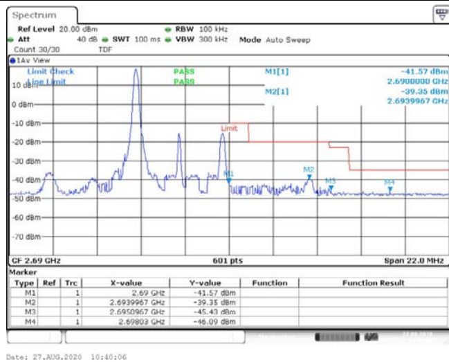
Band41-5MHz-16QAM-41565-1RB#0--41.57,-39.35,-45.43,-46.09-PASS
