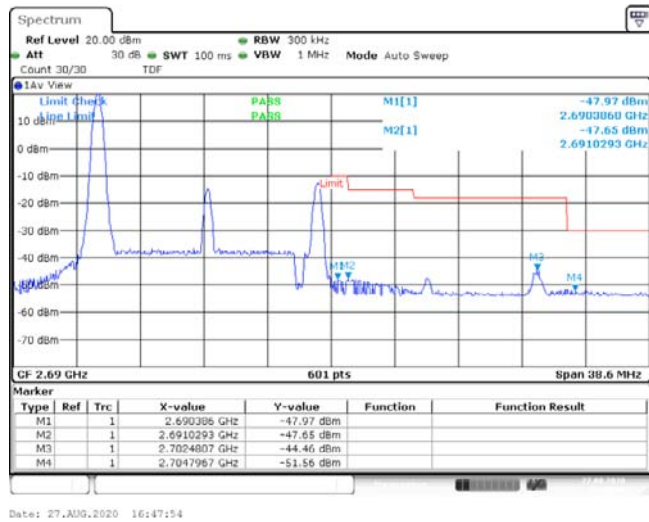
Band41-15MHz-16QAM-41515-1RB#0--47.97,-47.65,-44.46,-51.56-PASS
