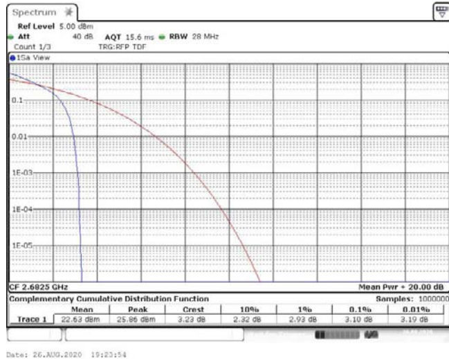
Band41-15MHz-QPSK-41515-75RB#0-3.10-13-PASS
