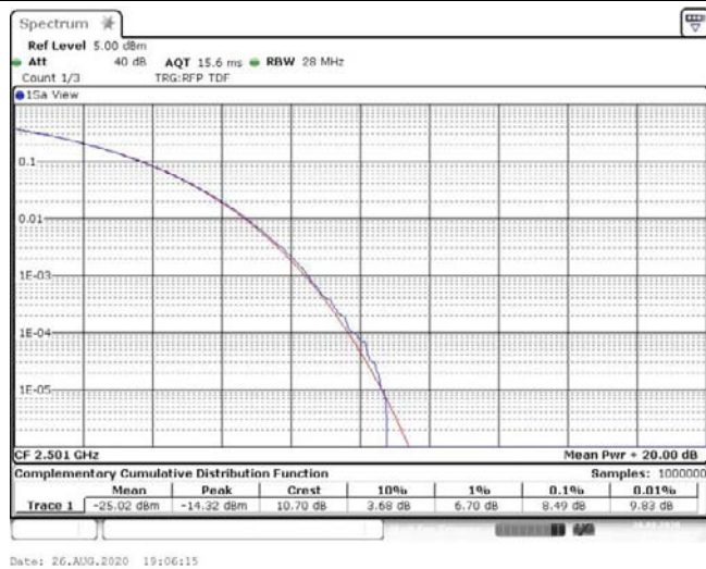
Band41-10MHz-16QAM-39700-50RB#0-8.49-13-PASS
