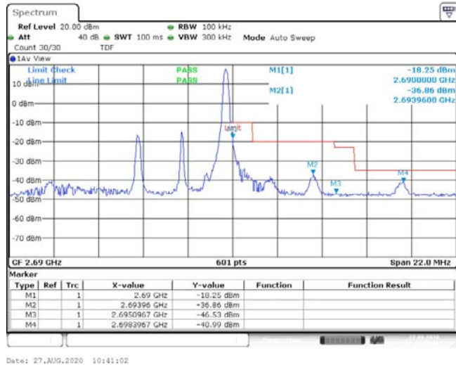
Band41-5MHz-16QAM-41565-1RB#24--18.25,-36.86,-46.53,-40.99-PASS
