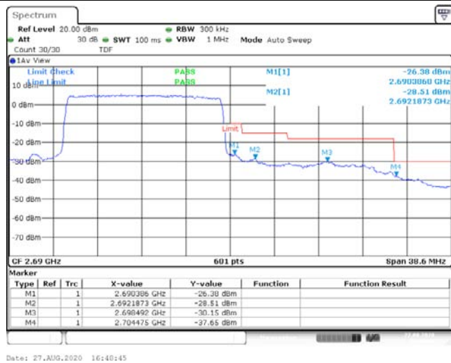
Band41-15MHz-QPSK-41515-75RB#0--26.38,-28.51,-30.15,-37.65-PASS
