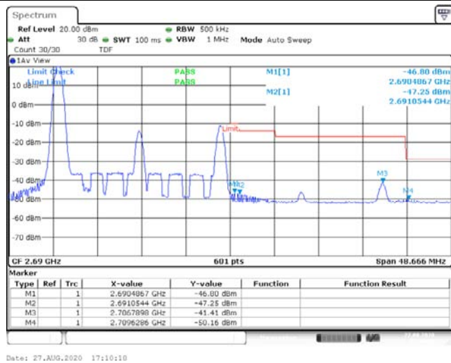
Band41-20MHz-QPSK-41490-1RB#0--46.80,-47.25,-41.41,-50.16-PASS
