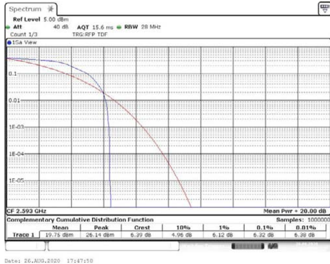
Band41-5MHz-16QAM-40620-1RB#0-6.32-13-PASS
