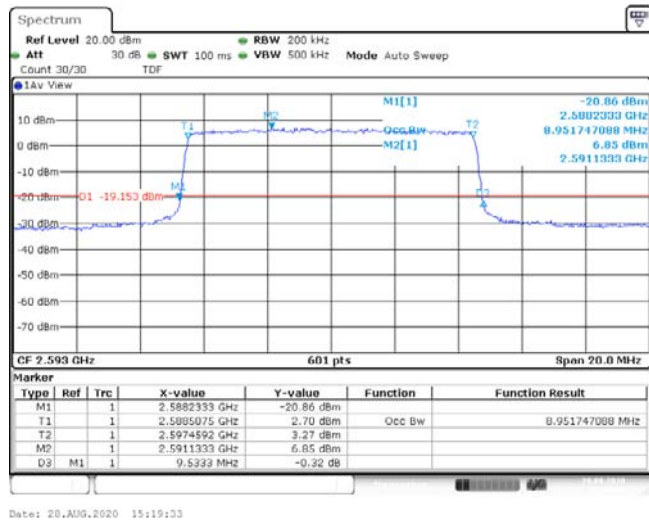
Band41-10MHz-QPSK-40620-50RB#0-8.952-9.533-PASS
